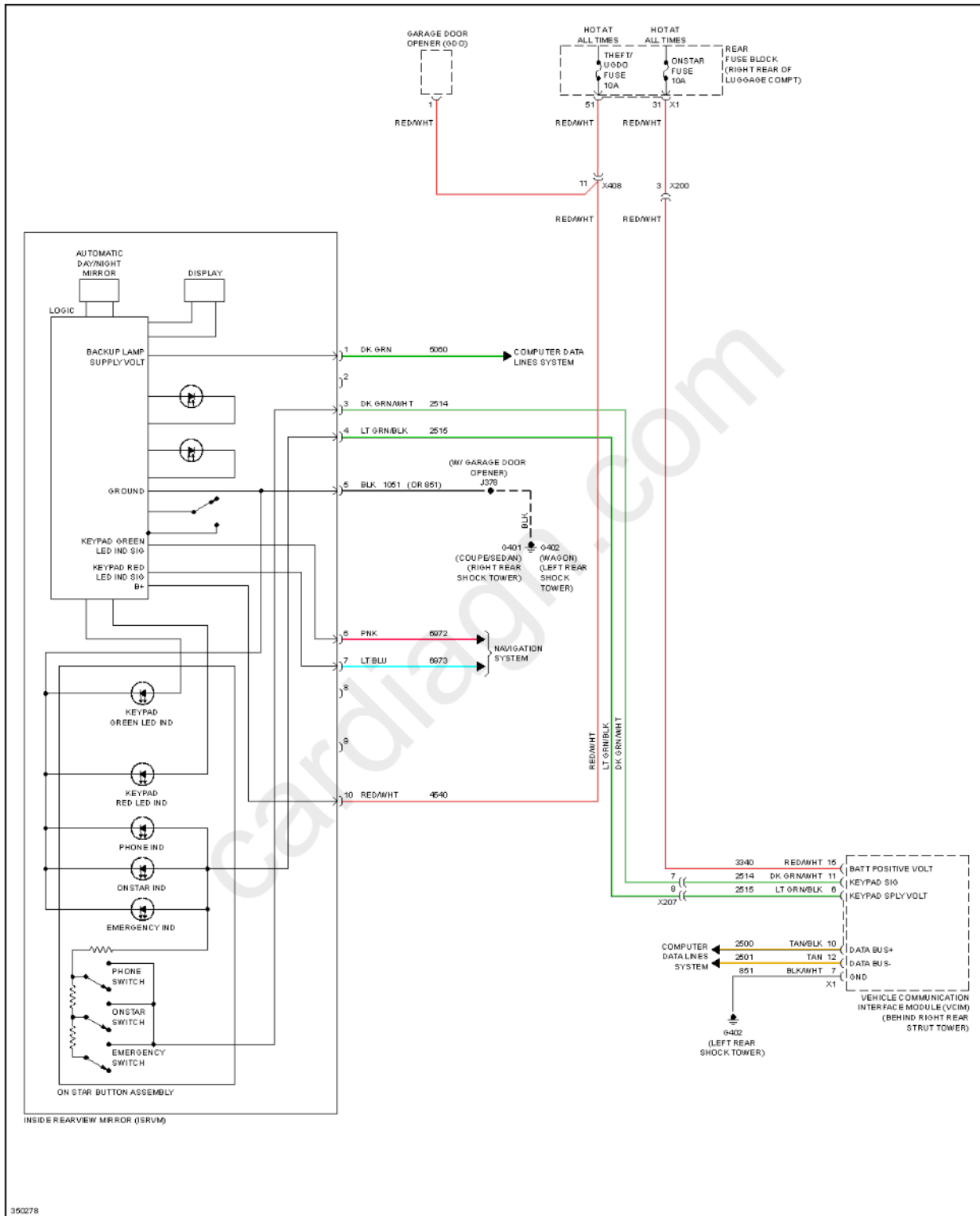
Fig. 84: Automatic Day/Night Mirror Circuit, W/ Infotainment System 1/2/3 & Rearview Camera
