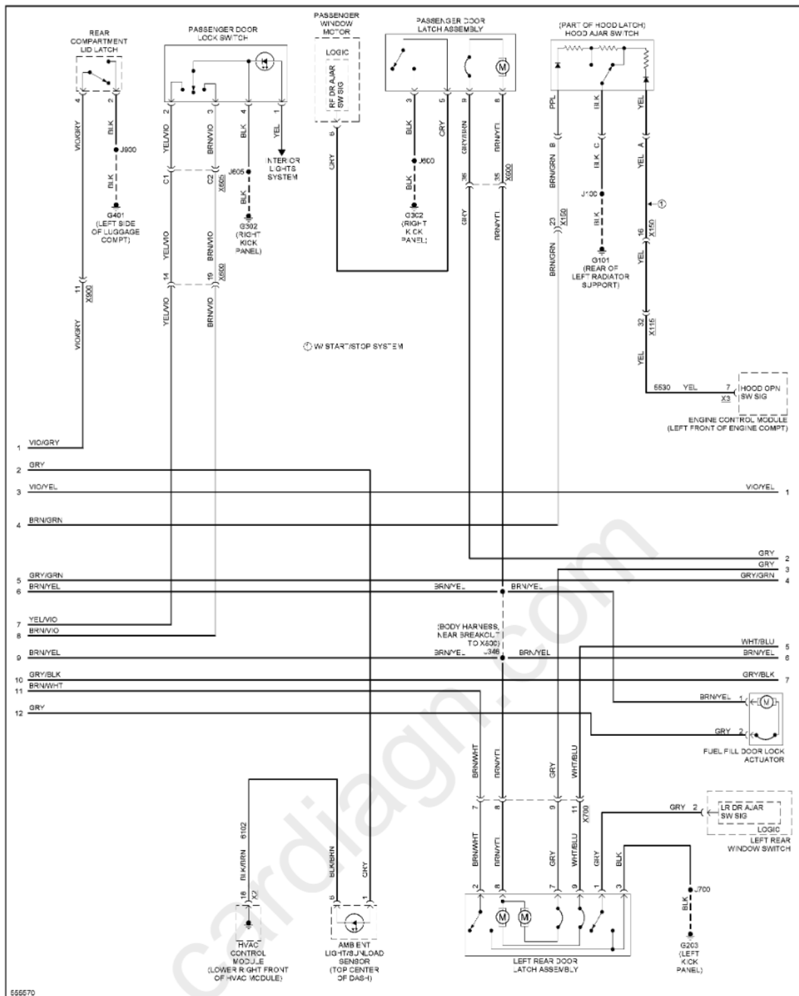
Fig. 96: Power Door Locks Circuit, W/O Passive Keyless Entry (2 of 3)
