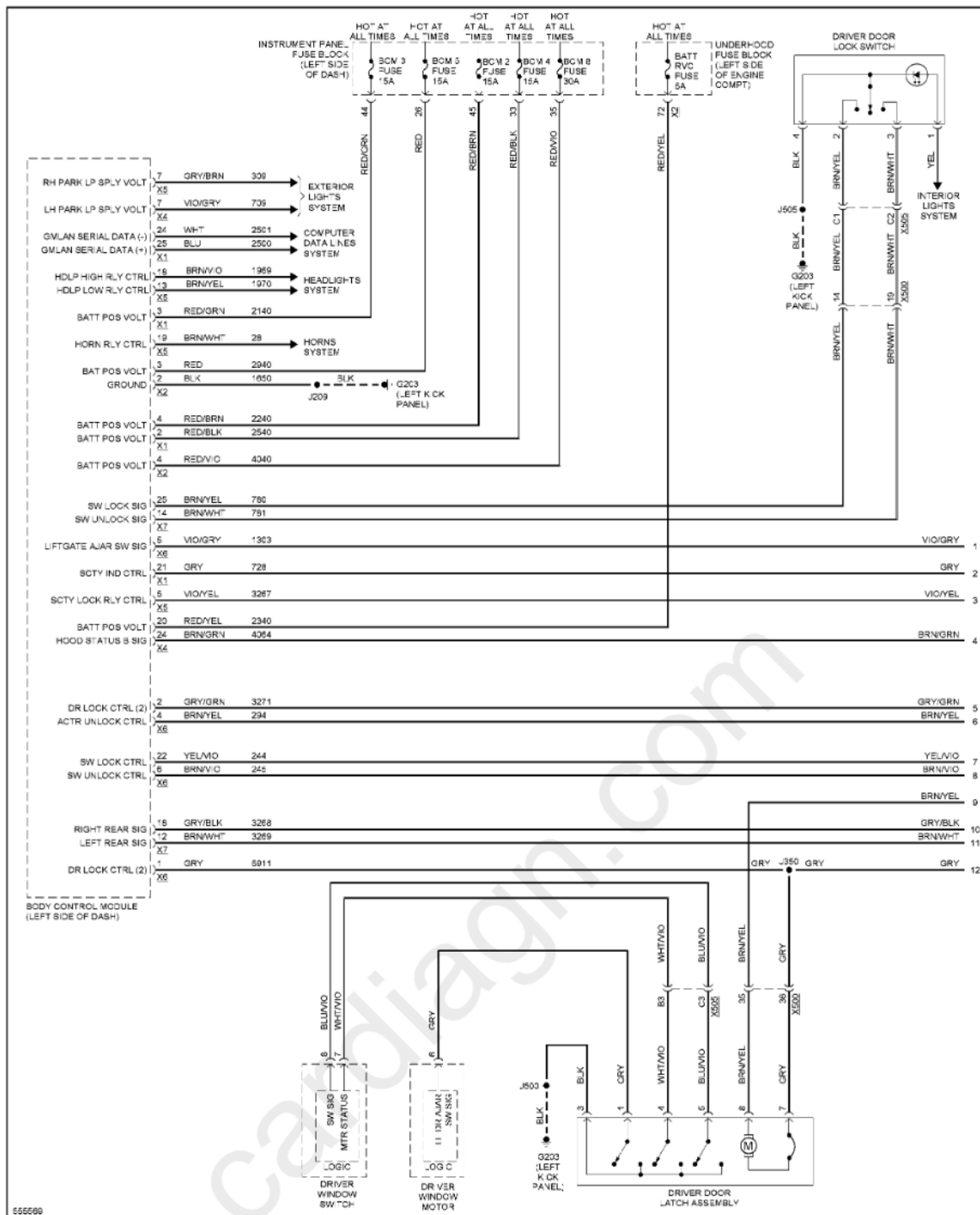
Fig. 95: Power Door Locks Circuit, W/O Passive Keyless Entry (1 of 3)
