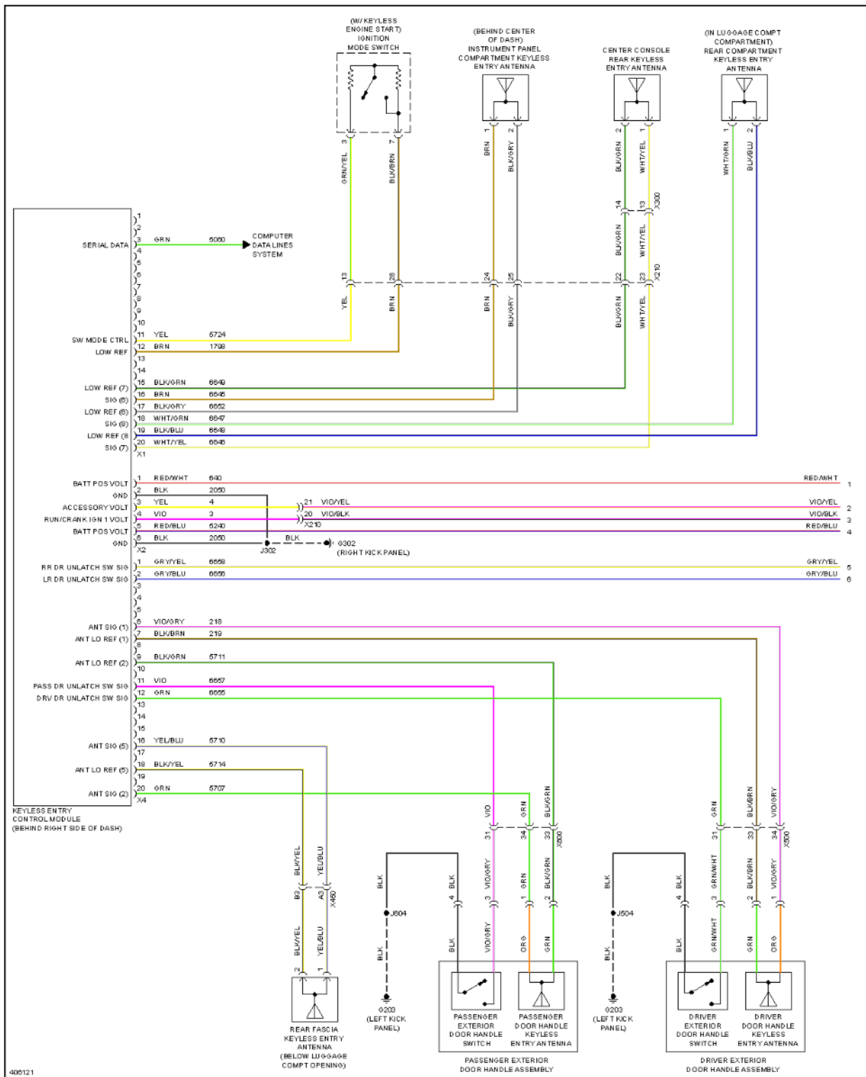
Fig. 94: Power Door Locks Circuit, W/ Passive Keyless Entry (1 of 4)
