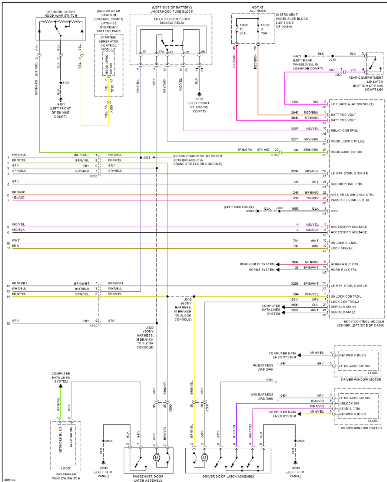
Fig. 97: Power Door Locks Circuit, W/ Passive Keyless Entry (4 of 4)
