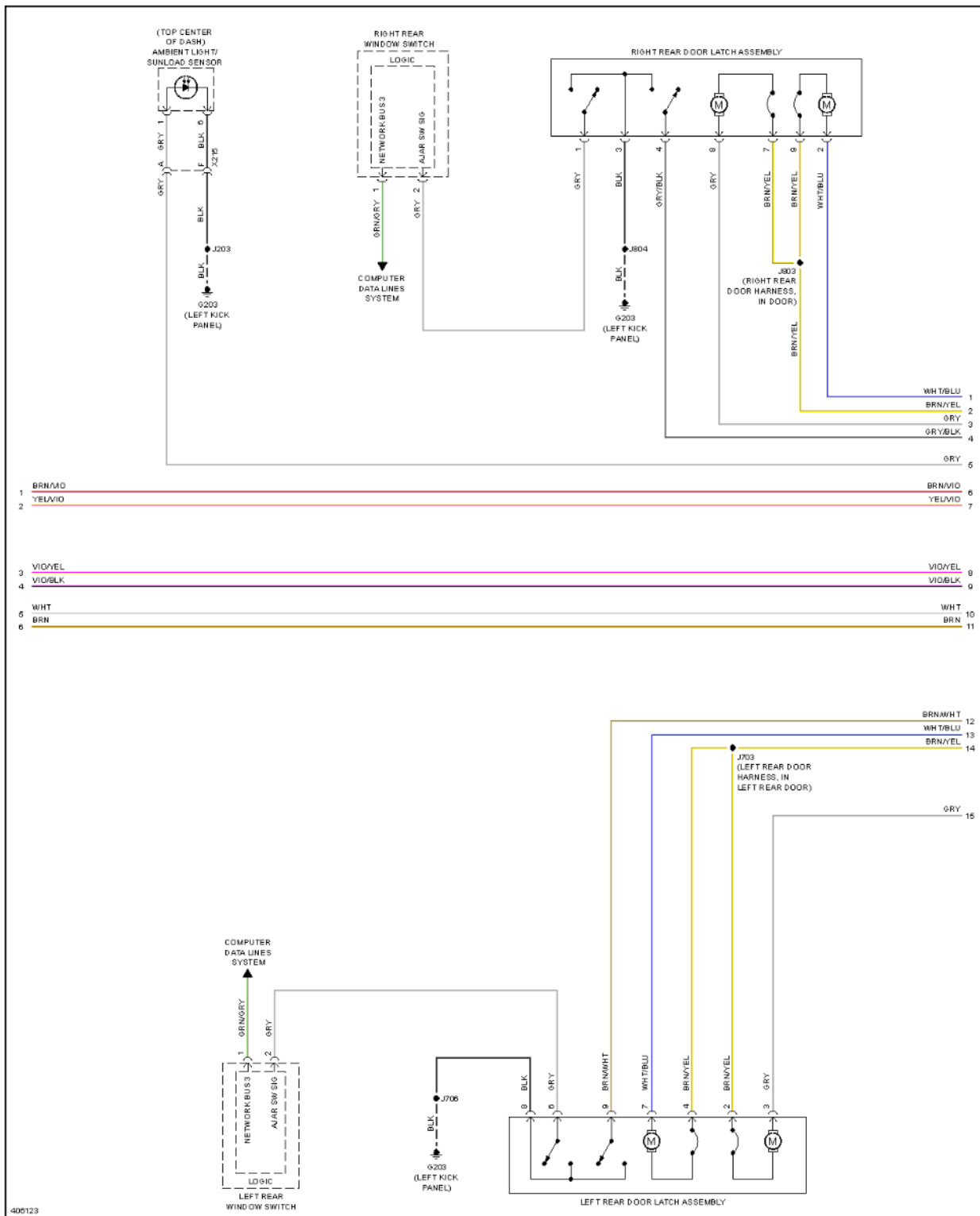
Fig. 96: Power Door Locks Circuit, W/ Passive Keyless Entry (3 of 4)
