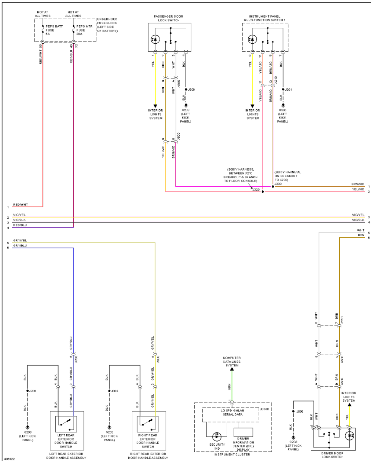
Fig. 95: Power Door Locks Circuit, W/ Passive Keyless Entry (2 of 4)
