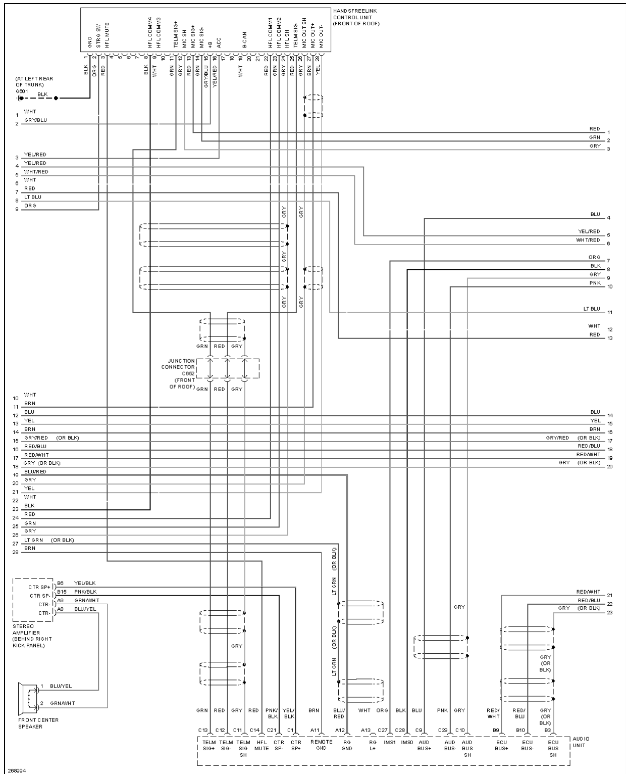
Fig. 62: Navigation Circuit, Canada (2 of 3)
