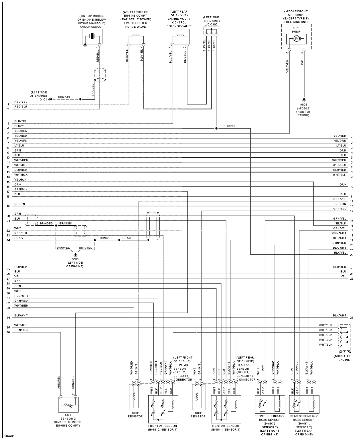
Fig. 34: 3.5L, Engine Performance Circuit, M/T (3 of 5)
