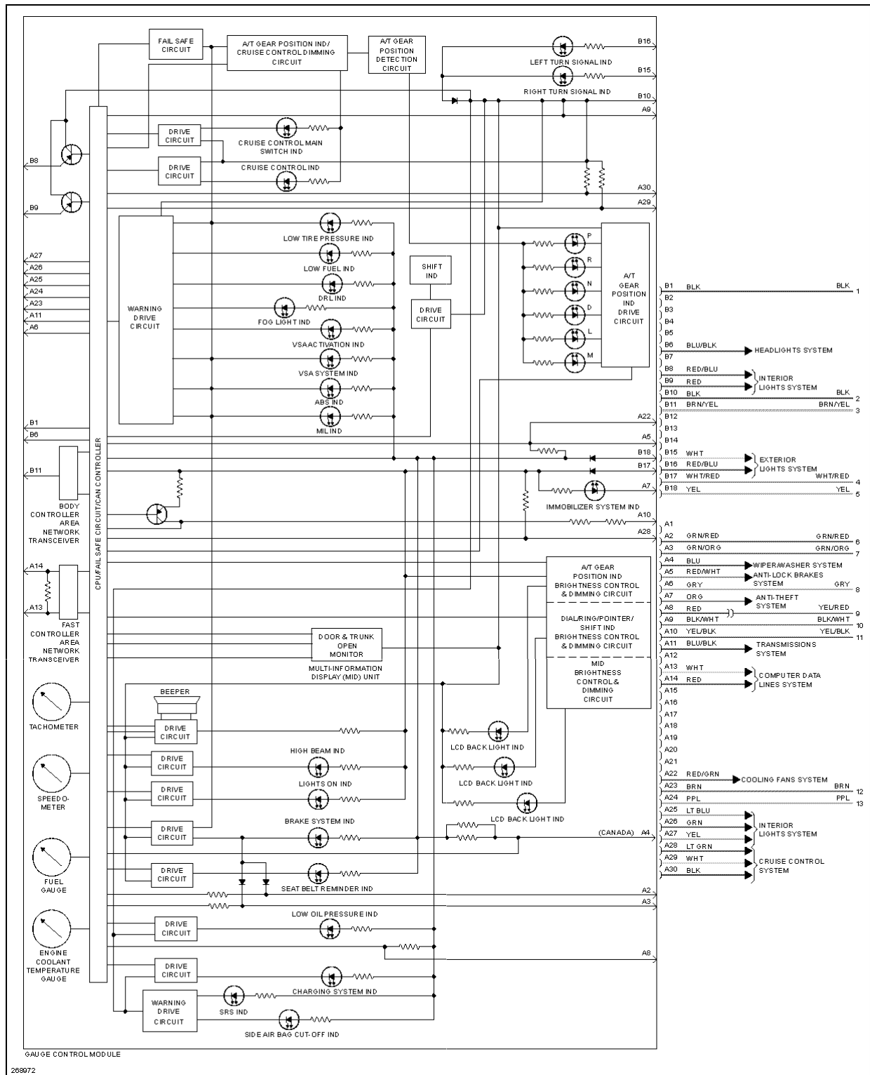
Fig. 50: Instrument Cluster Circuit (1 of 2)
