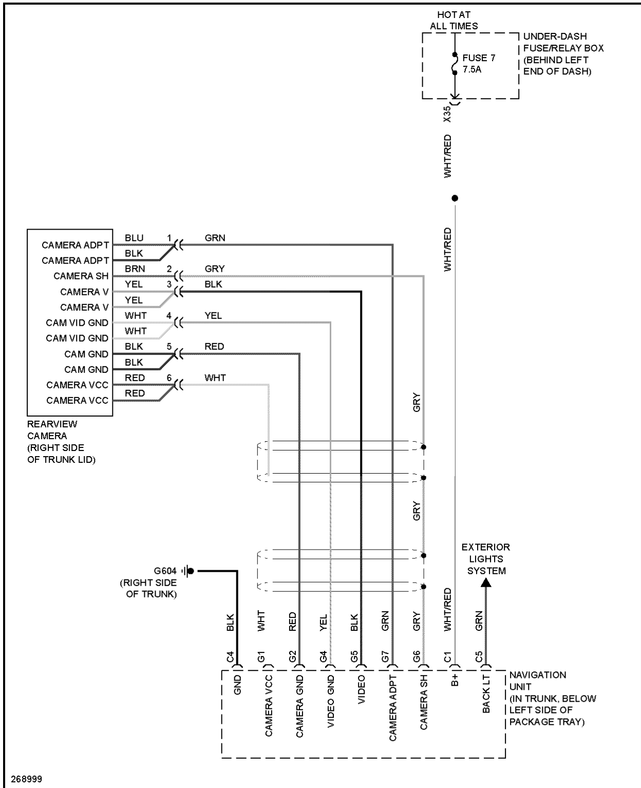
Fig. 68: Rear Camera Circuit
