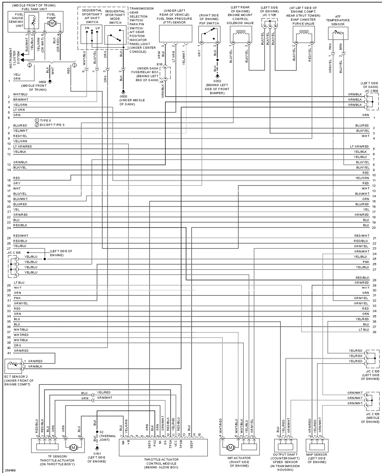
Fig. 28: 3.5L, Engine Performance Circuit, A/T (2 of 5)
