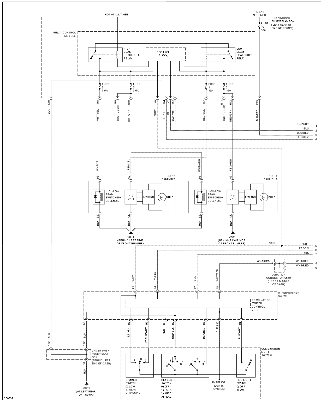
Fig. 45: Headlights Circuit, W/ DRL (1 of 2)
