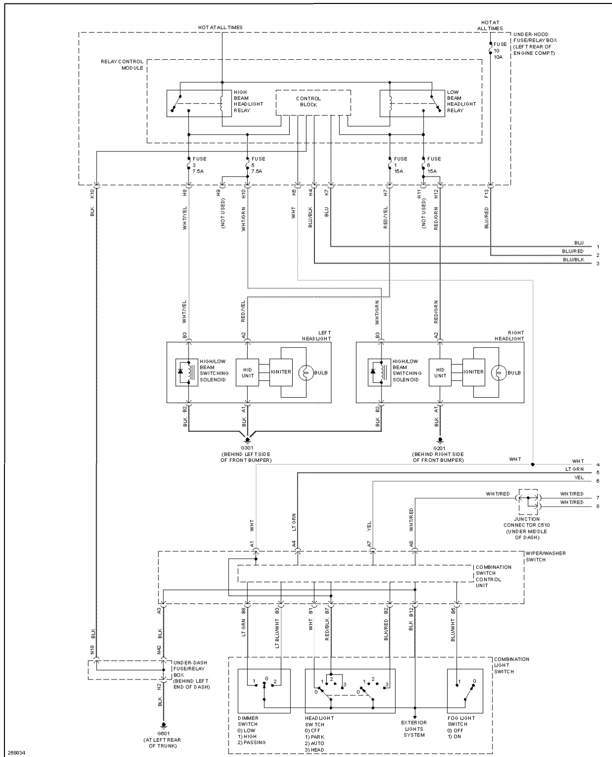
Fig. 47: Headlights Circuit, W/O DRL (1 of 2)
