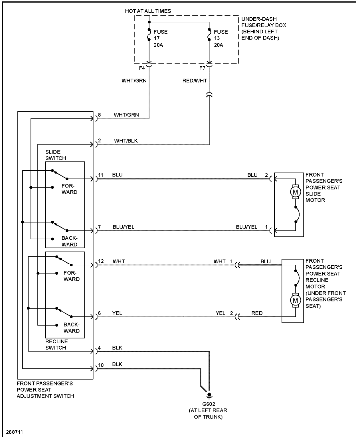
Fig. 81: Passenger Power Seat Circuit
