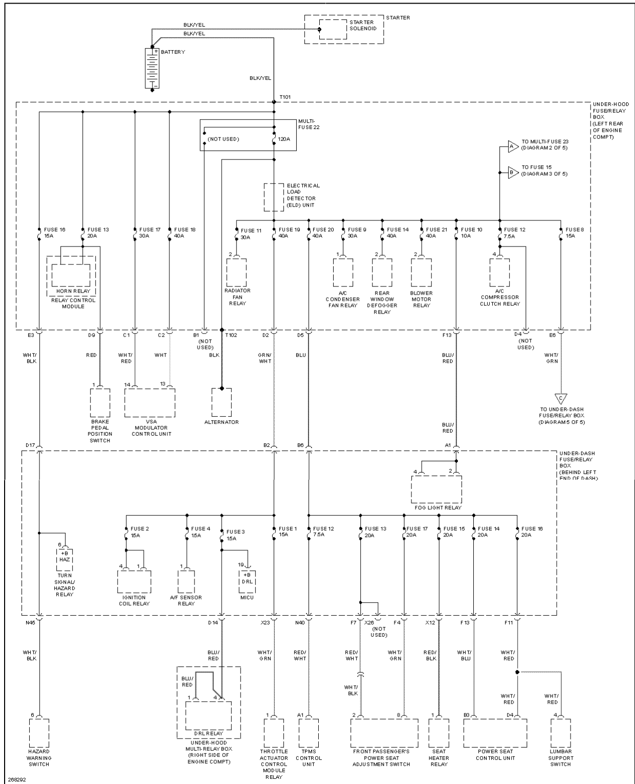
Fig. 70: Power Distribution Circuit (1 of 5)
