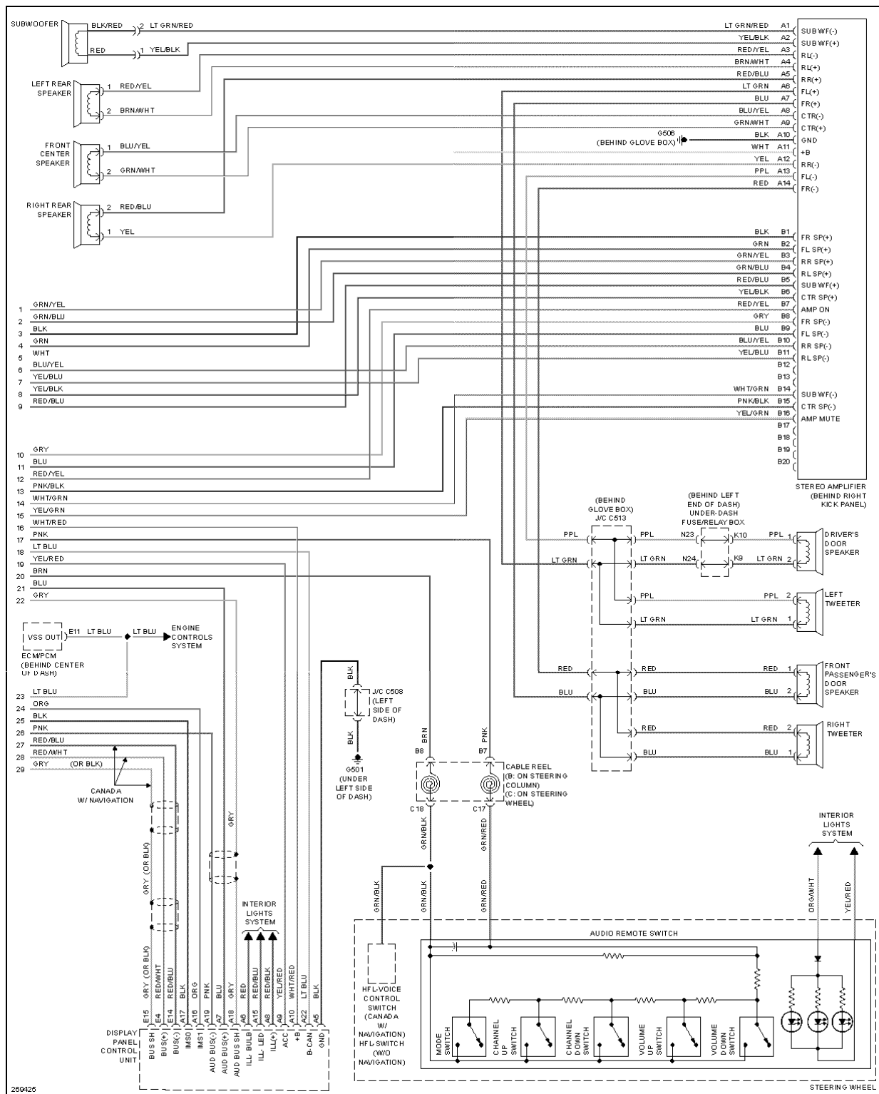
Fig. 91: Radio Circuit, W/O Navigation (3 of 3)
