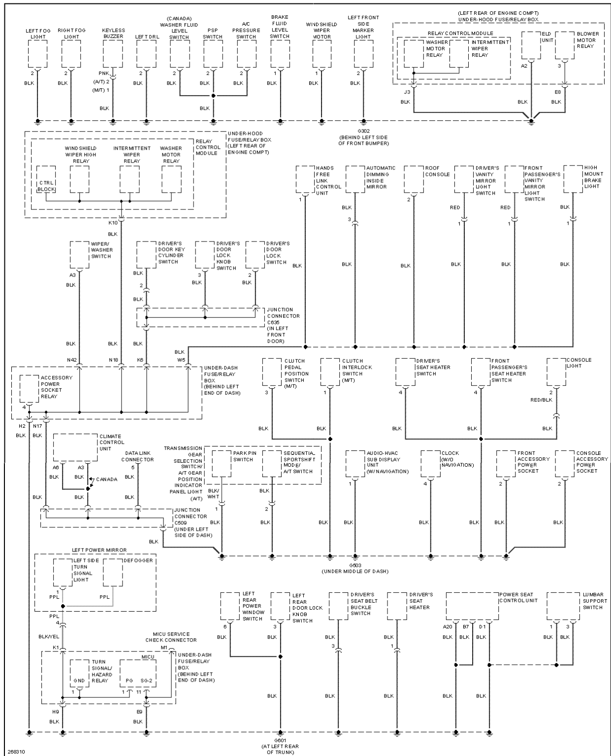
Fig. 42: Ground Distribution Circuit (2 of 4)
