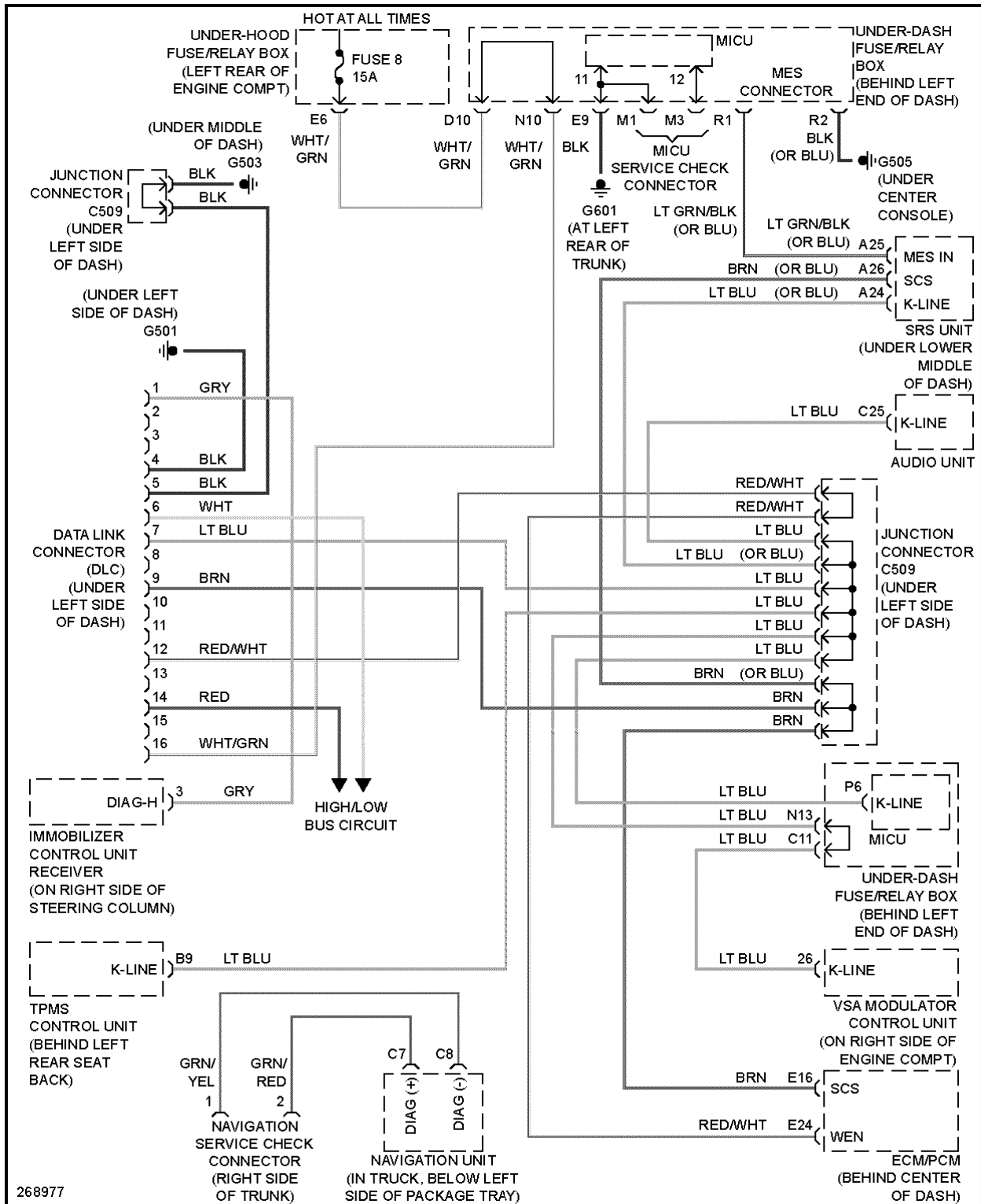
Fig. 11: Data Link Connector Circuit
