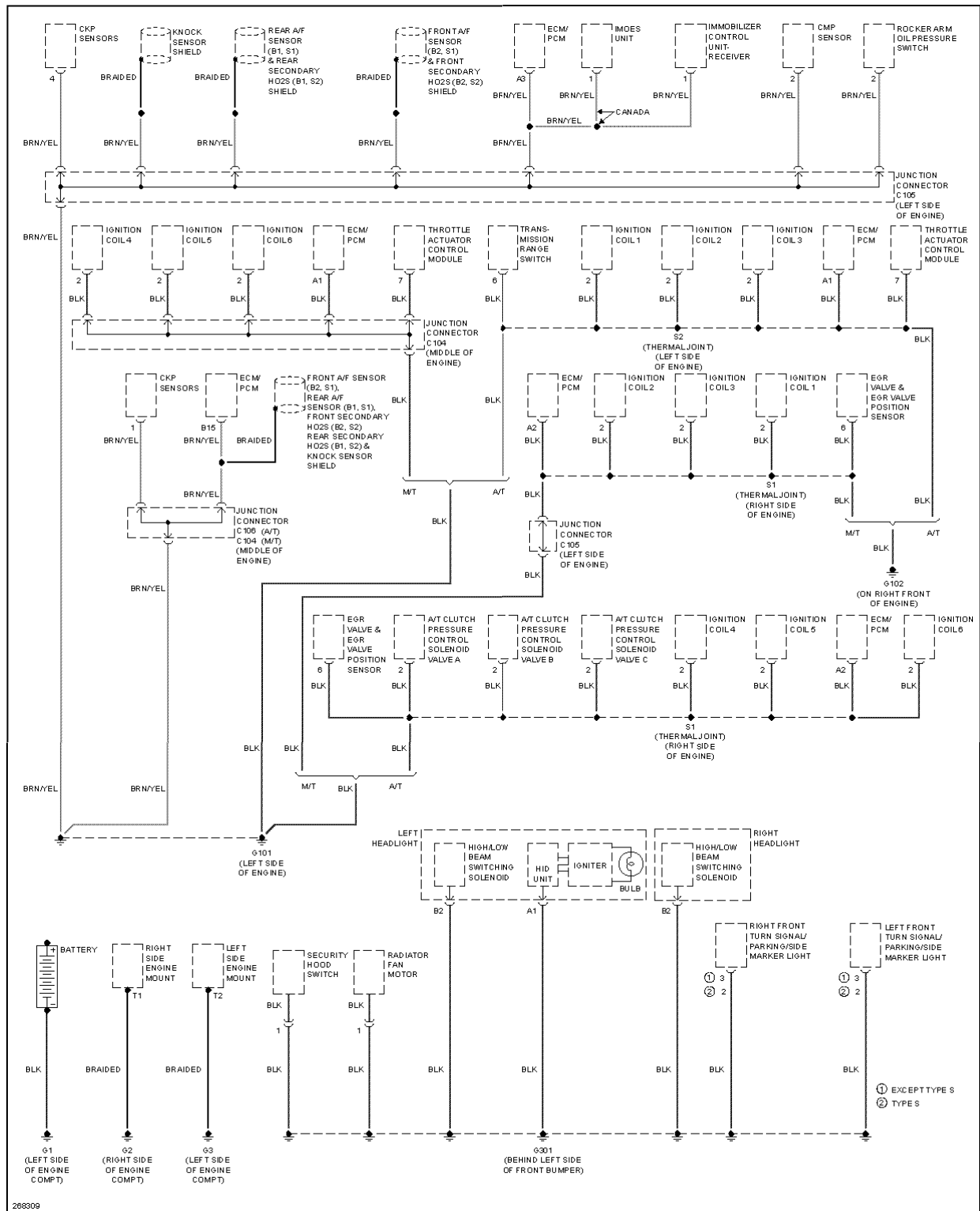
Fig. 41: Ground Distribution Circuit (1 of 4)
