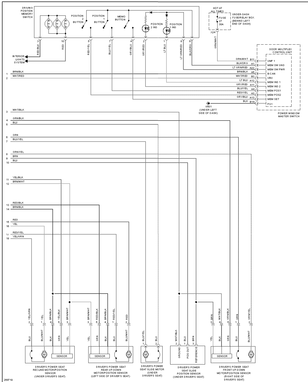
Fig. 58: Driver's Memory Seat Circuit (2 of 2)
