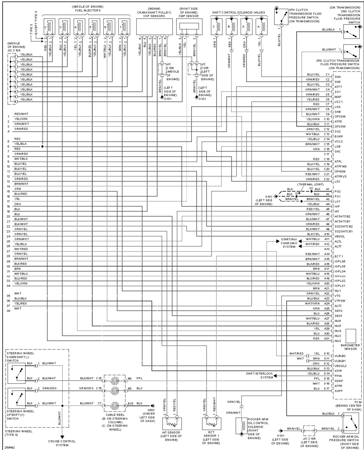
Fig. 21: 3.2L, Engine Performance Circuit, A/T (5 of 5)
