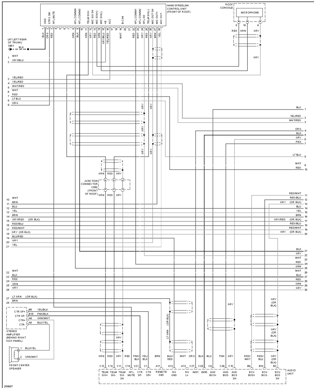
Fig. 65: Navigation Circuit, USA (2 of 3)
