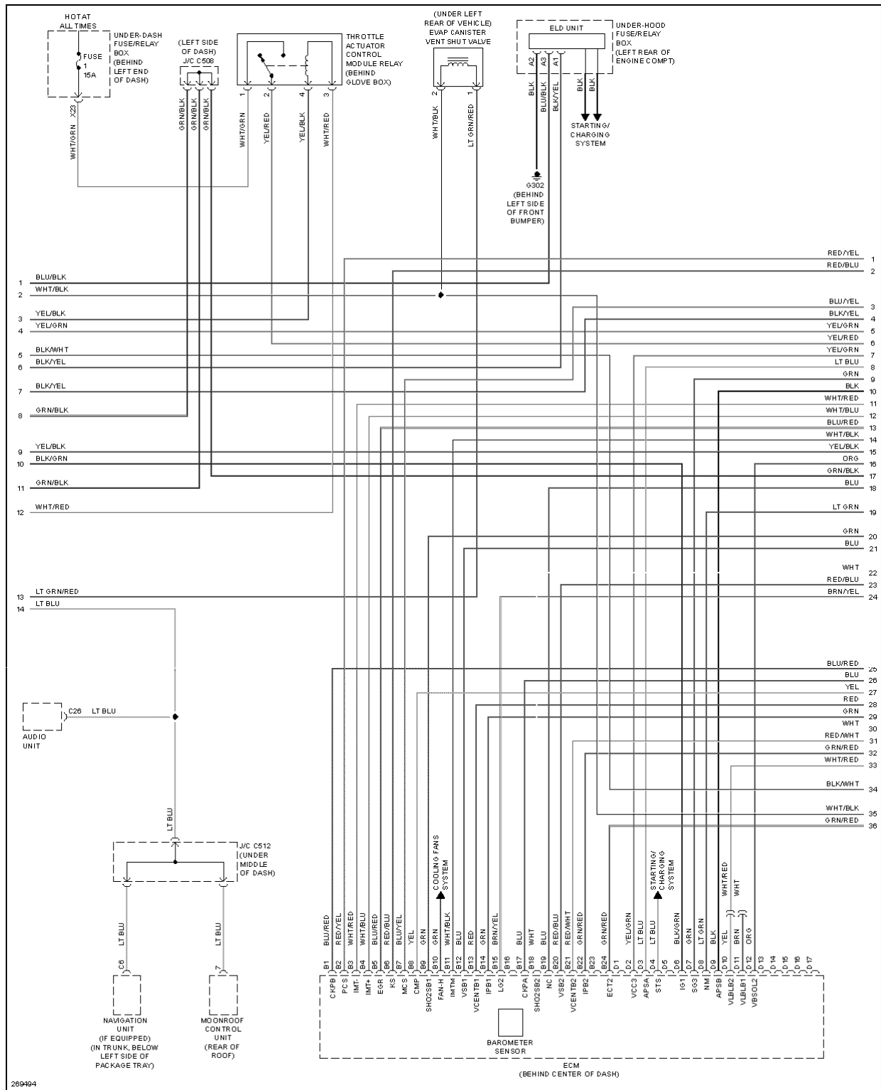
Fig. 23: 3.2L, Engine Performance Circuit, M/T (2 of 5)
