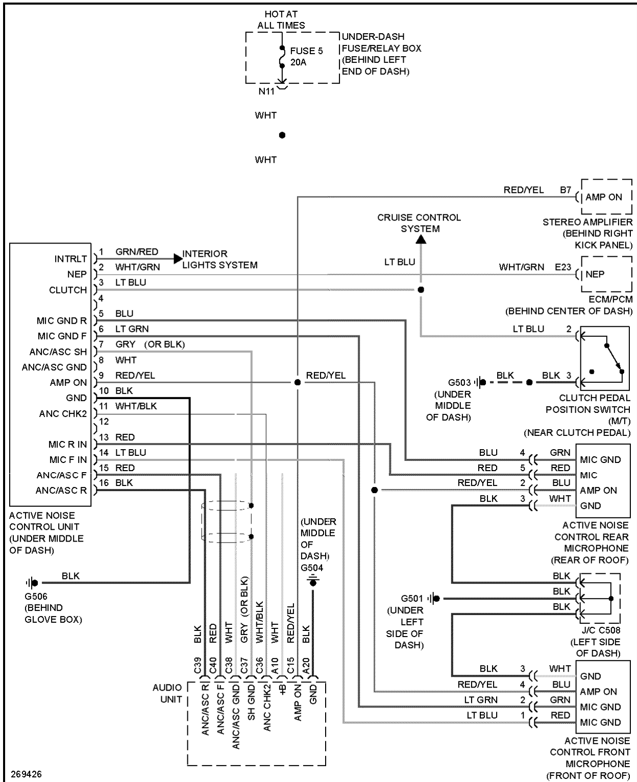
Fig. 85: Active Noise Control Circuit
