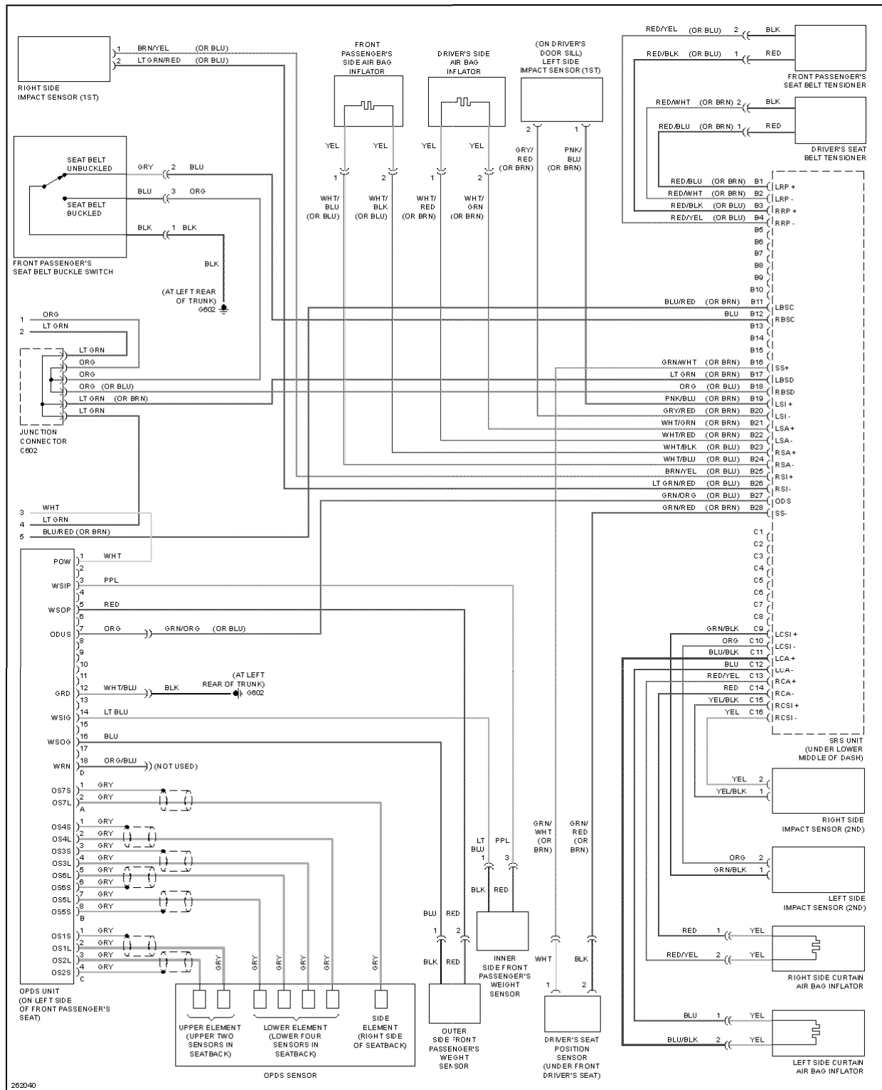
Fig. 98: Supplemental Restraints Circuit (2 of 2)
