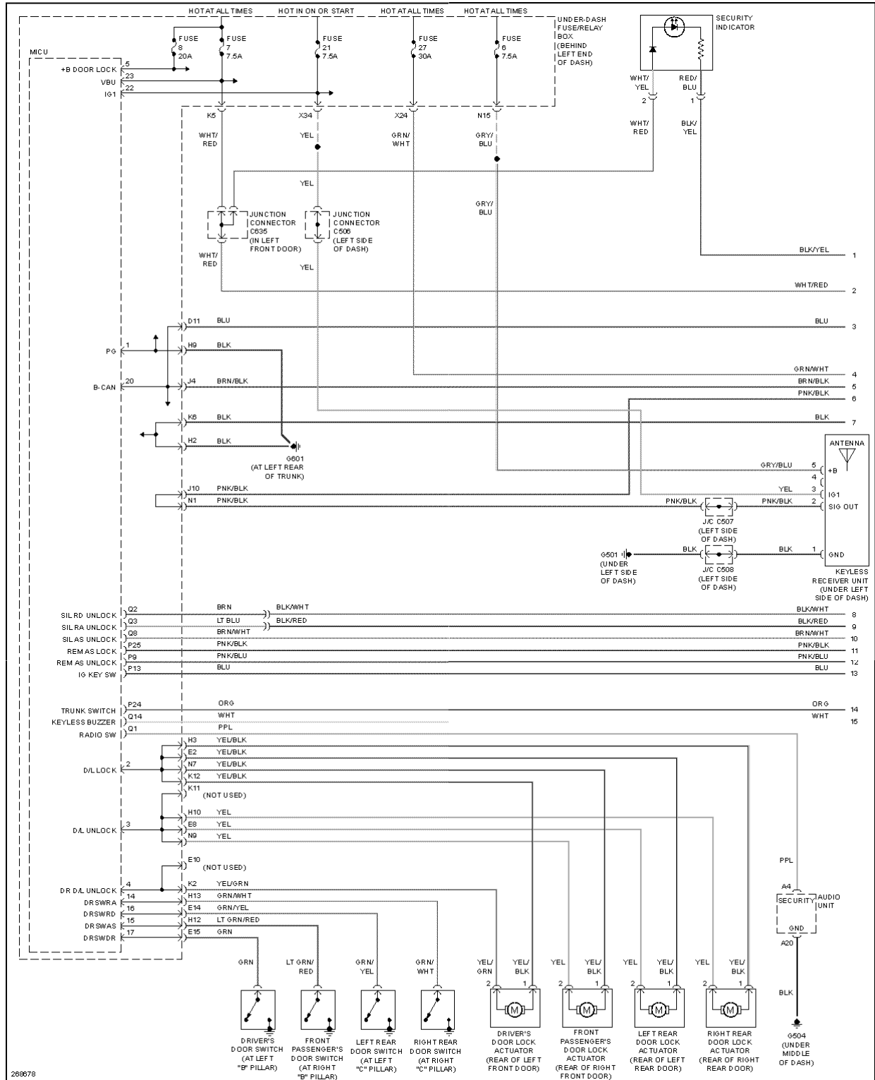
Fig. 75: Power Door Locks Circuit (1 of 2)
