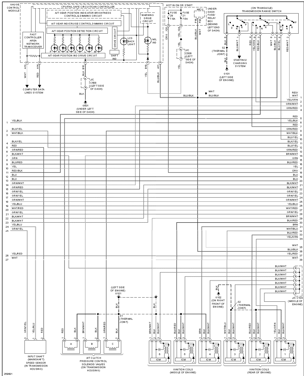
Fig. 20: 3.2L, Engine Performance Circuit, A/T (4 of 5)
