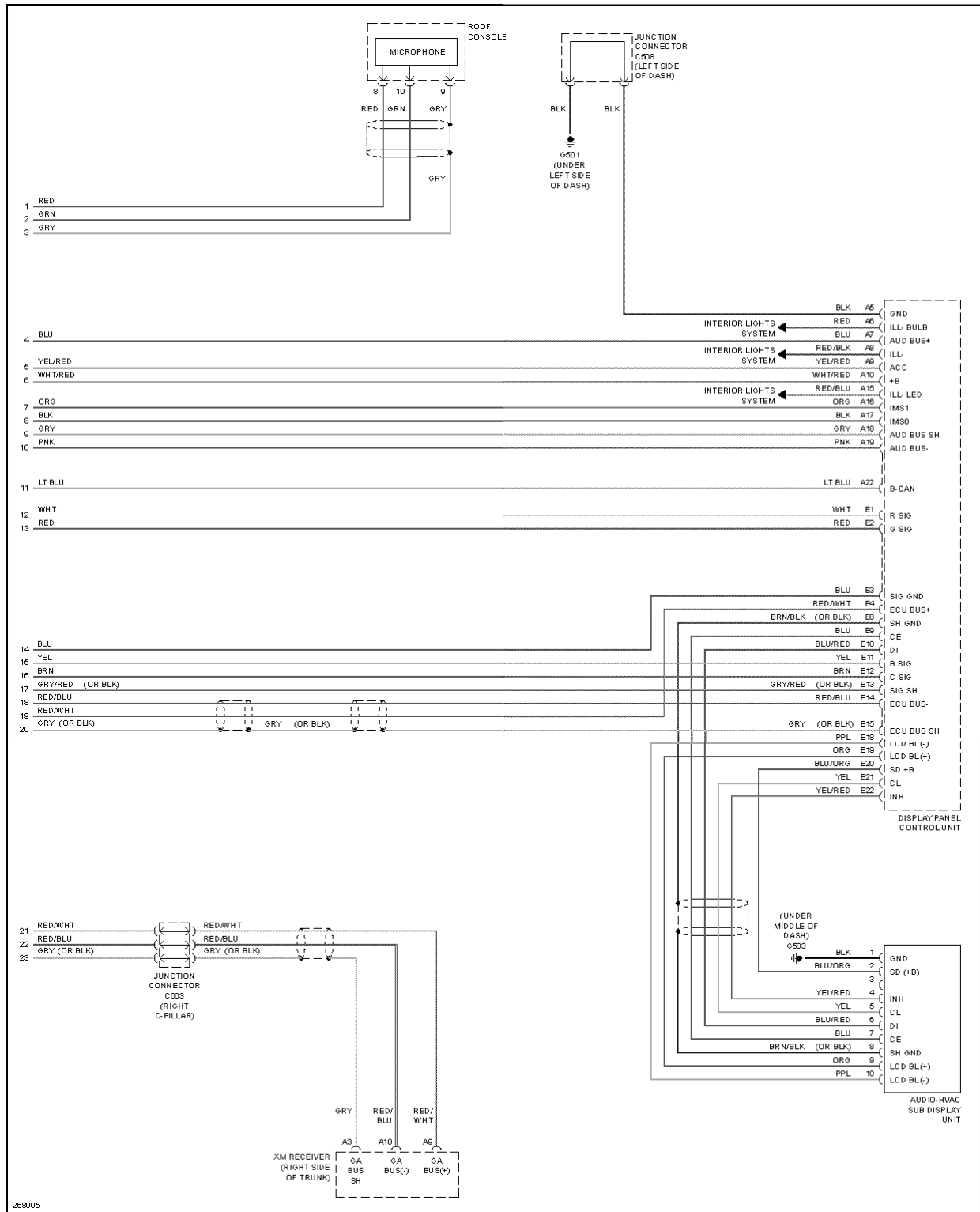
Fig. 63: Navigation Circuit, Canada (3 of 3)
