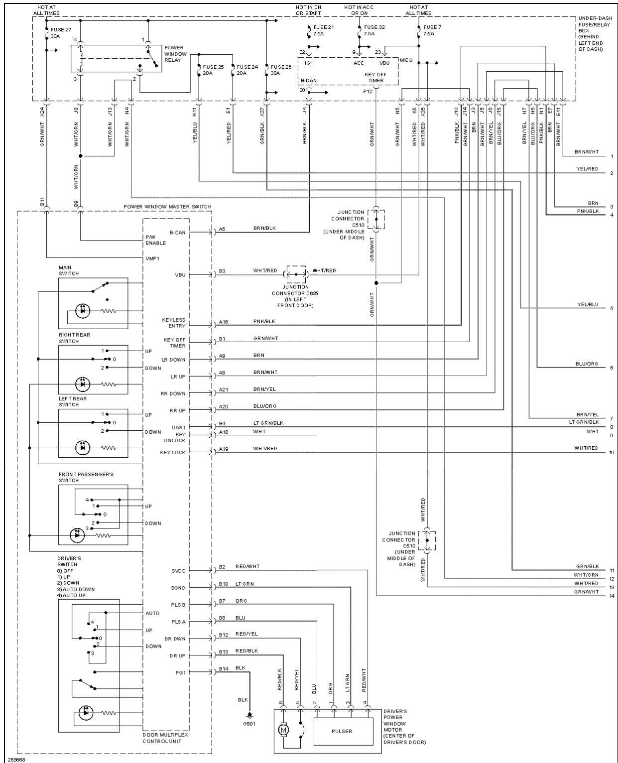
Fig. 83: Power Windows Circuit (1 of 2)
