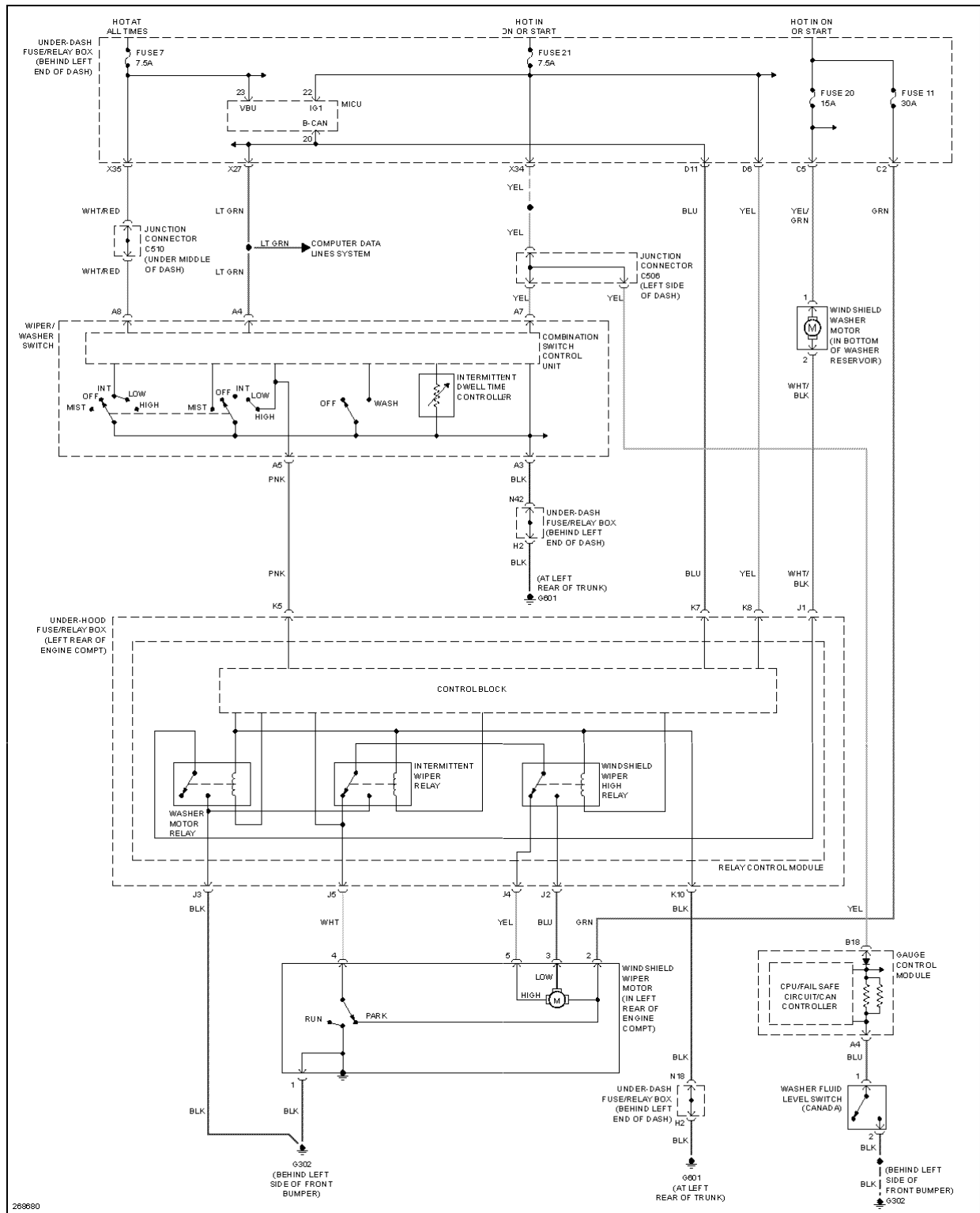
Fig. 104: Wiper/Washer Circuit
