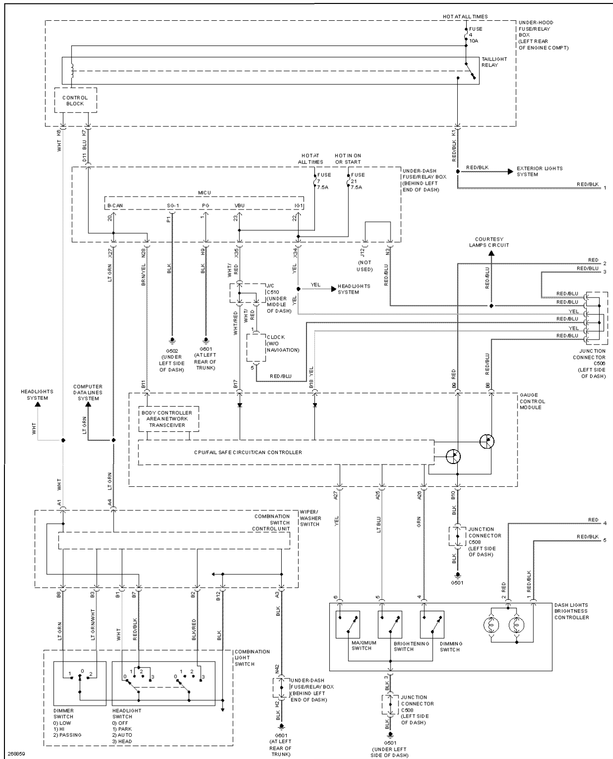
Fig. 54: Instrument Illumination Circuit (1 of 3)
