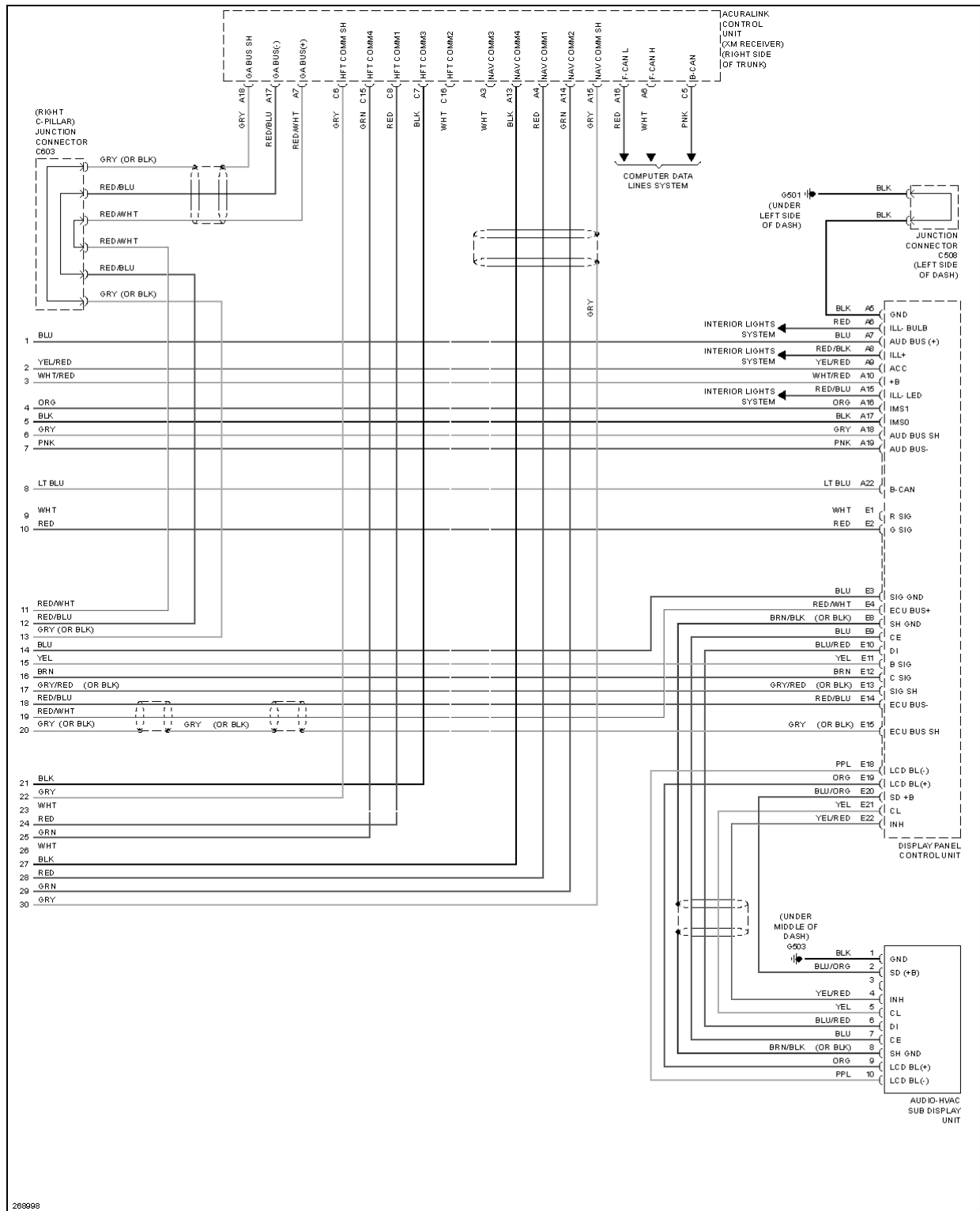
Fig. 66: Navigation Circuit, USA (3 of 3)
