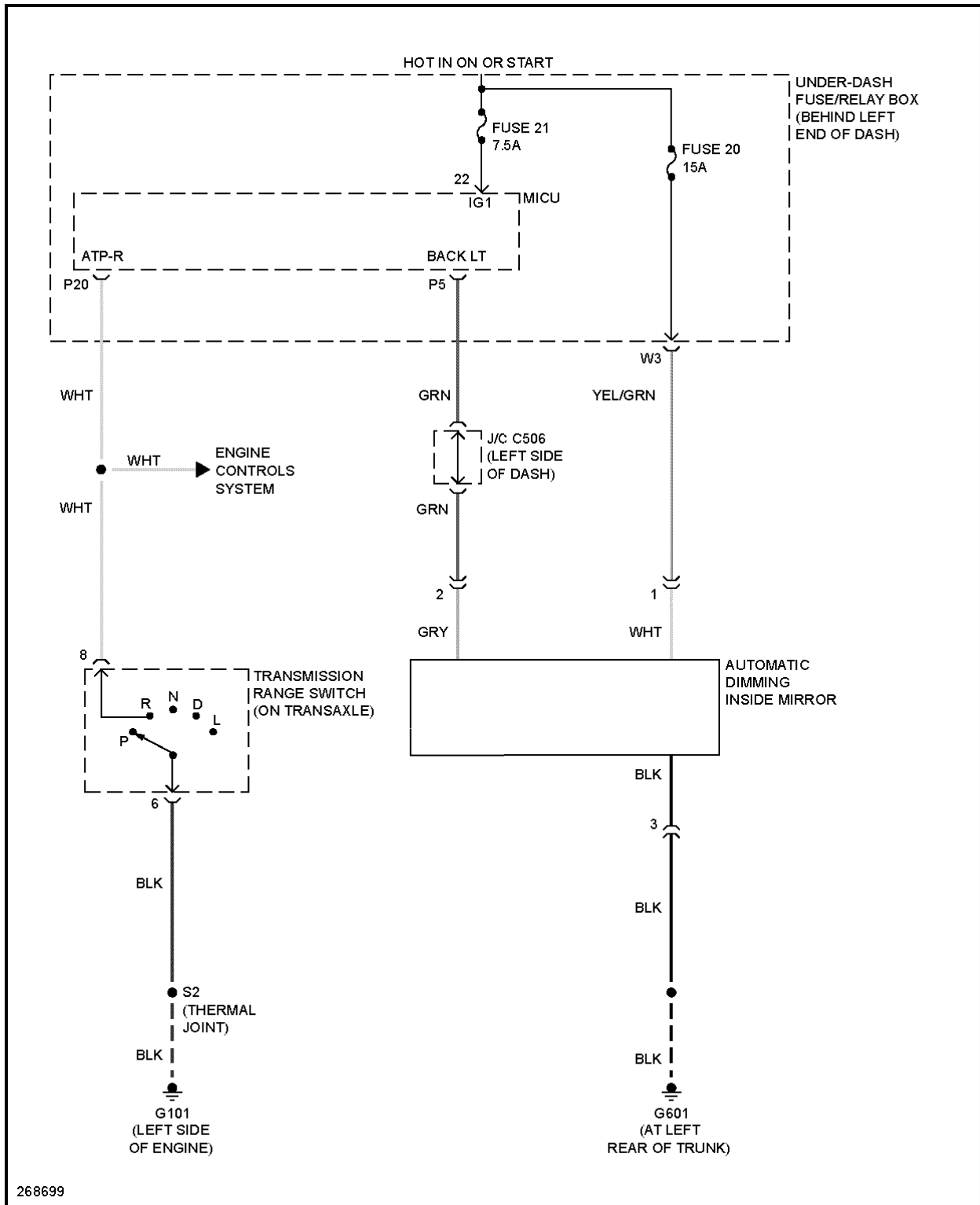
Fig. 77: Automatic Day/Night Mirror Circuit, A/T
