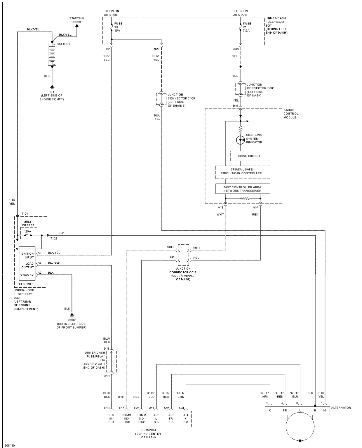
Fig. 94: Charging Circuit
