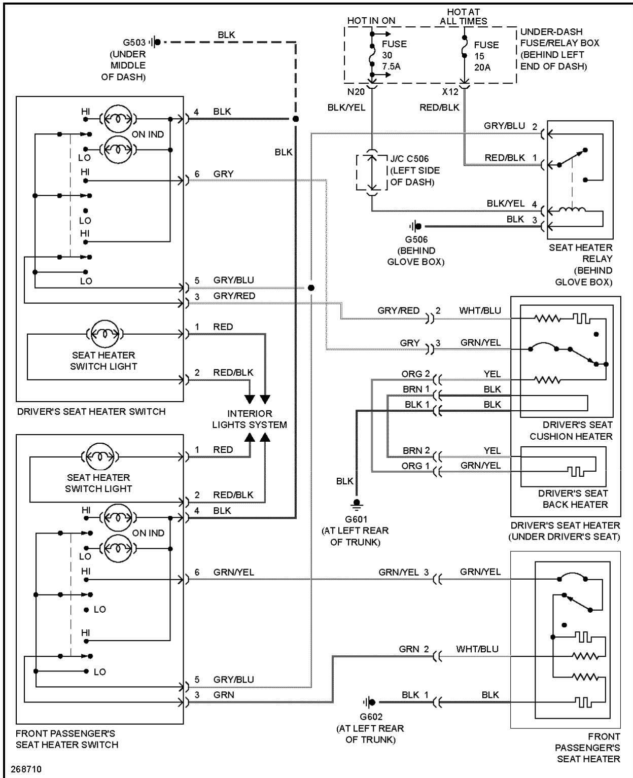
Fig. 80: Heated Seats Circuit
