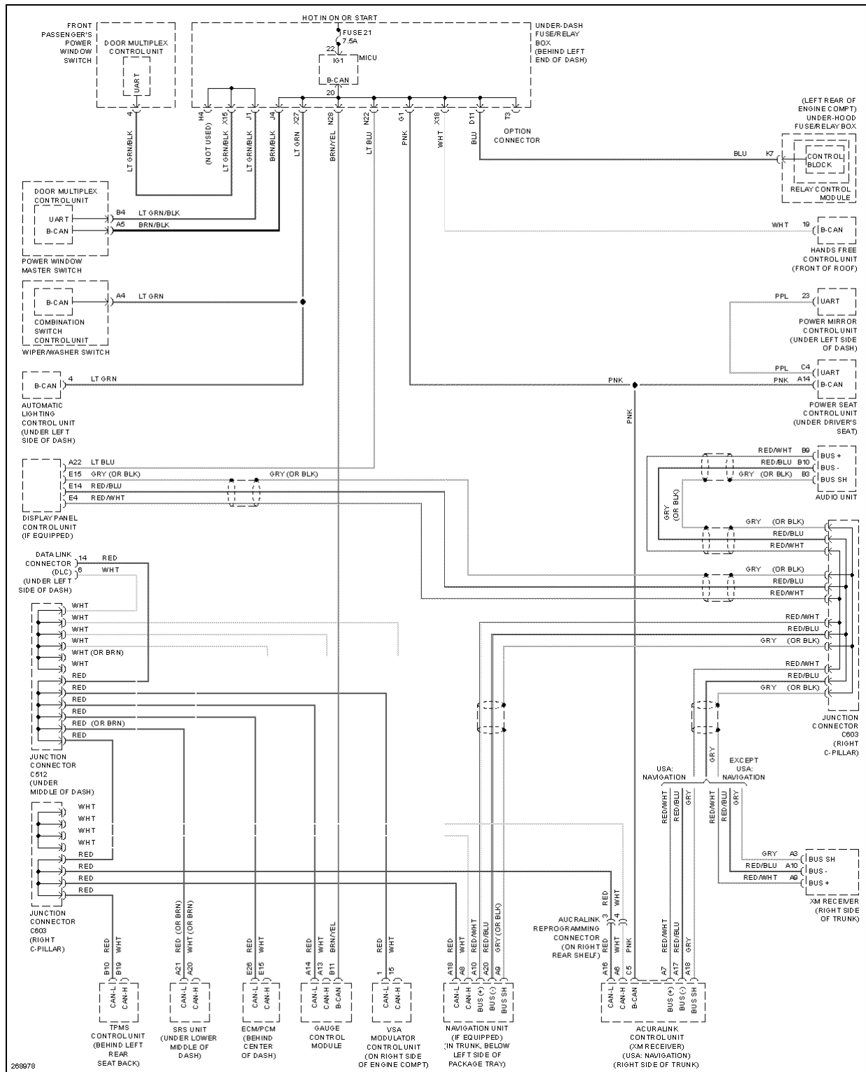
Fig. 12: High/Low Bus Circuit
