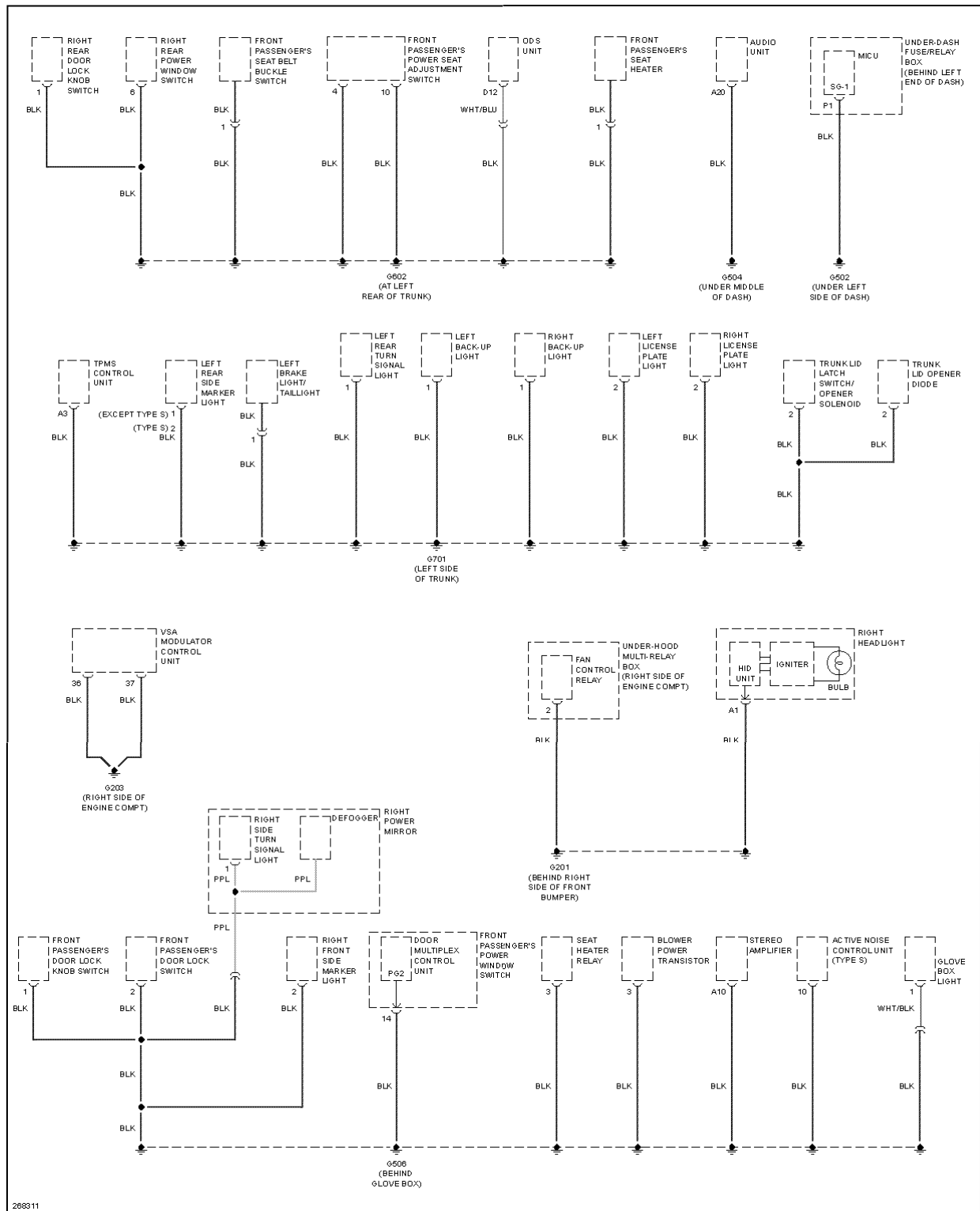
Fig. 43: Ground Distribution Circuit (3 of 4)
