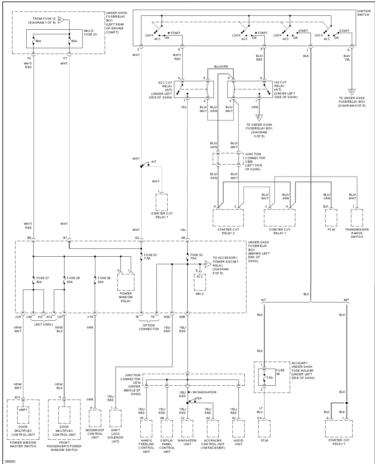
Fig. 71: Power Distribution Circuit (2 of 5)
