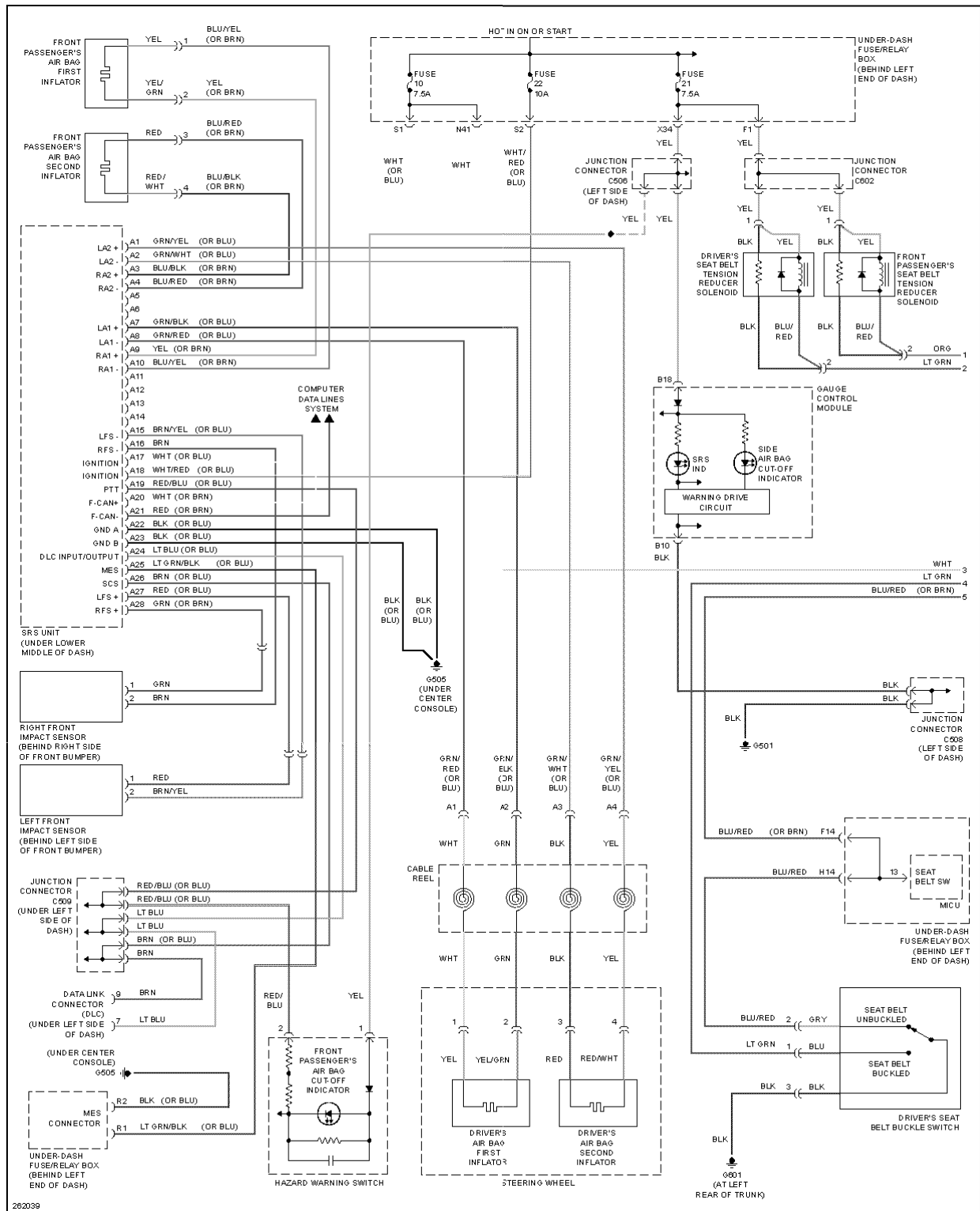
Fig. 97: Supplemental Restraints Circuit (1 of 2)
