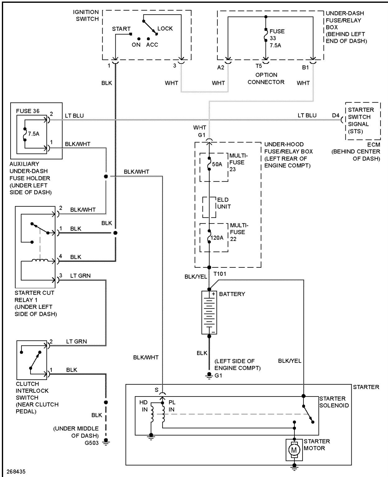
Fig. 96: Starting Circuit, M/T
