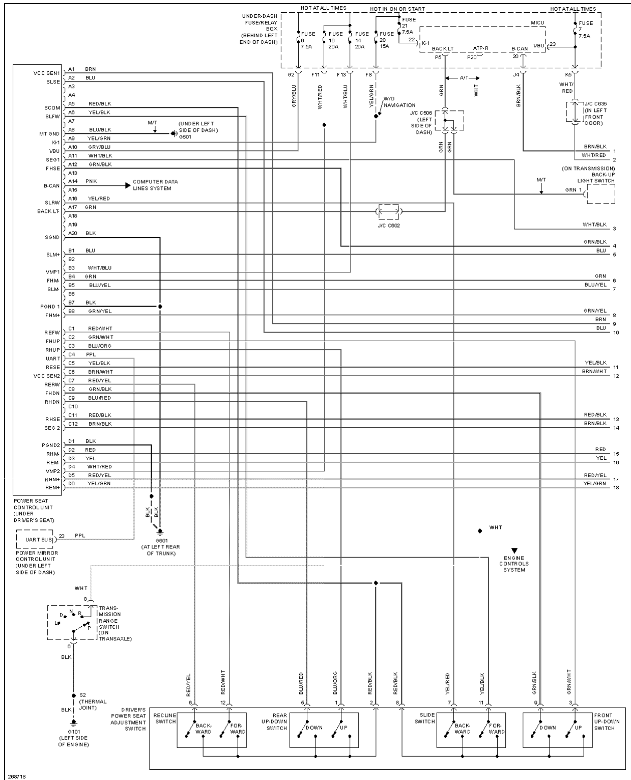
Fig. 57: Driver's Memory Seat Circuit (1 of 2)
