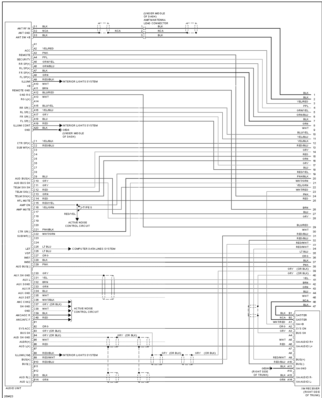
Fig. 89: Radio Circuit, W/O Navigation (1 of 3)
