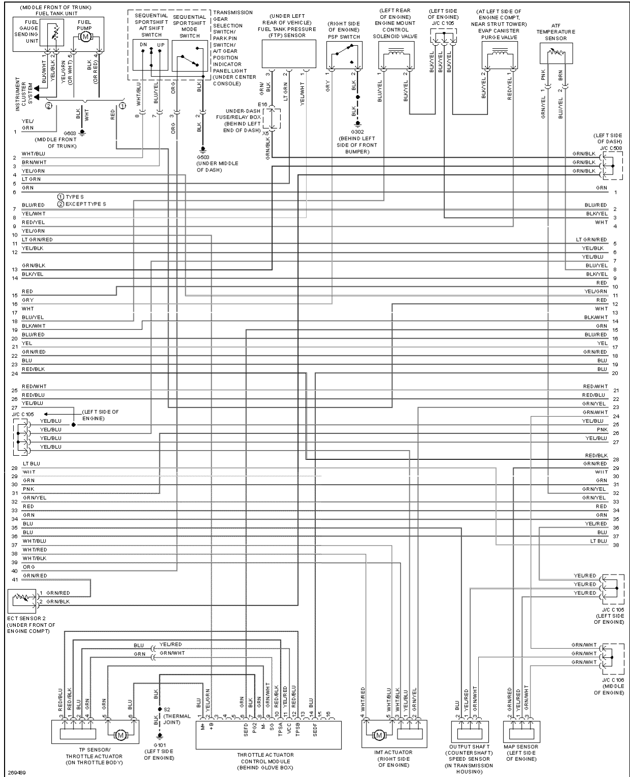
Fig. 18: 3.2L, Engine Performance Circuit, A/T (2 of 5)
