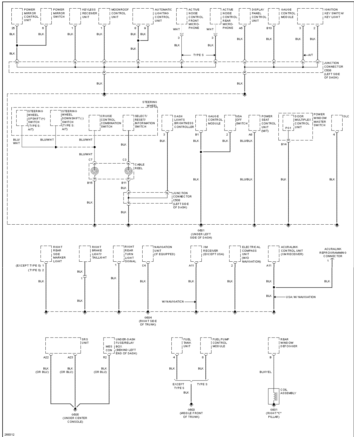
Fig. 44: Ground Distribution Circuit (4 of 4)
