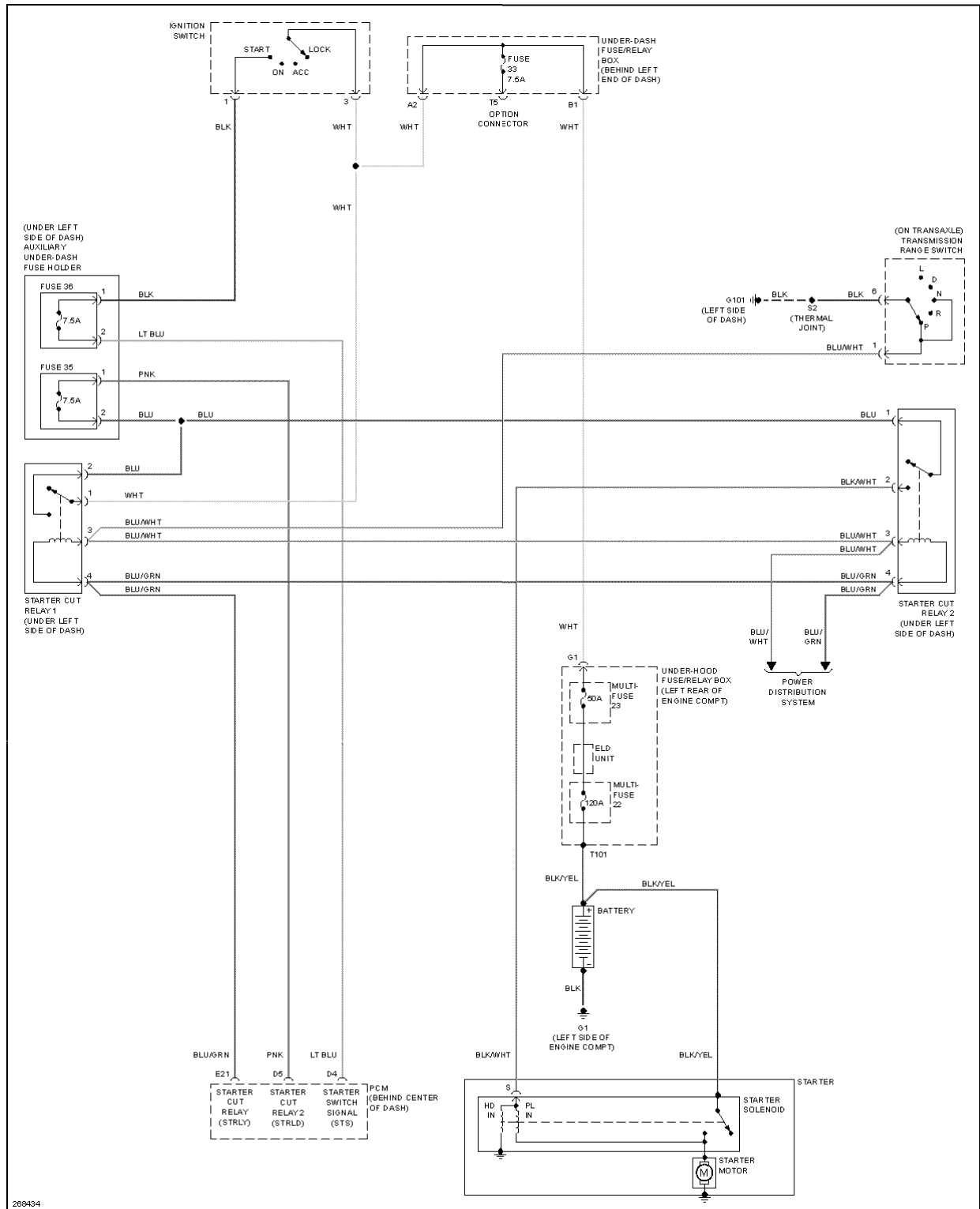
Fig. 95: Starting Circuit, A/T
