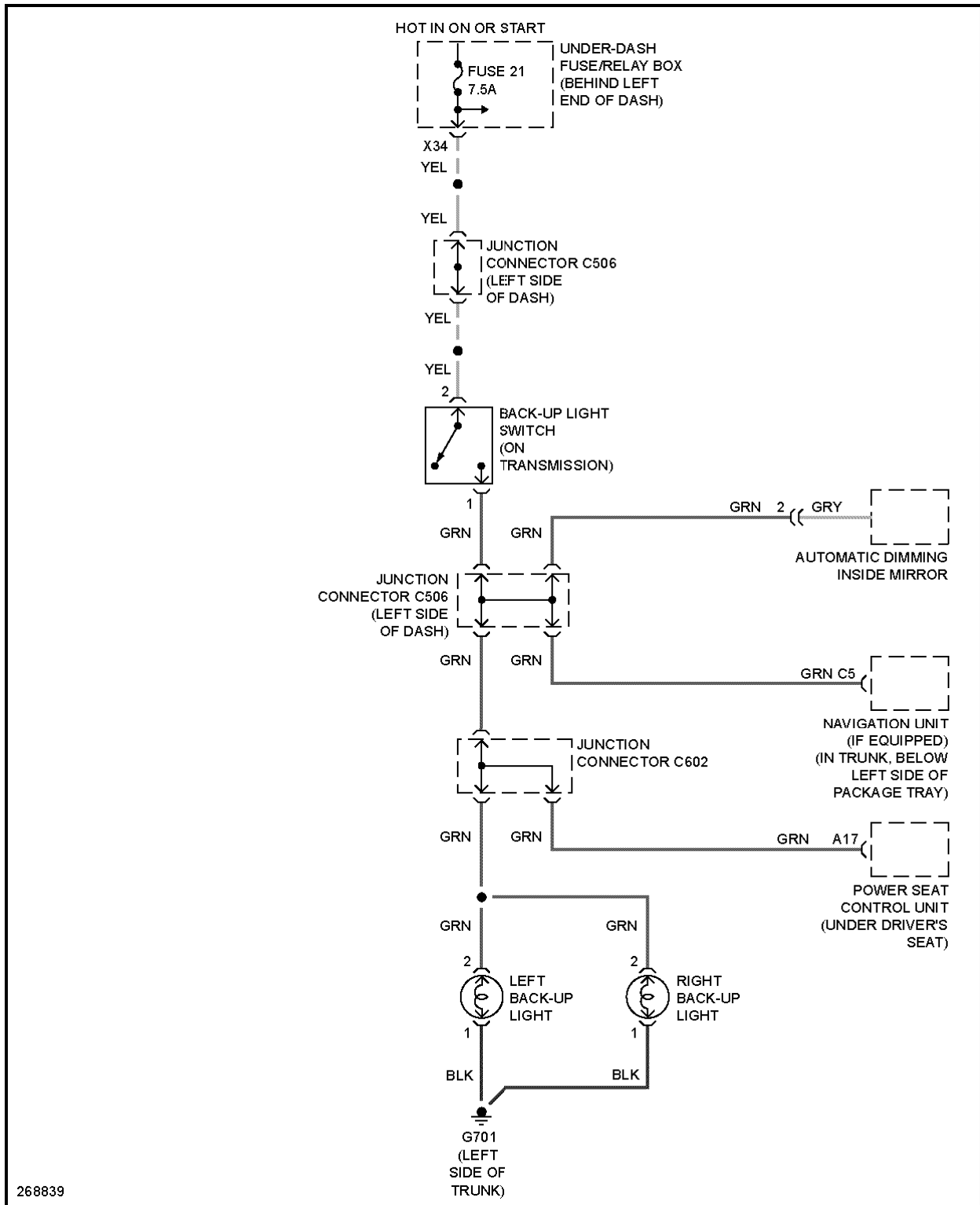
Fig. 38: Backup Lamps Circuit, M/T
