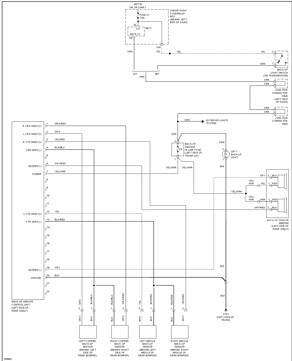
Fig. 67: Parking Assistant Circuit, Accessory
