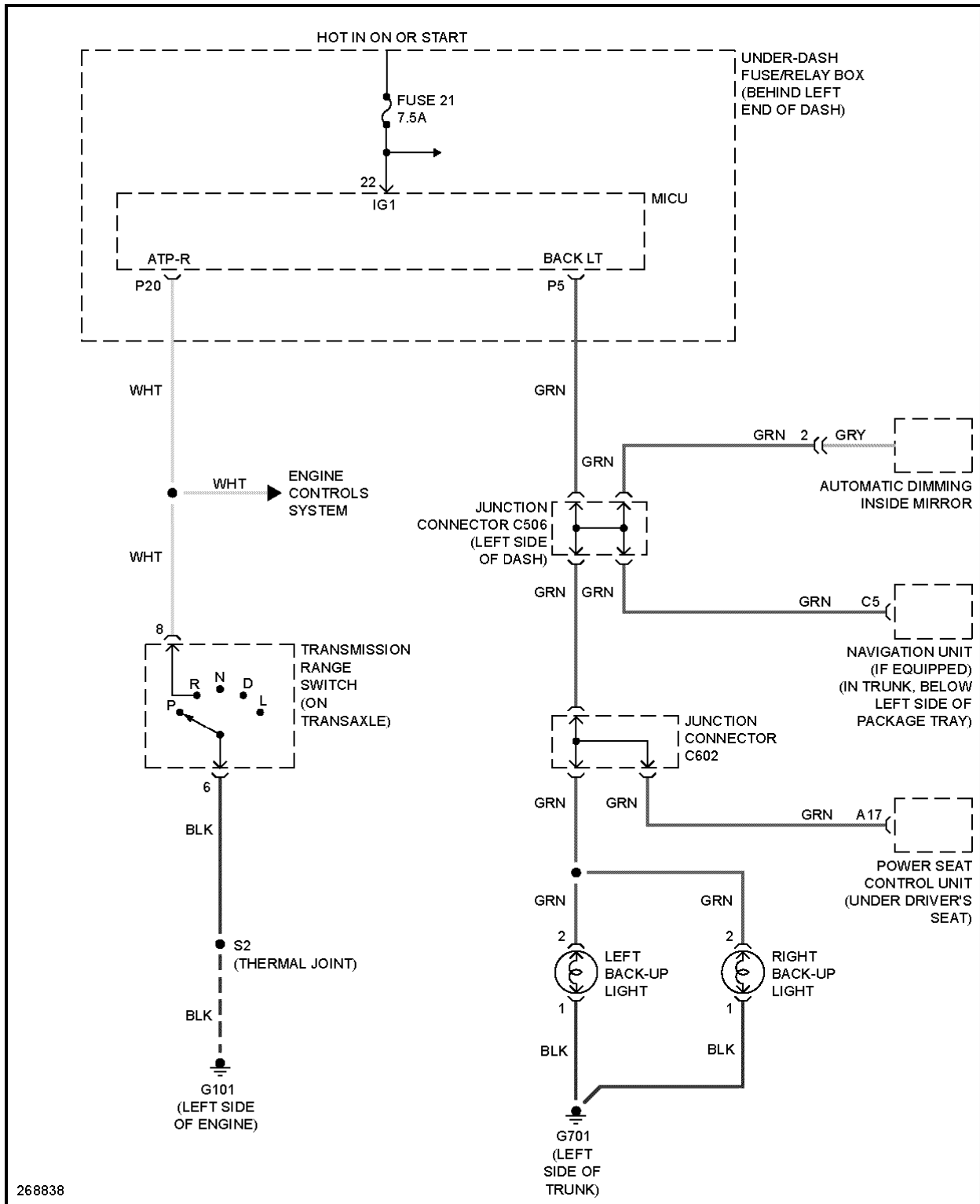
Fig. 37: Backup Lamps Circuit, A/T
