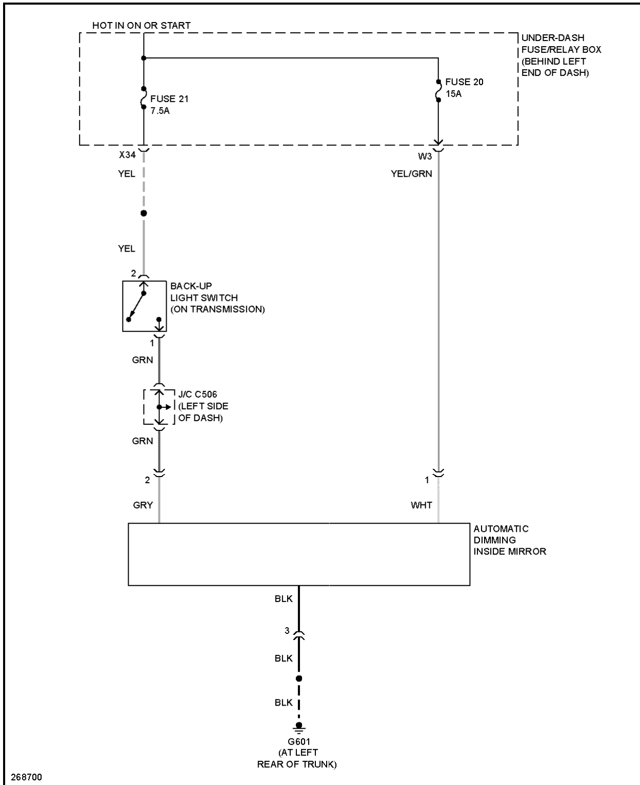
Fig. 78: Automatic Day/Night Mirror Circuit, M/T
