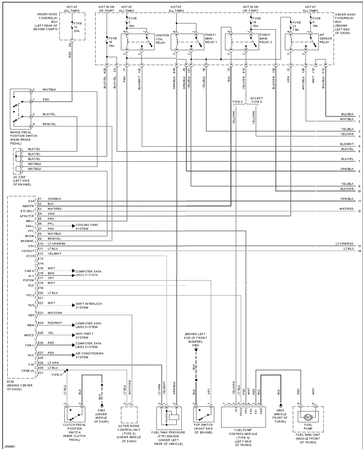
Fig. 32: 3.5L, Engine Performance Circuit, M/T (1 of 5)
