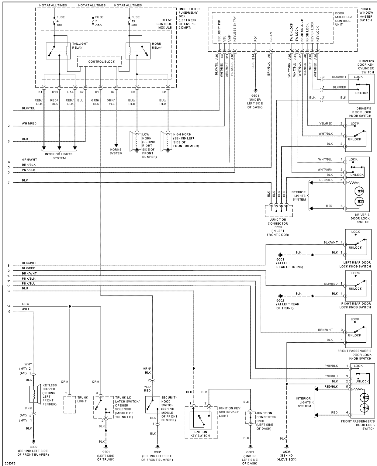
Fig. 76: Power Door Locks Circuit (2 of 2)
