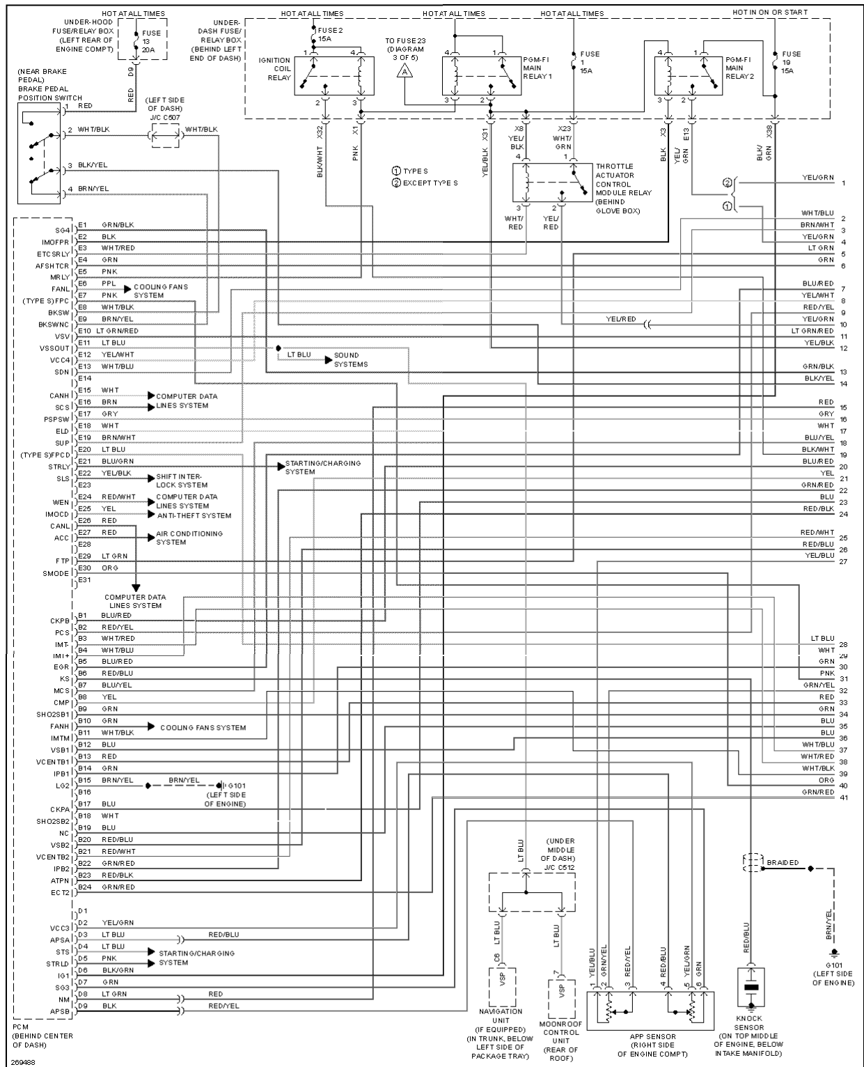
Fig. 27: 3.5L, Engine Performance Circuit, A/T (1 of 5)
