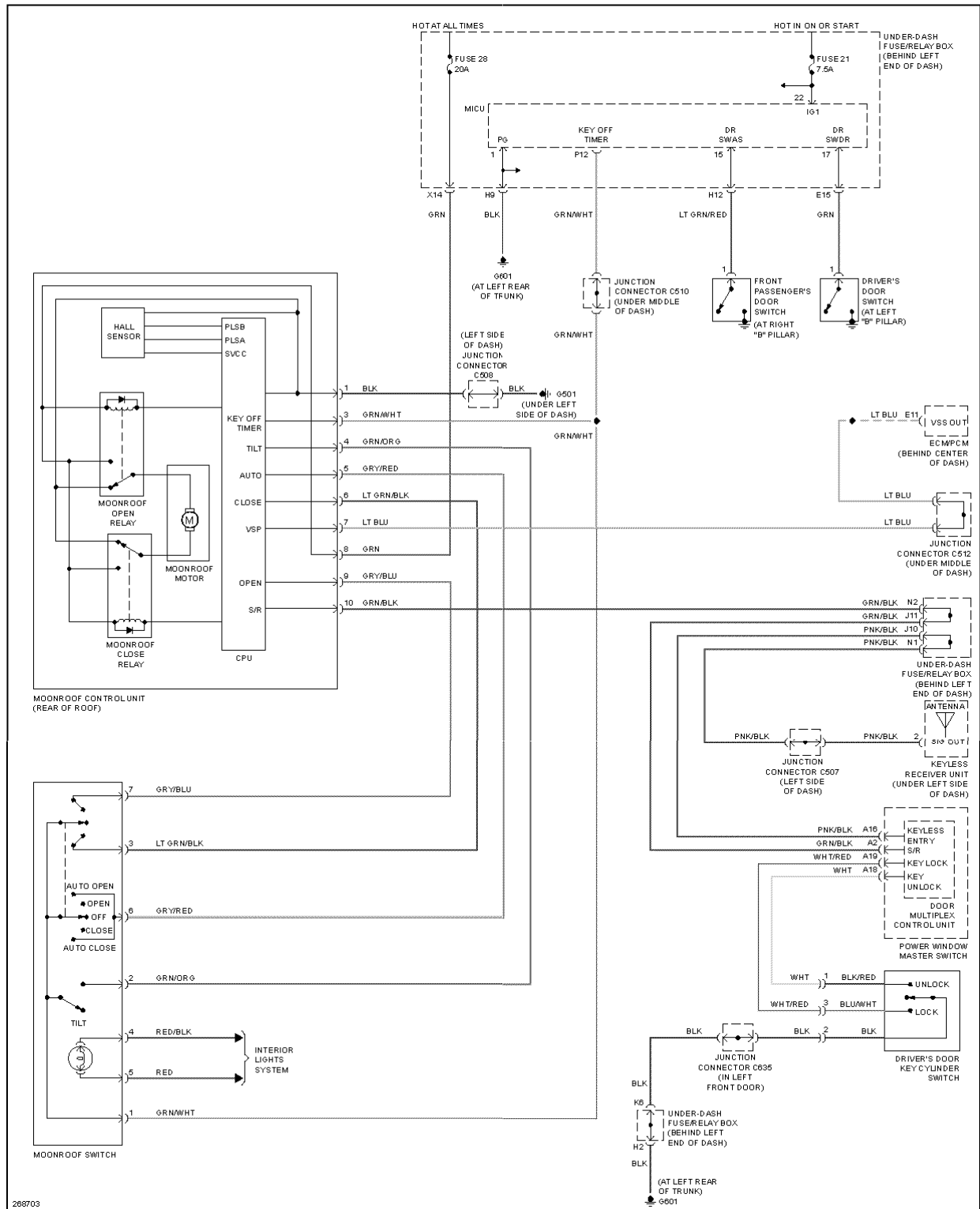
Fig. 82: Power Top/Sunroof Circuit
