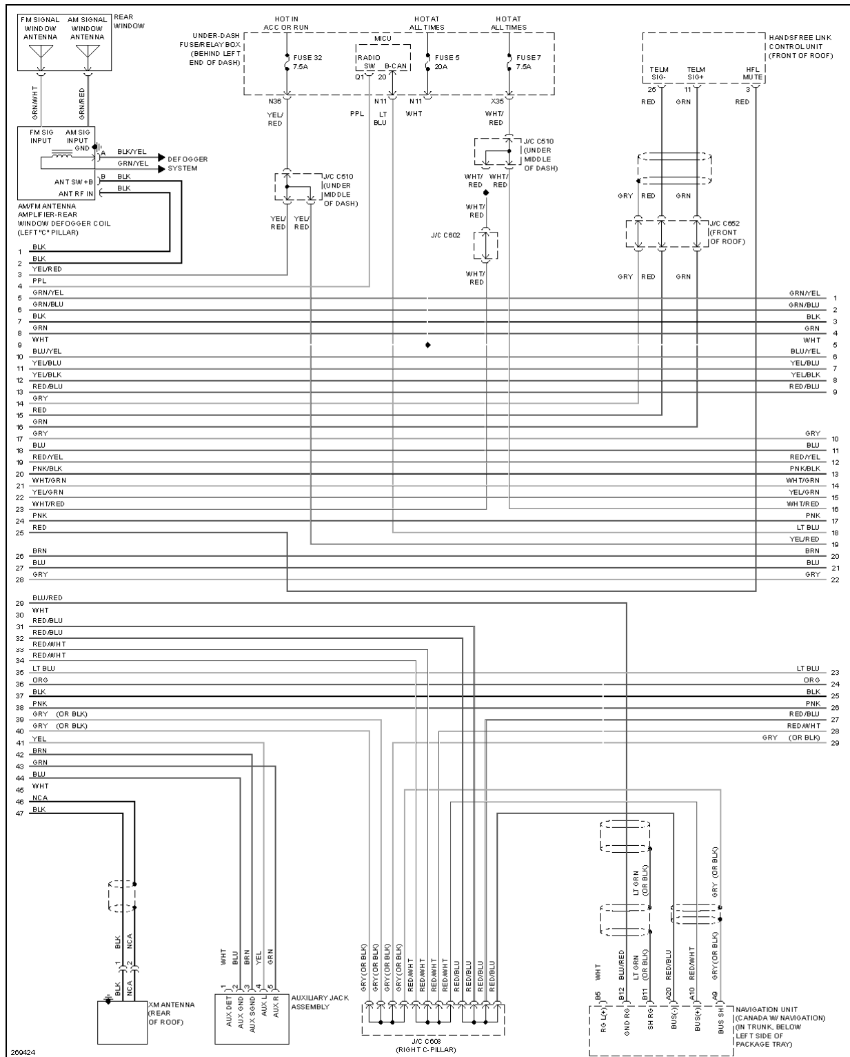
Fig. 90: Radio Circuit, W/O Navigation (2 of 3)
