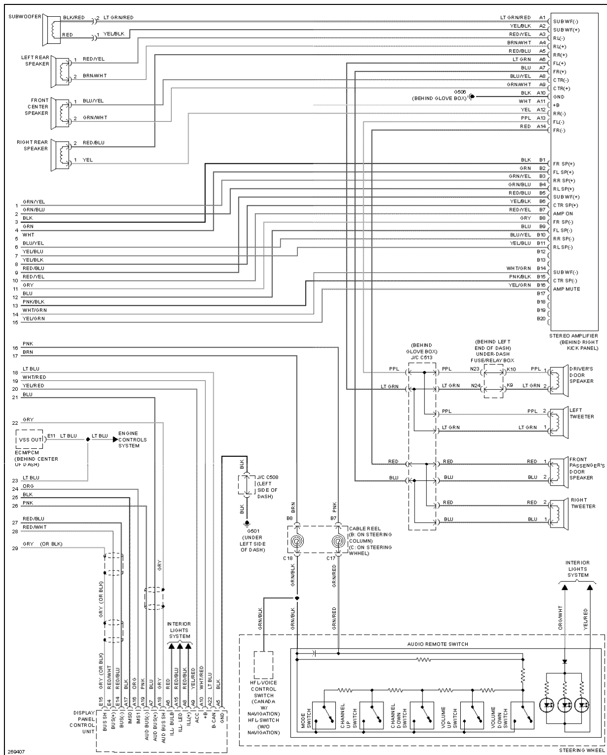
Fig. 88: Radio Circuit, W/ Navigation (3 of 3)
