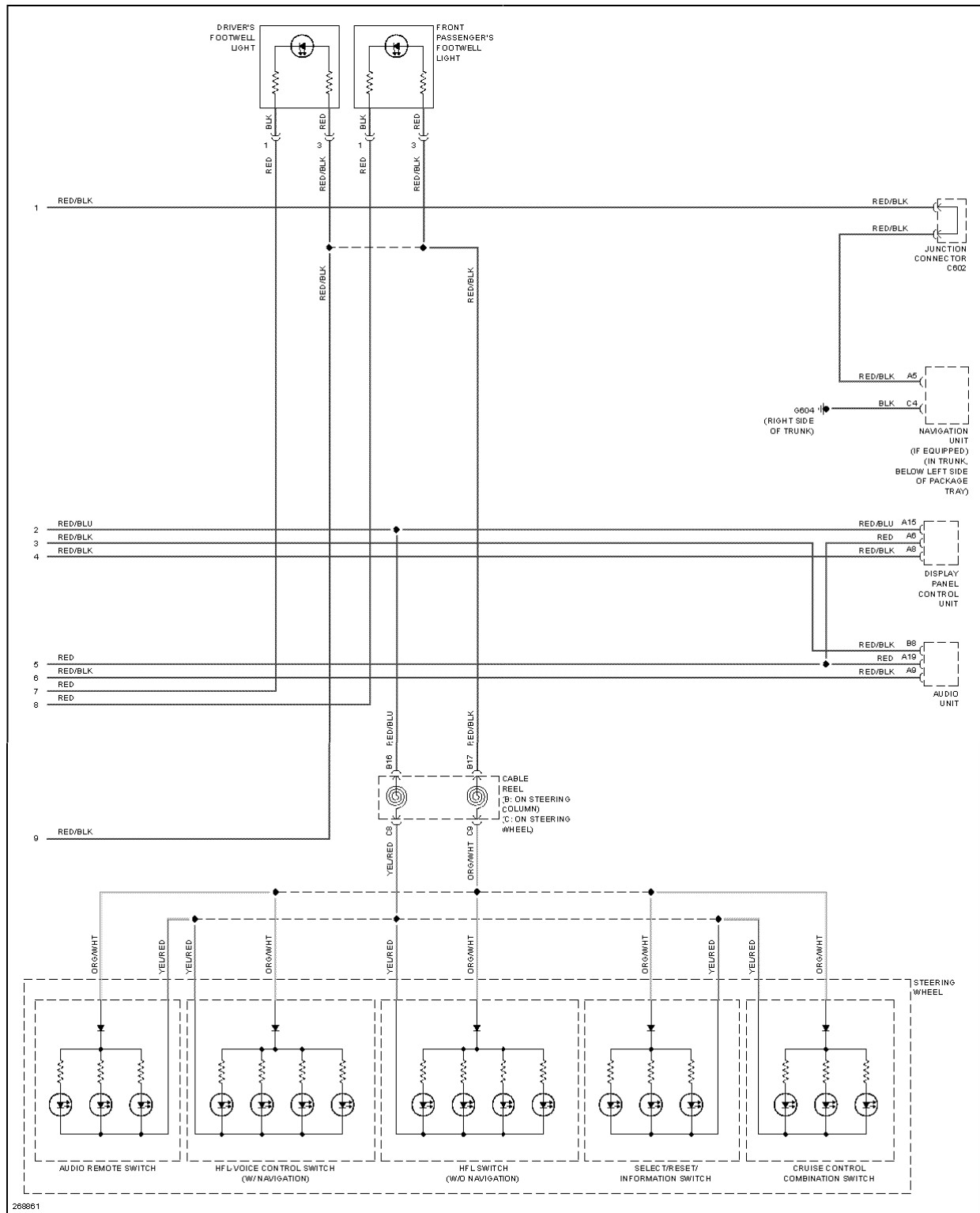
Fig. 56: Instrument Illumination Circuit (3 of 3)
