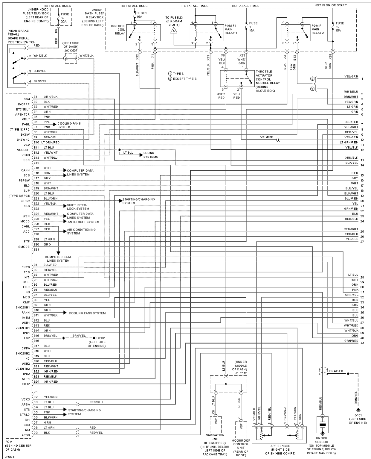
Fig. 17: 3.2L, Engine Performance Circuit, A/T (1 of 5)
