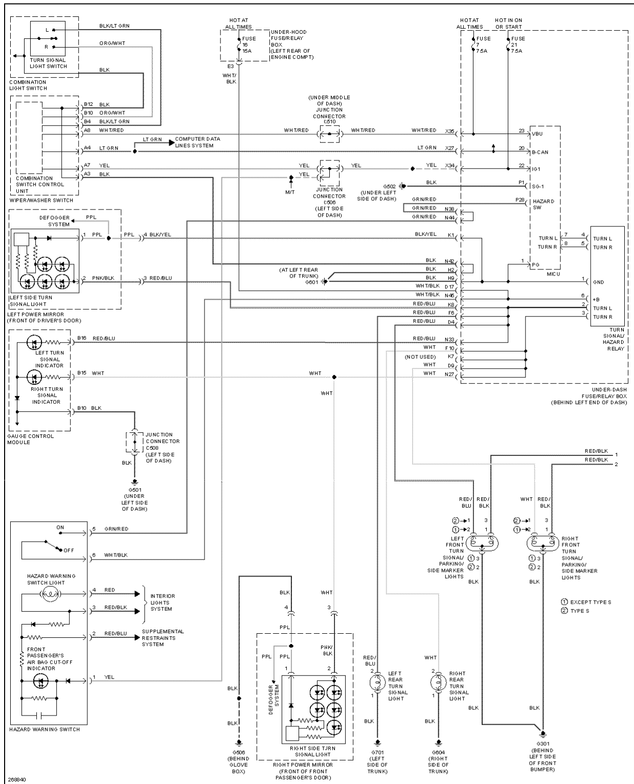
Fig. 39: Exterior Lamps Circuit (1 of 2)
