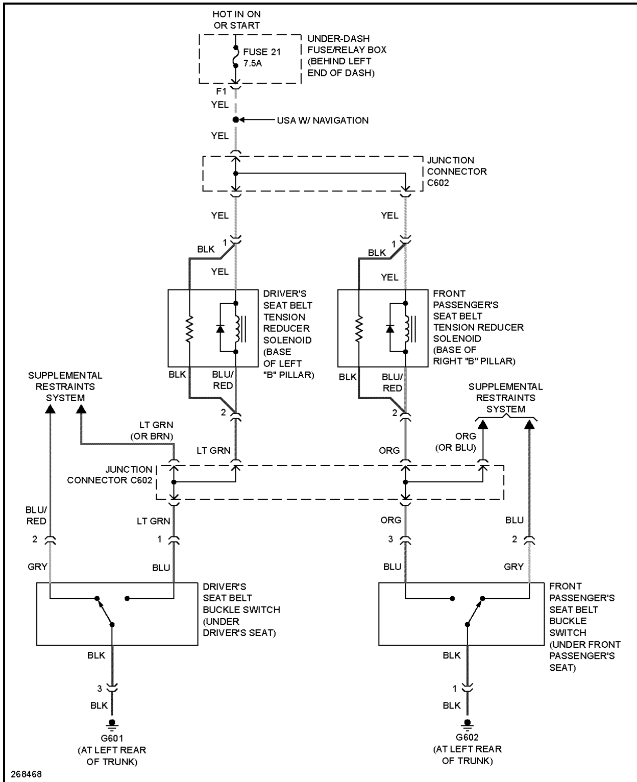
Fig. 69: Passive Restraints Circuit
