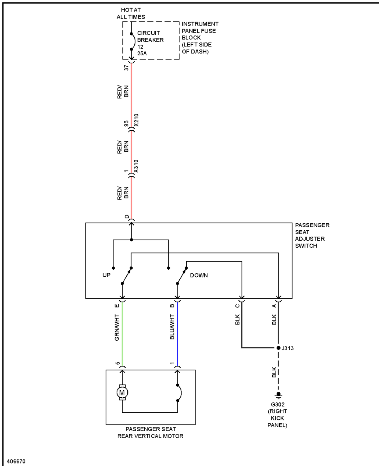
Fig. 107: Passenger Power Seat Circuit, 2-Way Power Seat
