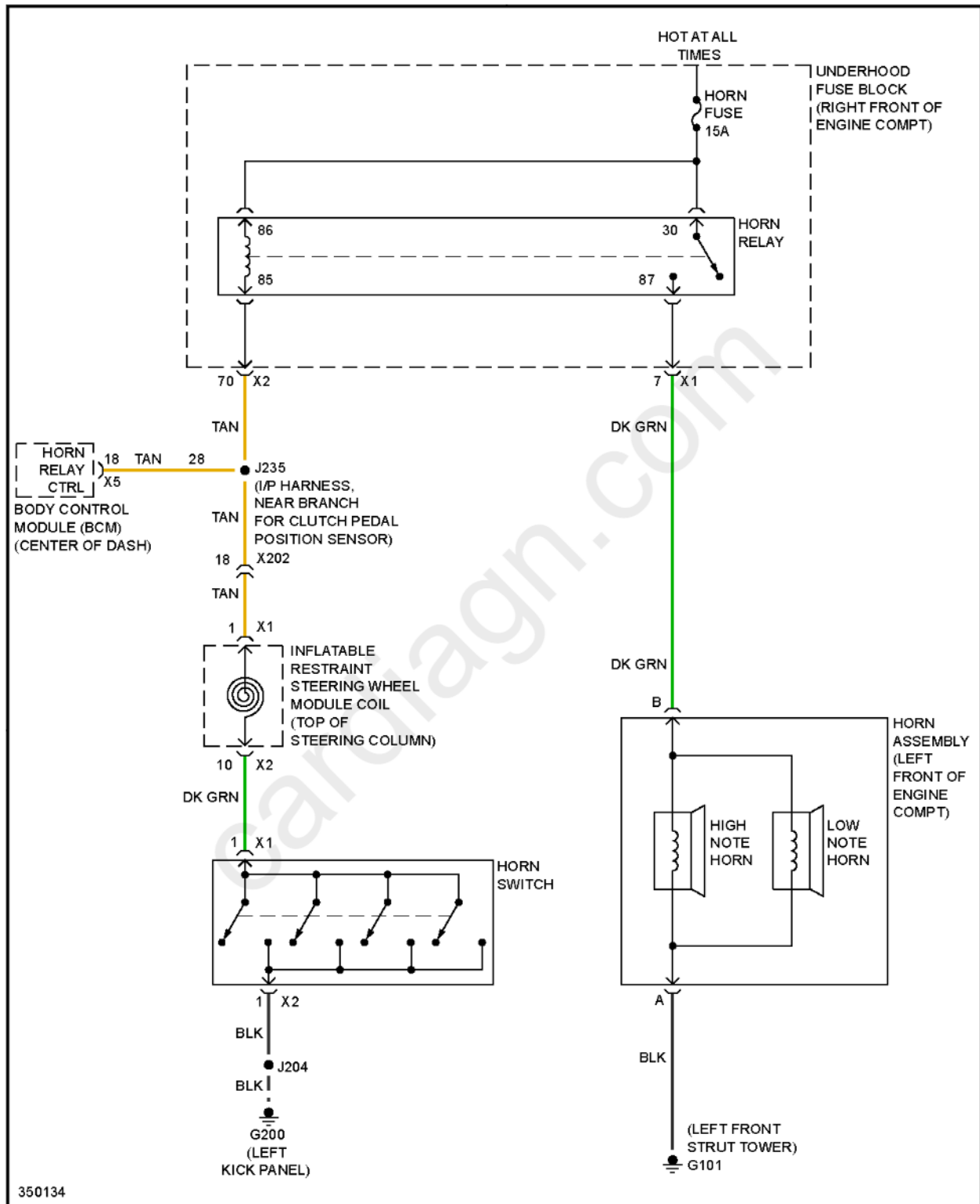
Fig. 53: Horn Circuit
