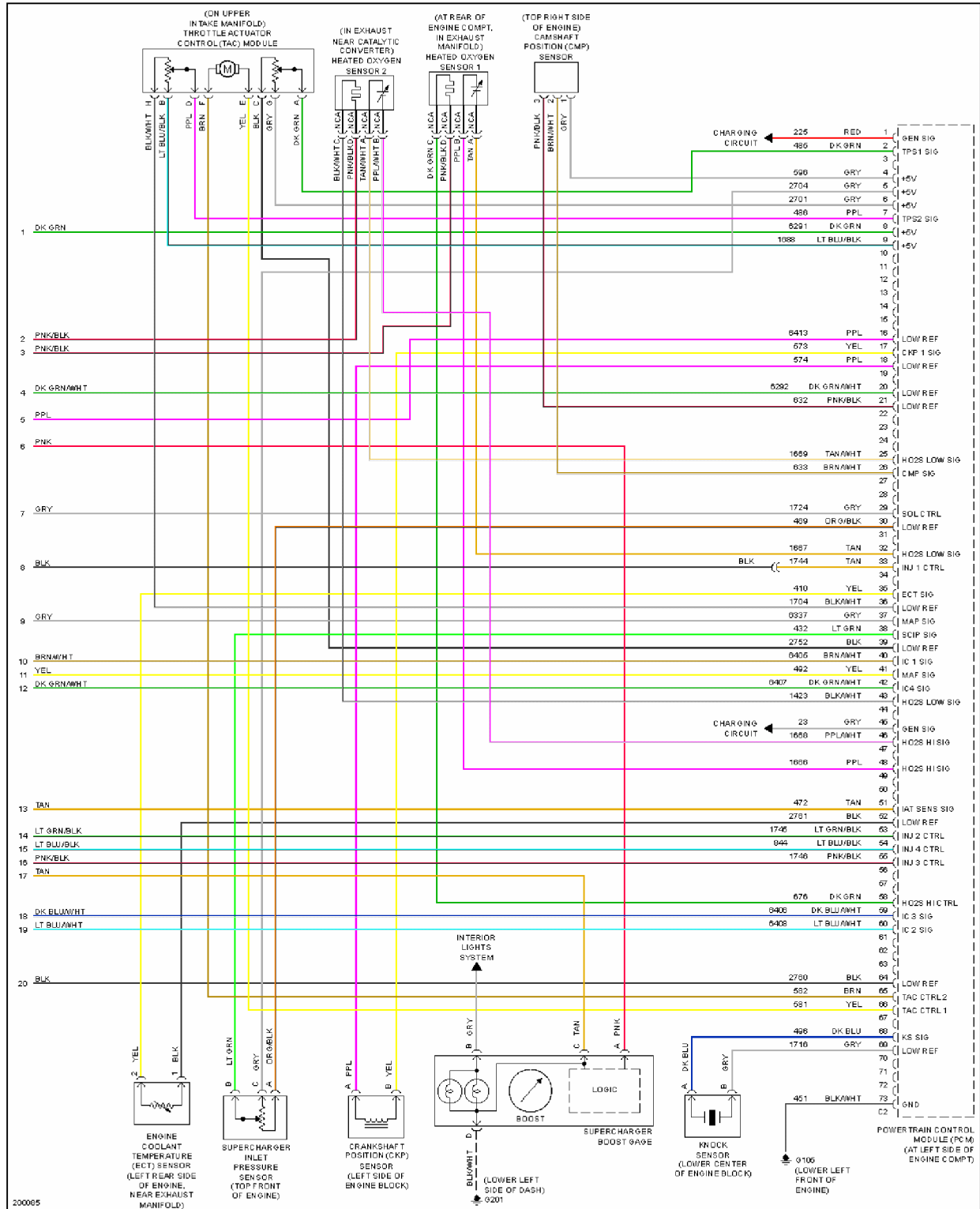
Fig. 24: 2.0L VIN P, Engine Performance Circuit (4 of 4)
