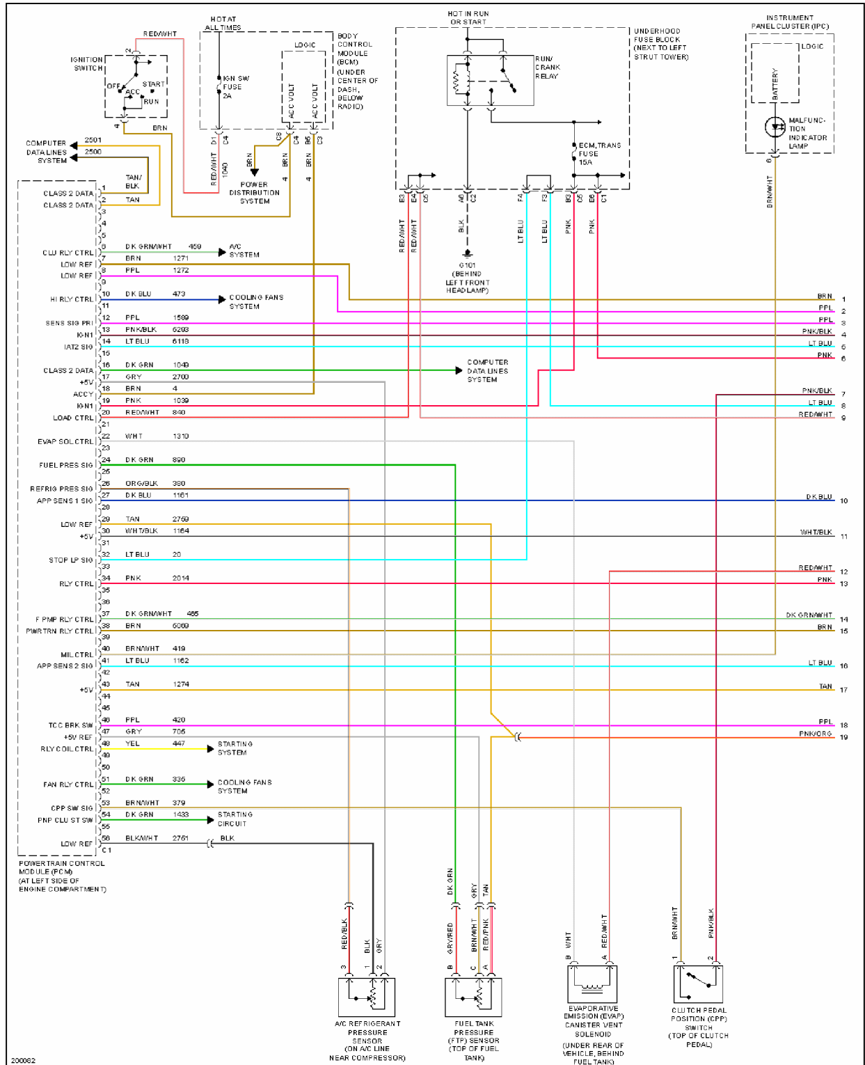
Fig. 21: 2.0L VIN P, Engine Performance Circuit (1 of 4)
