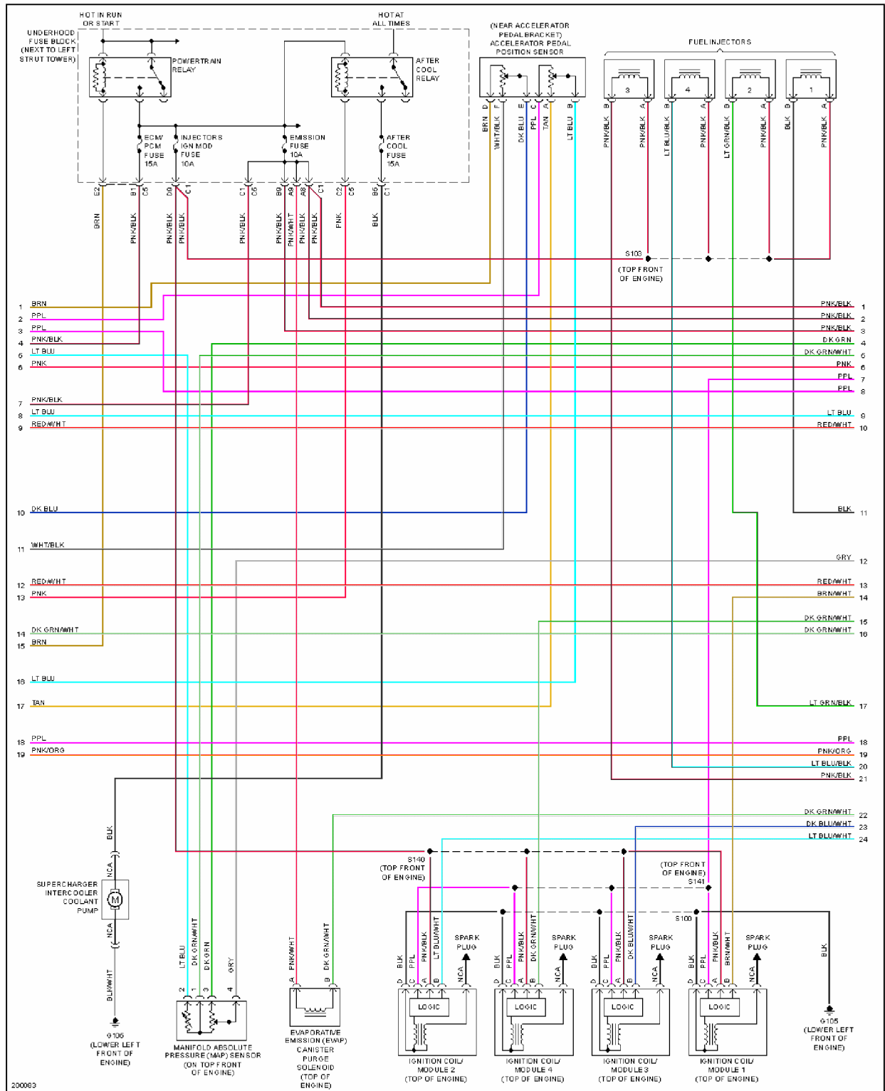
Fig. 22: 2.0L VIN P, Engine Performance Circuit (2 of 4)
