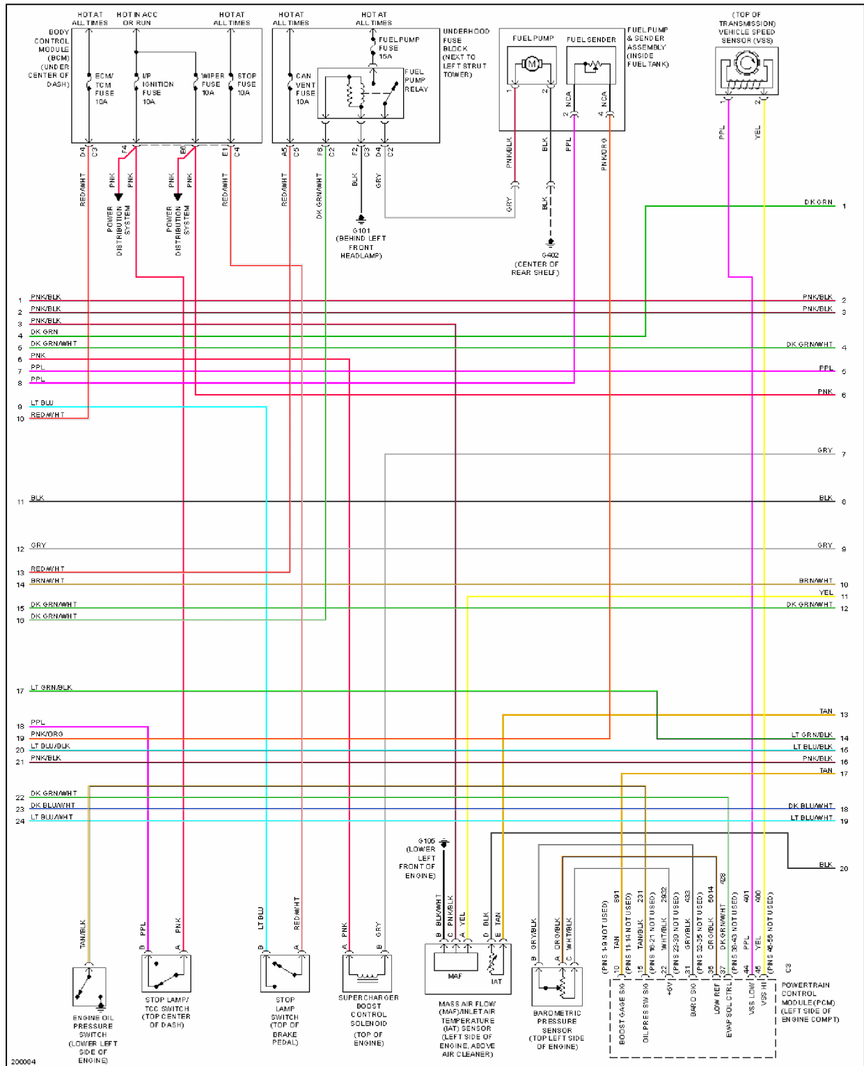
Fig. 23: 2.0L VIN P, Engine Performance Circuit (3 of 4)
