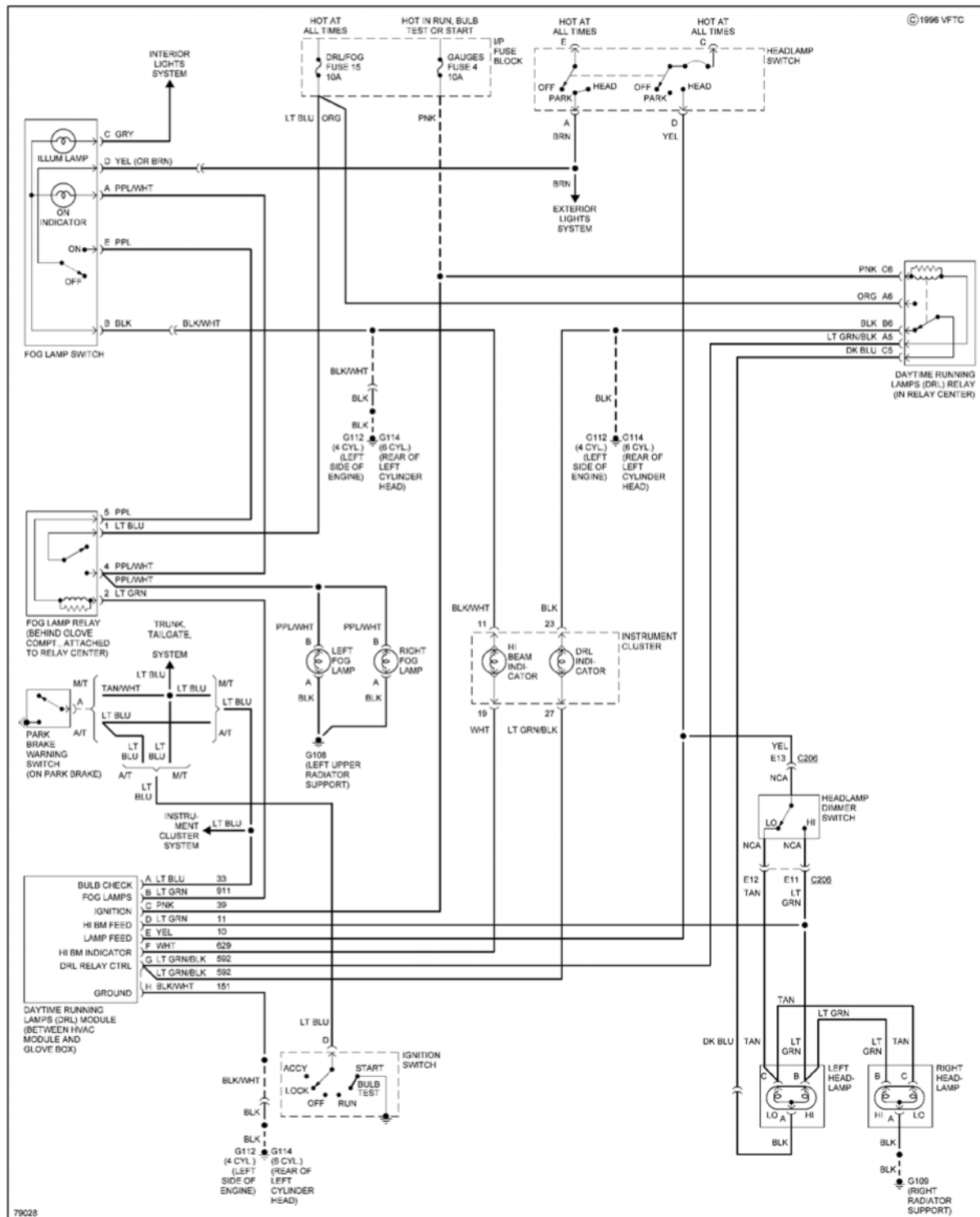
Fig. 15: Headlight Circuit, W/ Sealed Beam Lamps
