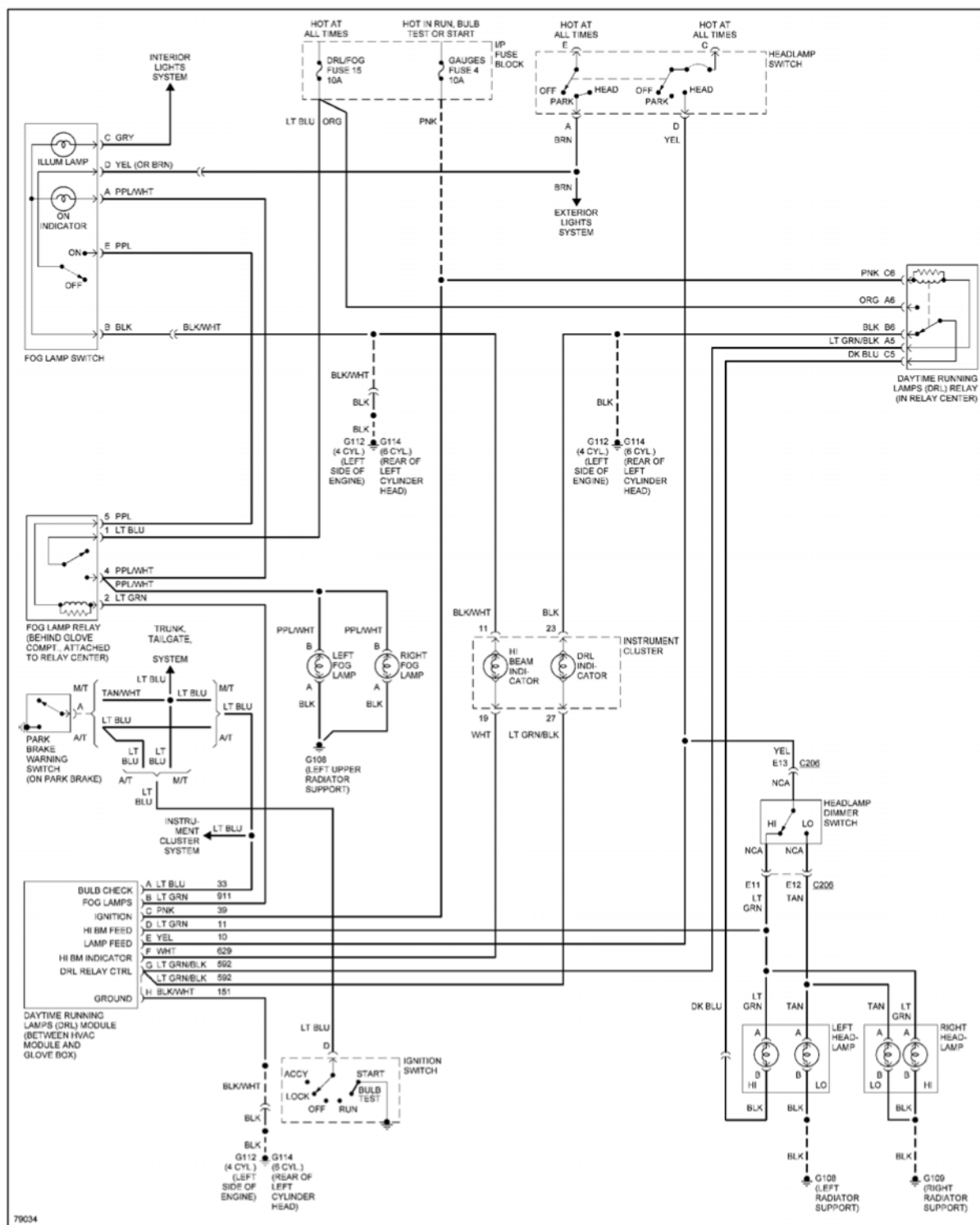
Fig. 14: Headlight Circuit, W/ Composite Headlamps
