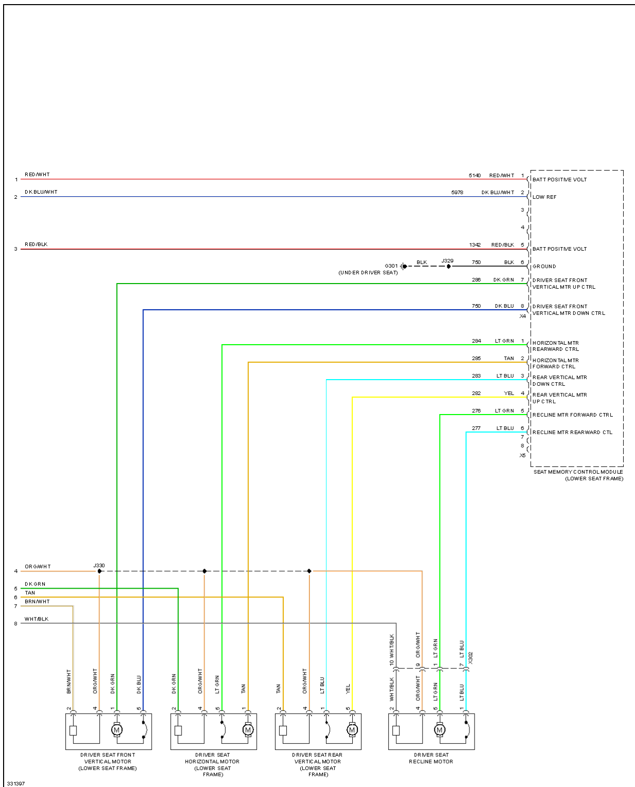
Fig. 44: Driver's Memory Seat Circuit (2 of 2)
