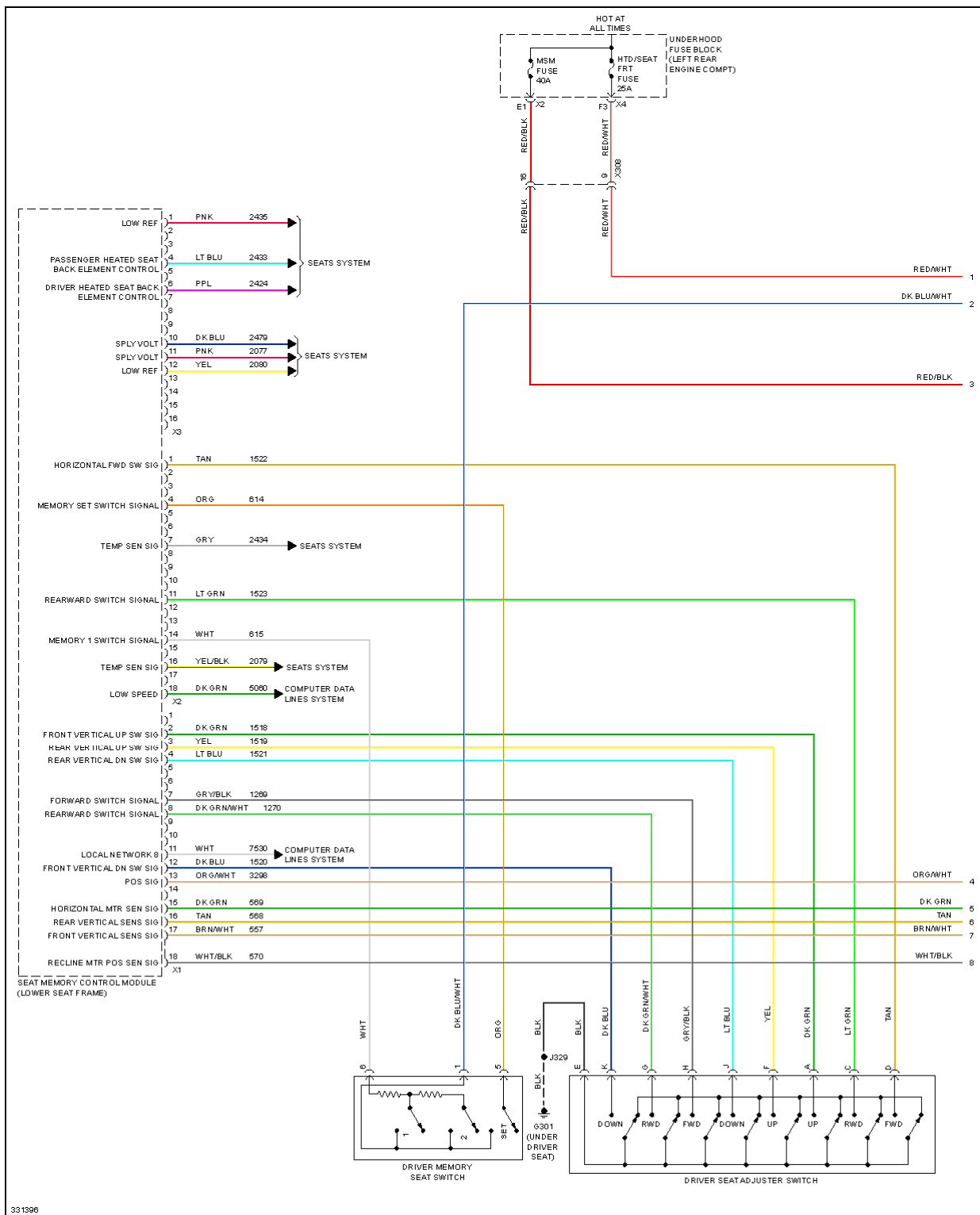
Fig. 43: Driver's Memory Seat Circuit (1 of 2)
