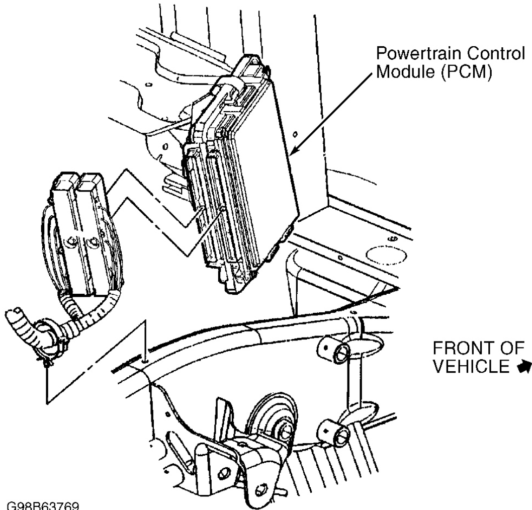
Fig. 10: Left Front Of Engine Compartment (4.8L VIN V, 5.3L VIN T, 6.0L VIN U & 8.1L VIN G) Courtesy of GENERAL MOTORS CORP.
