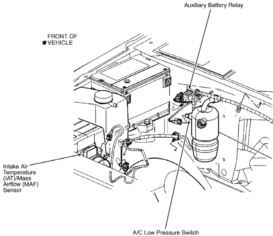
Fig. 9: Right Rear Of Engine Compartment Courtesy of GENERAL MOTORS CORP.
