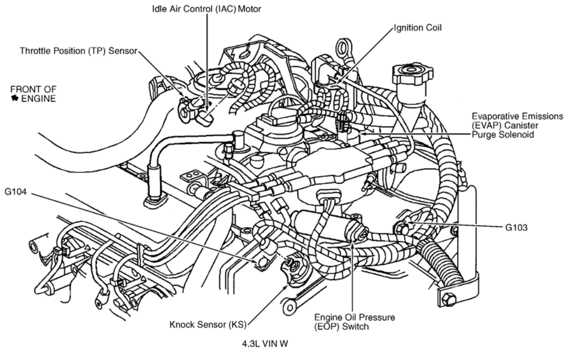
Fig. 1: Rear Of Engine (4.3L VIN W) Courtesy of GENERAL MOTORS CORP.
