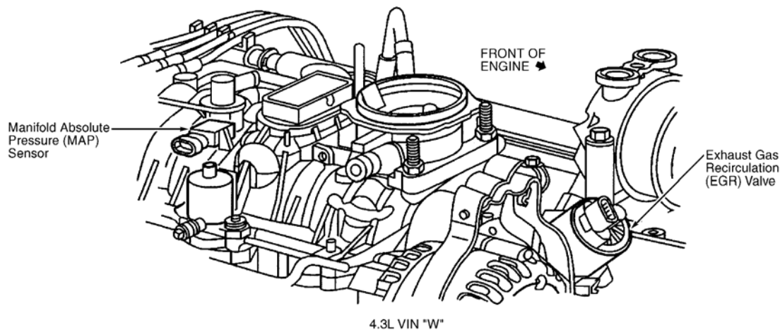
Fig. 4: Top Of Engine (4.3L VIN W) Courtesy of GENERAL MOTORS CORP.
