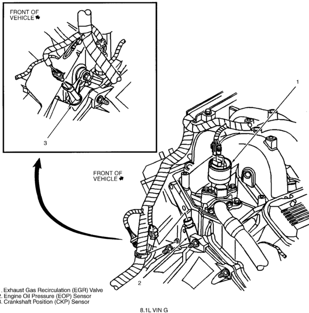
Fig. 8: Rear Of Engine (8.1L VIN G) Courtesy of GENERAL MOTORS CORP.
