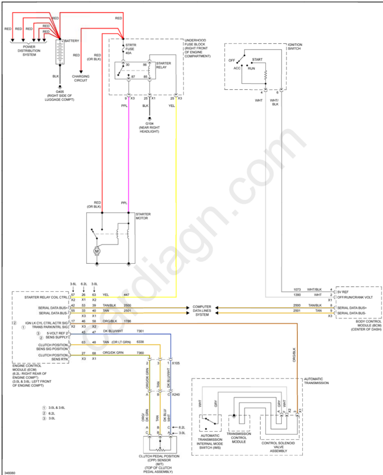
Fig. 112: Starting Circuit
