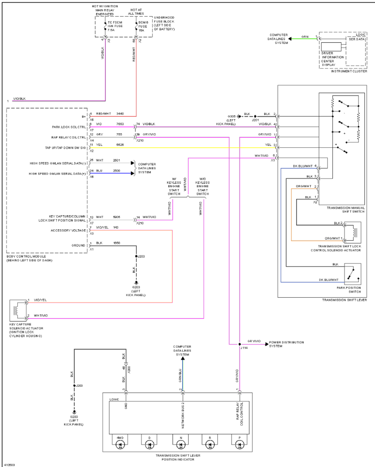
Fig. 133: 2.4L VIN R, Transmission Circuit (2 of 2)
