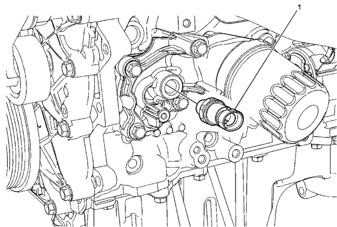
Fig. 192: Engine Oil Pressure Sensor And/Or Switch (LF1) Courtesy of GENERAL MOTORS CORP.
