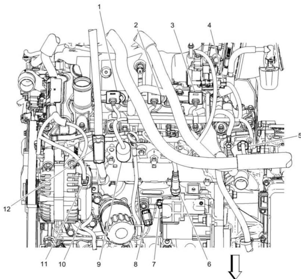
Fig. 4: Engine Components -- Front Courtesy of GENERAL MOTORS COMPANY
