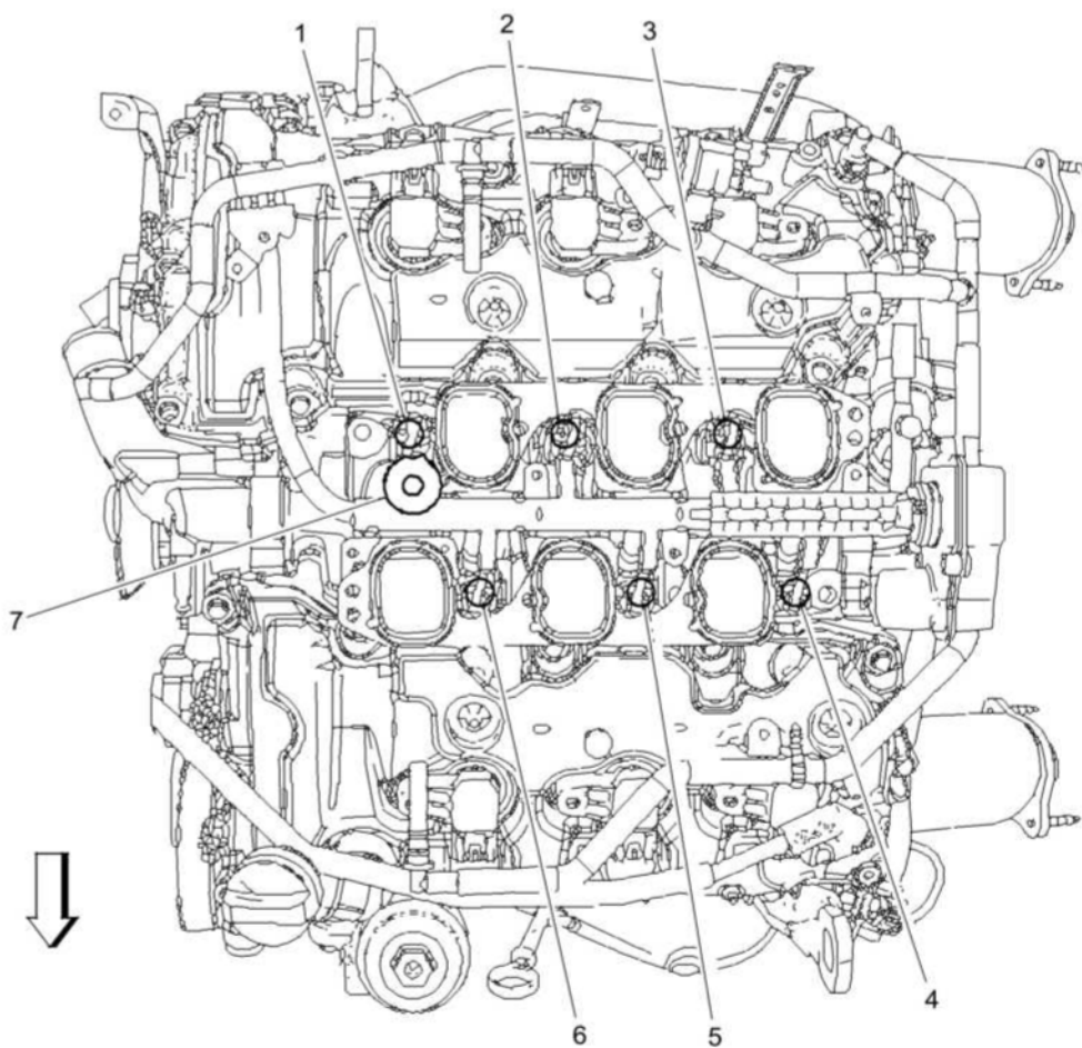
Fig. 1: Identifying Engine - Top Components (LLT) Courtesy of GENERAL MOTORS COMPANY
