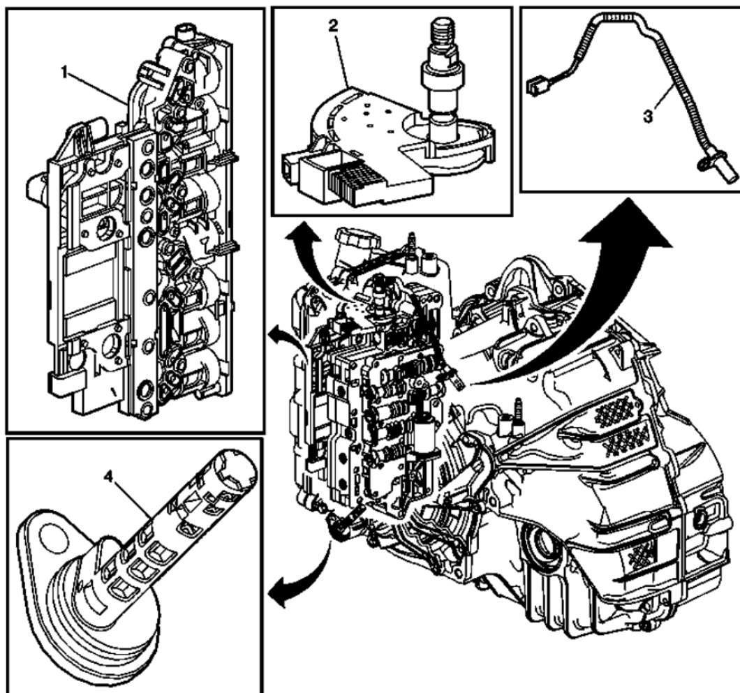
Fig. 3: Identifying Automatic Transmission Electronic Components Courtesy of GENERAL MOTORS COMPANY
