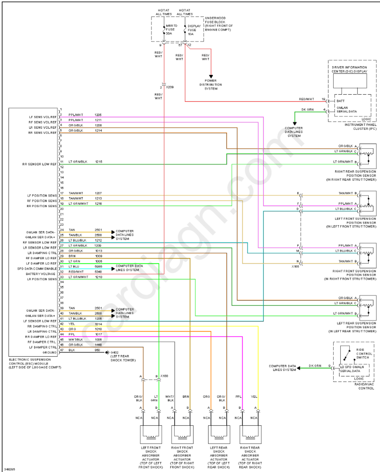
Fig. 25: Electronic Suspension Circuit
