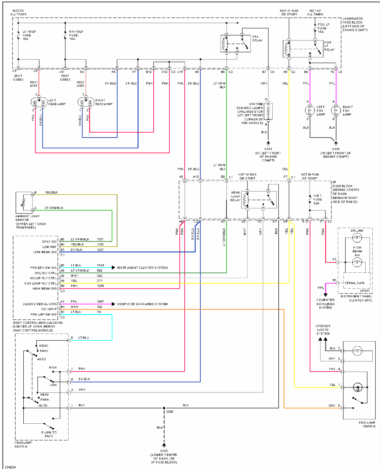
Fig. 22: Headlights Circuit
