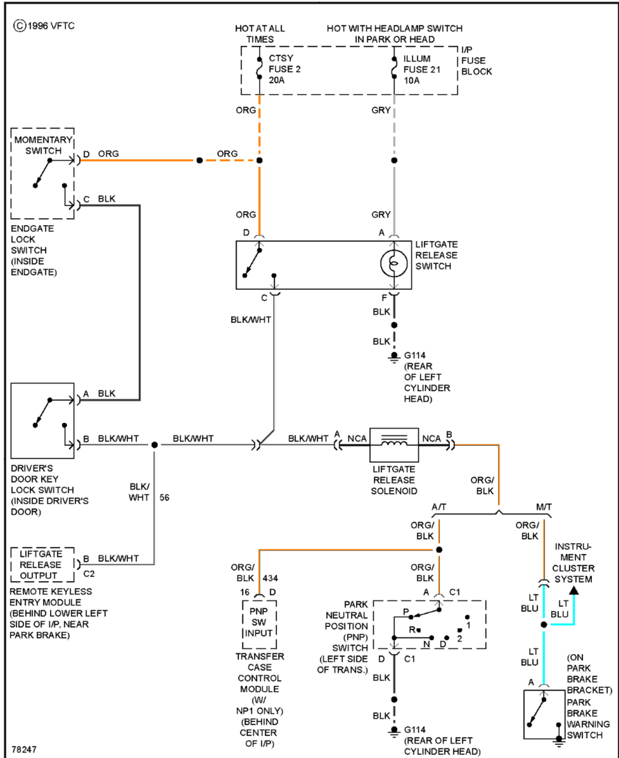
Fig. 39: Rear Glass Release Circuit
