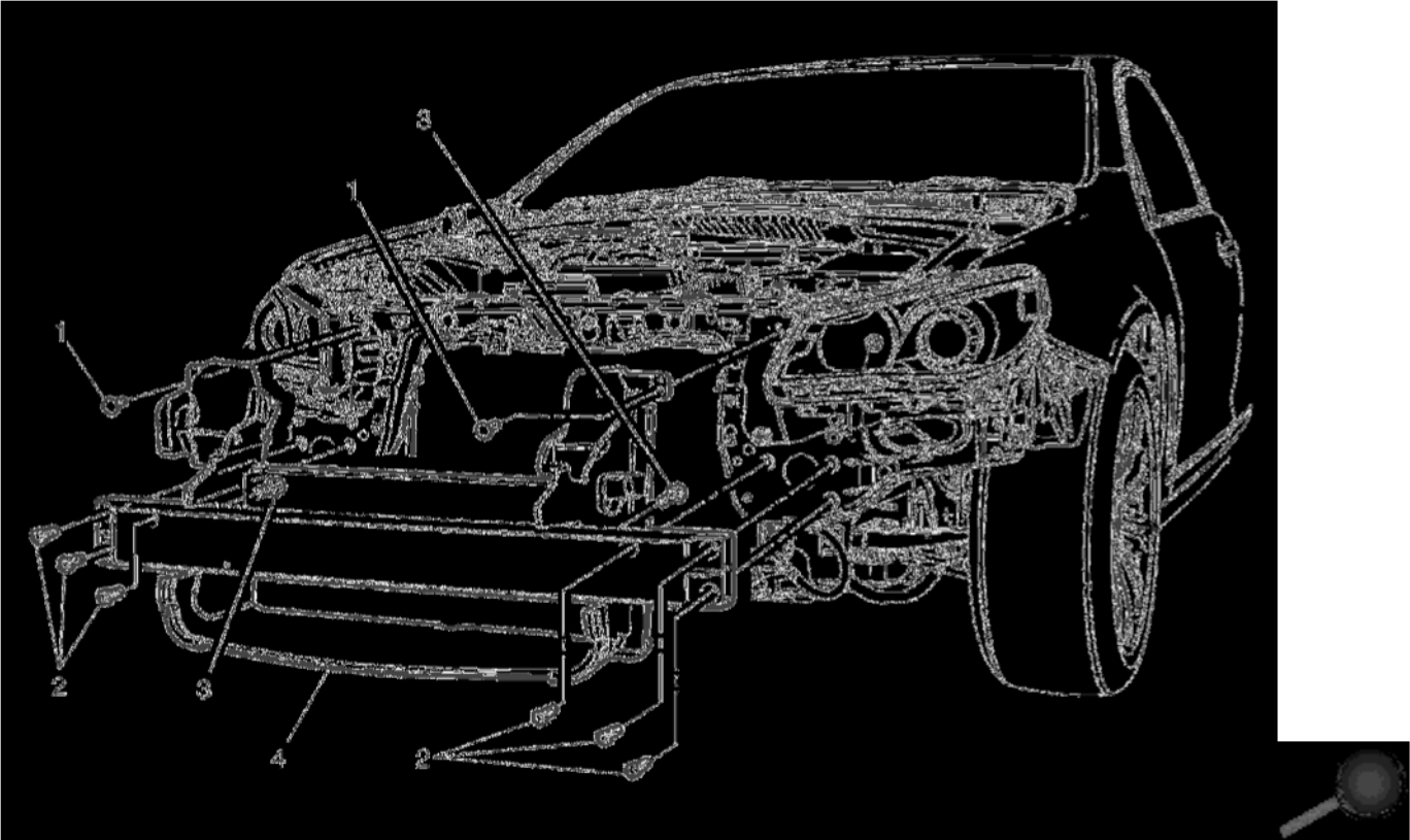
Front Bumper Impact Bar Replacement
