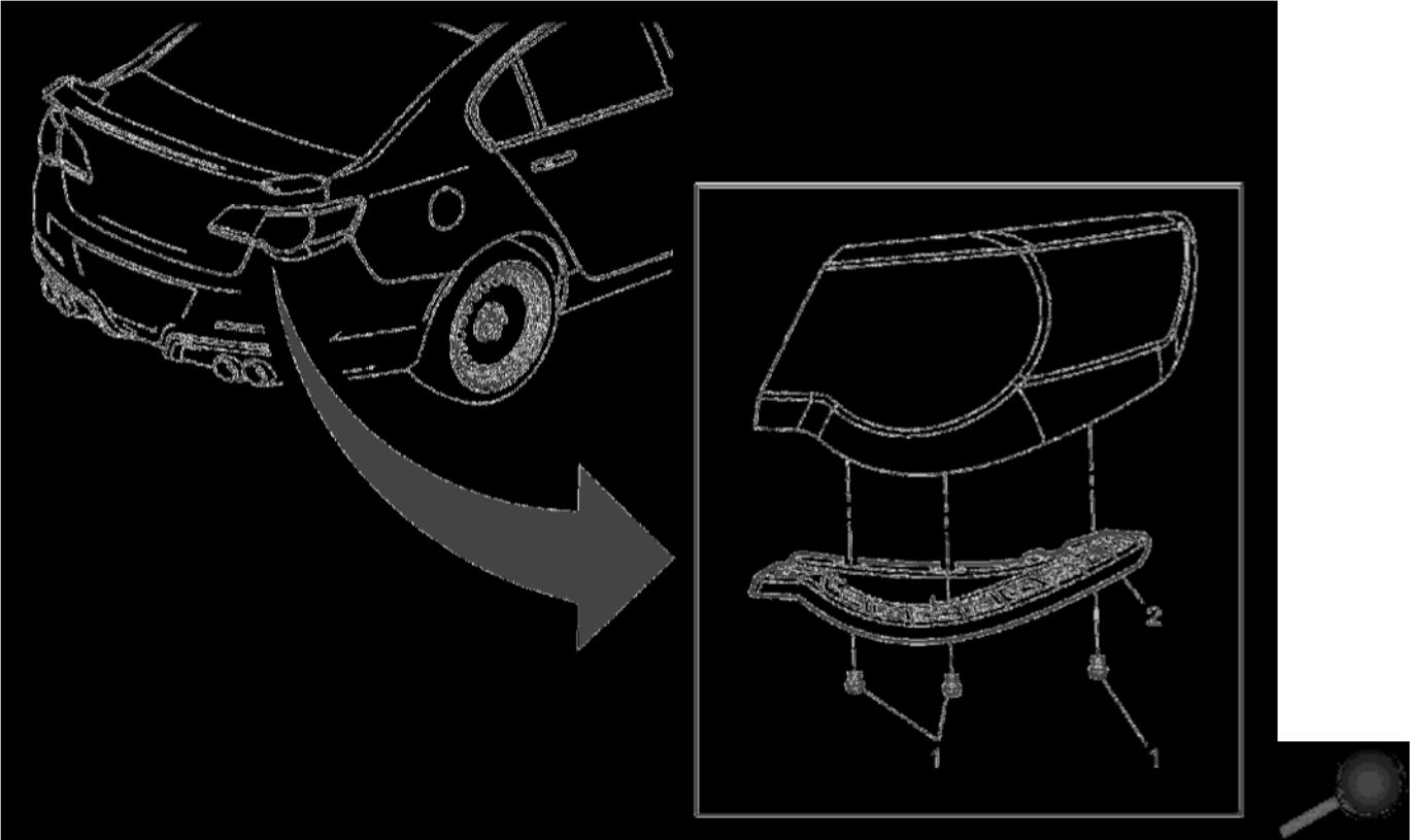
Rear Bumper Fascia Support Replacement
