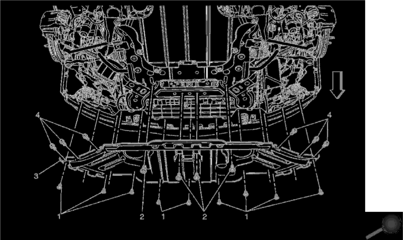
Front Bumper Fascia Extension Replacement
