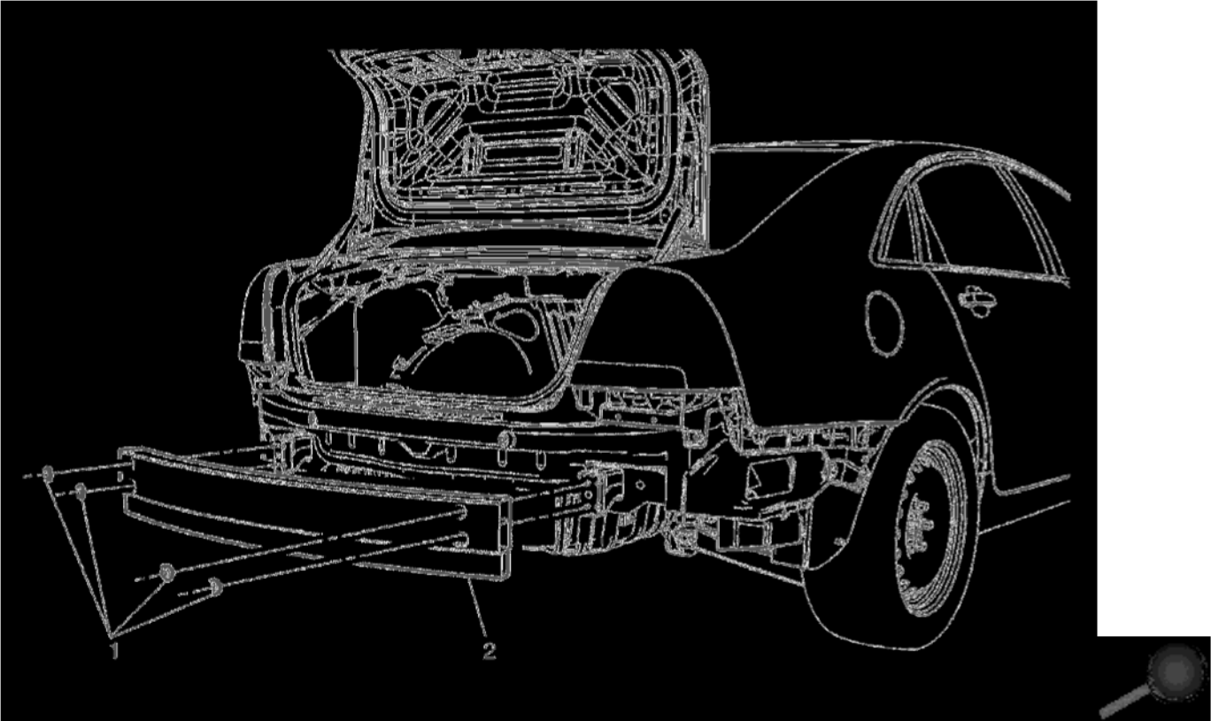
Rear Bumper Impact Bar Replacement
