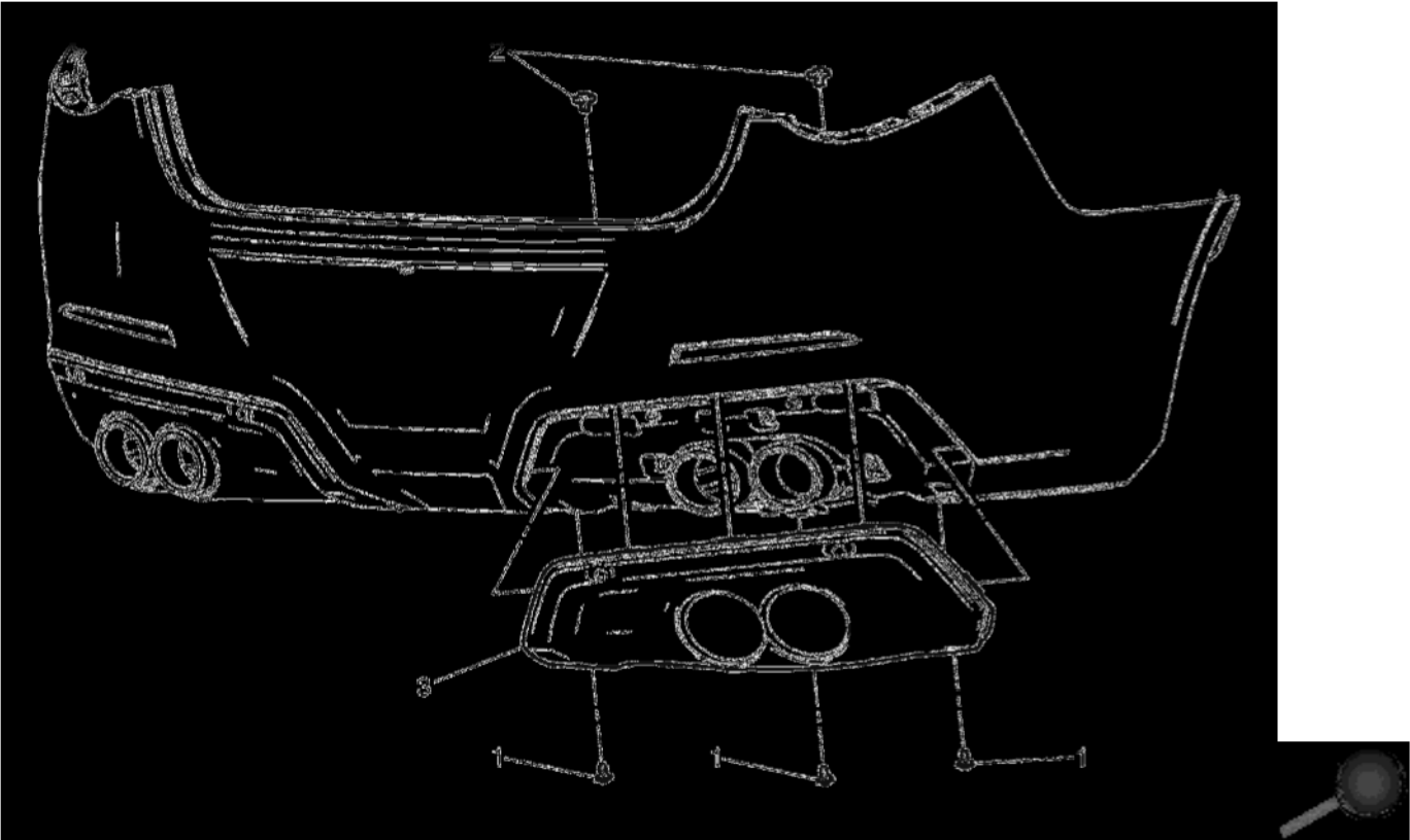
Rear Bumper Fascia Insert Replacement
