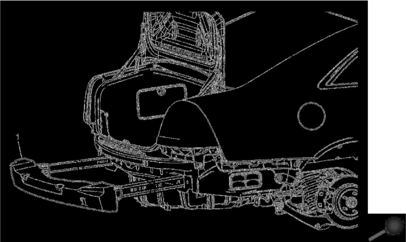
Rear Bumper Fascia Energy Absorber Replacement
