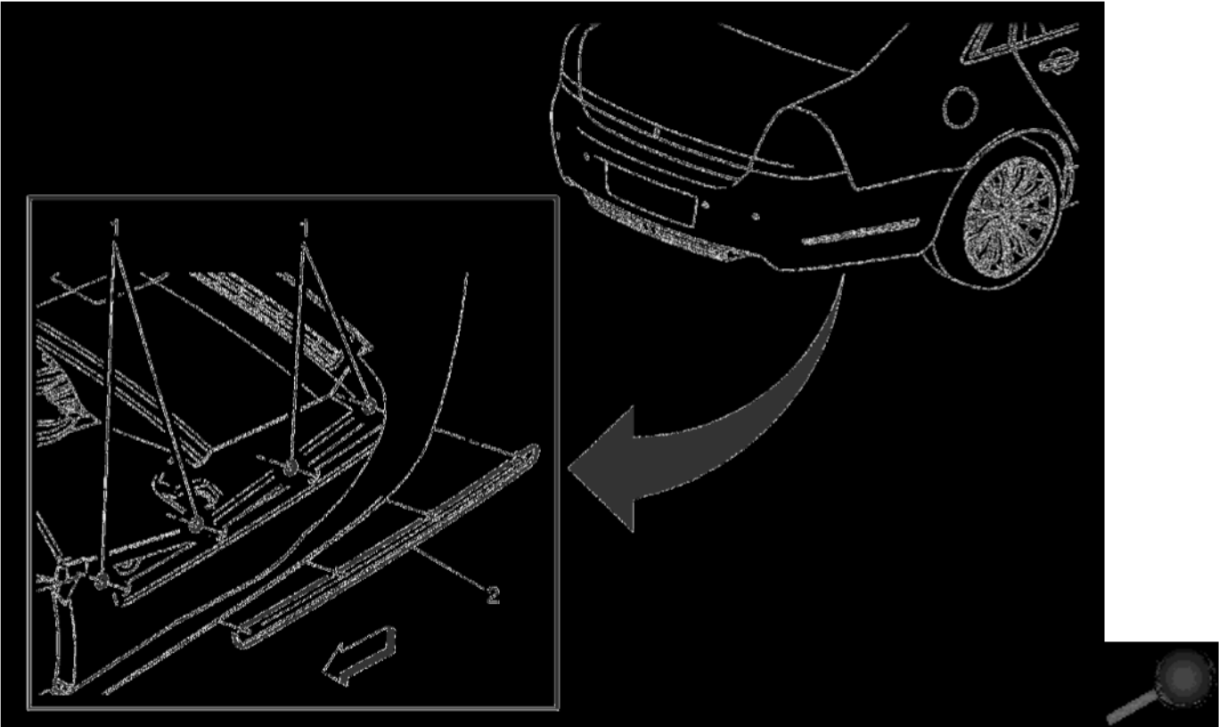
Rear Bumper Fascia Molding Replacement
