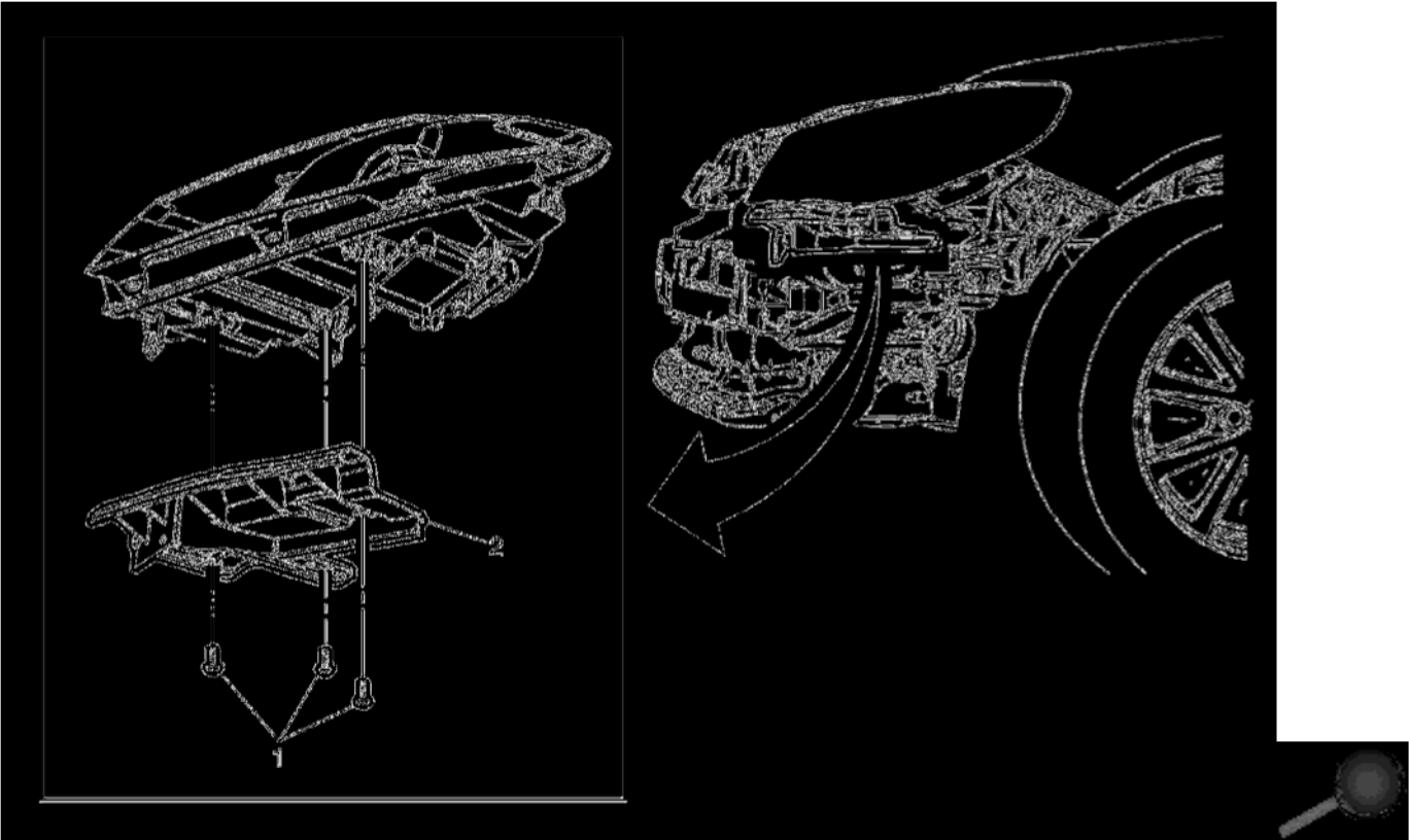
Front Bumper Fascia Reinforcement Replacement
