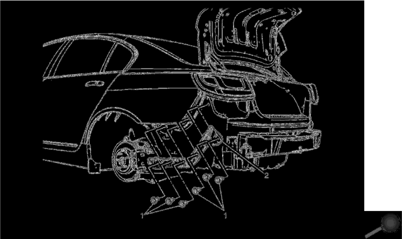
Rear Bumper Fascia Guide Replacement
