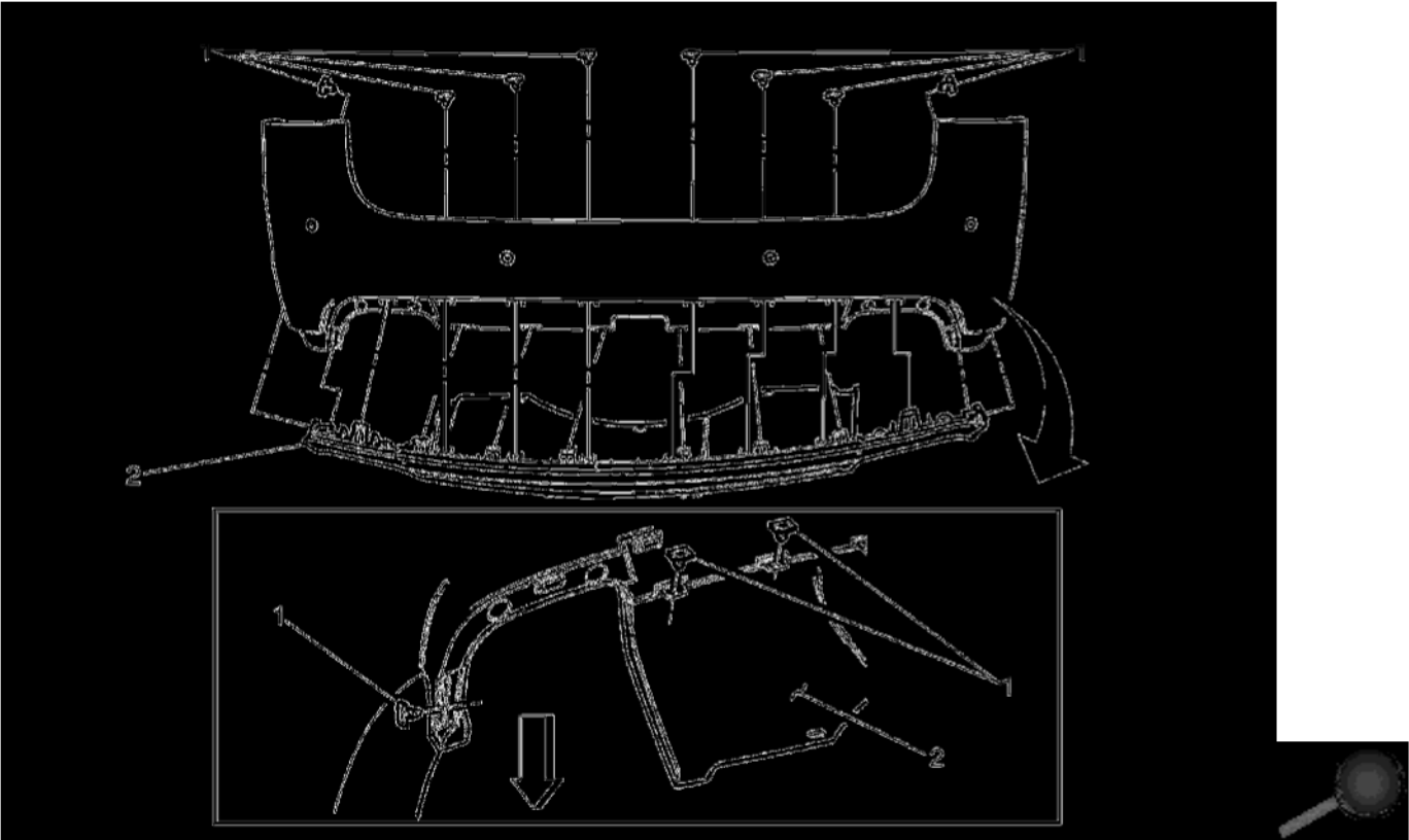
Rear Bumper Fascia Extension Replacement
