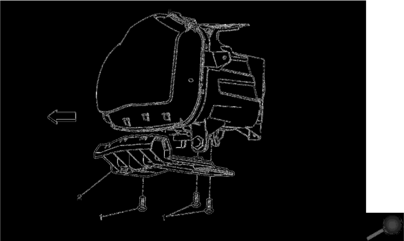
Front Bumper Fascia Support Bracket Replacement
