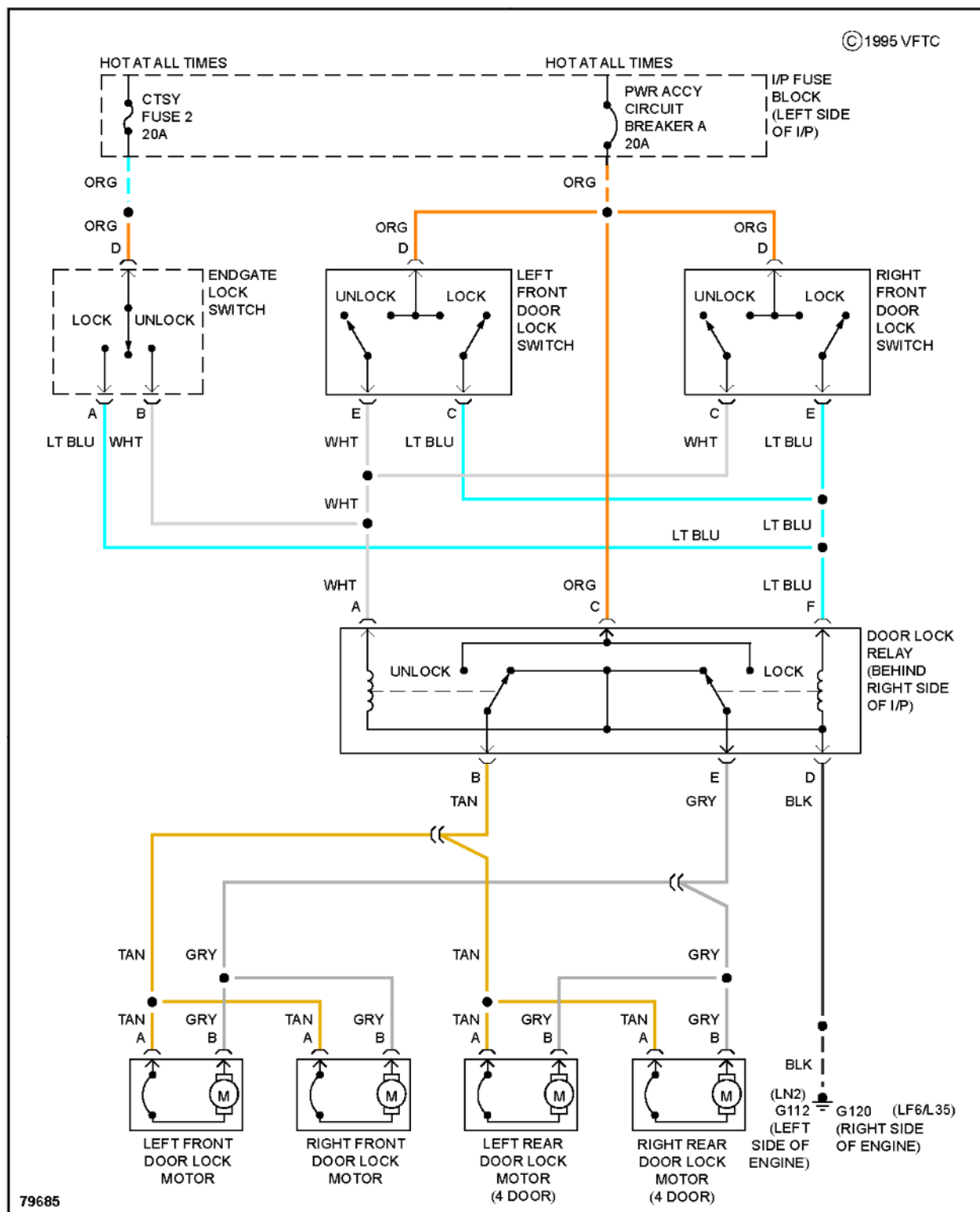
Fig. 23: Door Lock Circuit
