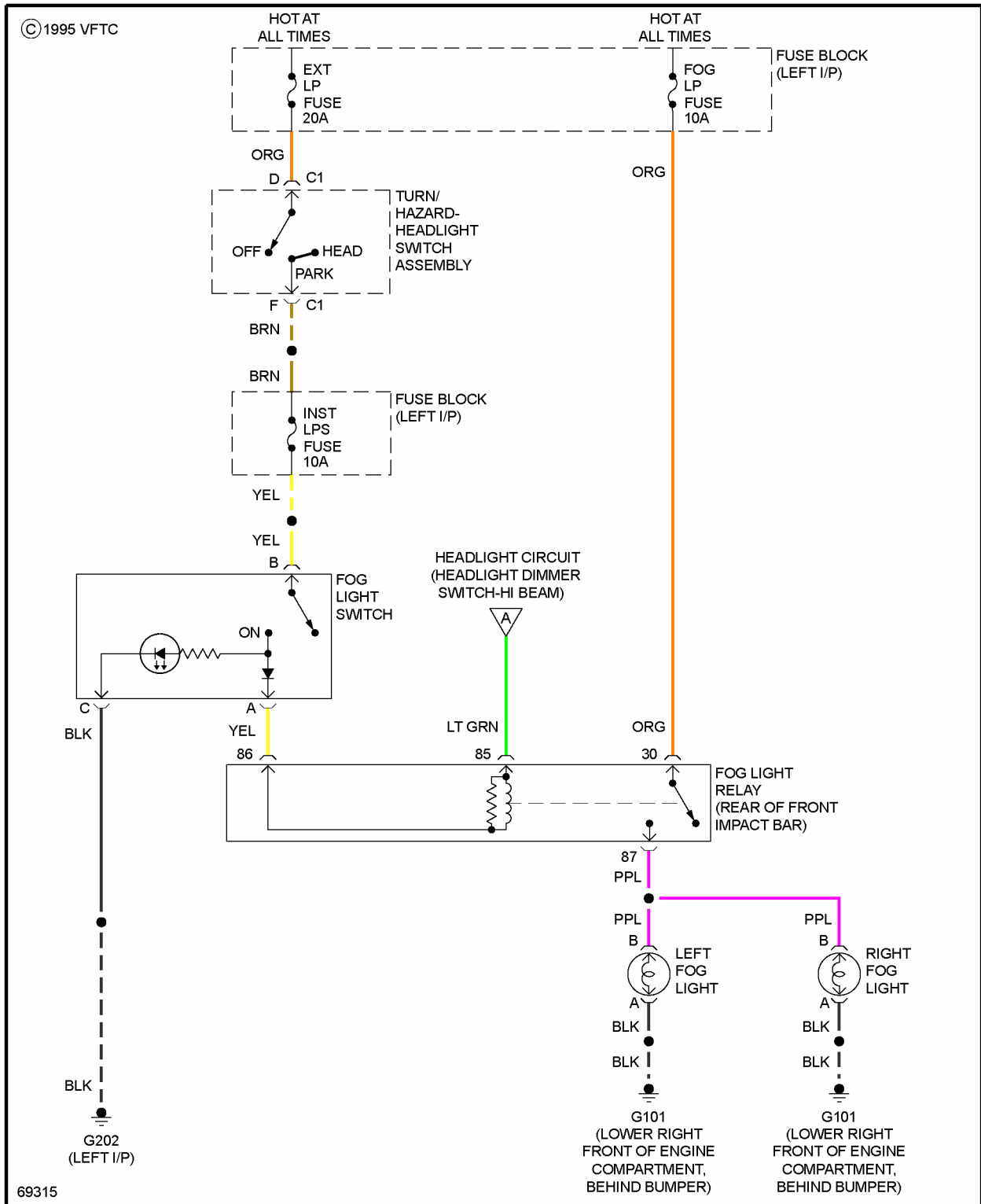
Fig. 23: Fog Lamps Circuit, W/O DRL
