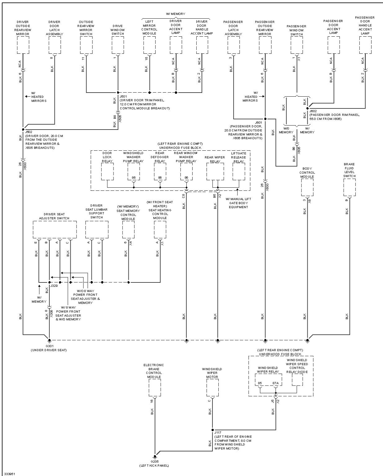
Fig. 34: Ground Distribution Circuit (3 of 4)
