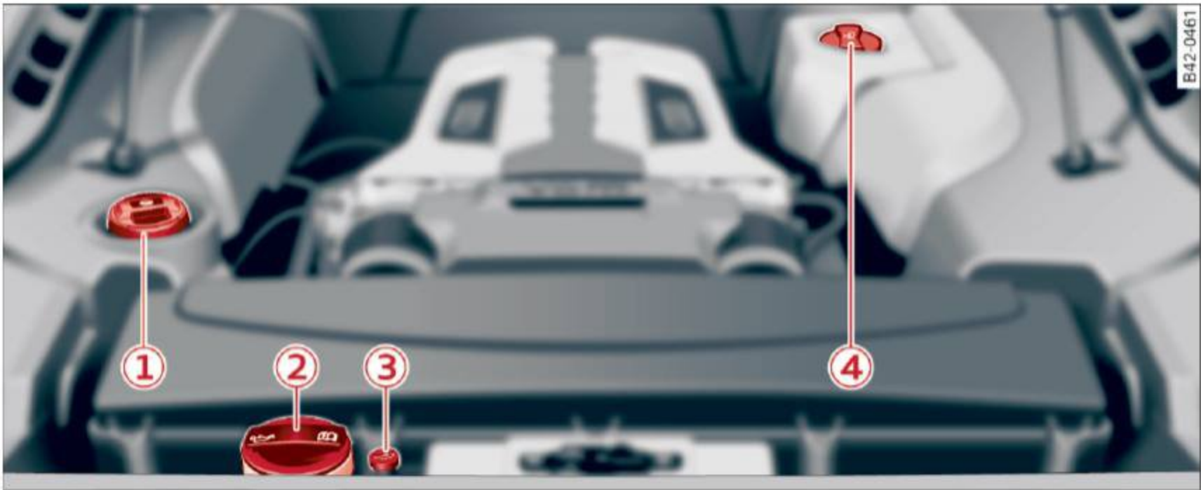
Fig. 112 Typical layout for containers, engine oil dipstick and engine oil filler cap (manual transmission)
