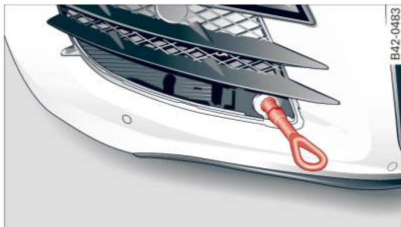
Fig. 140 Right front bumper without grille: Towing loop fully screwed in
