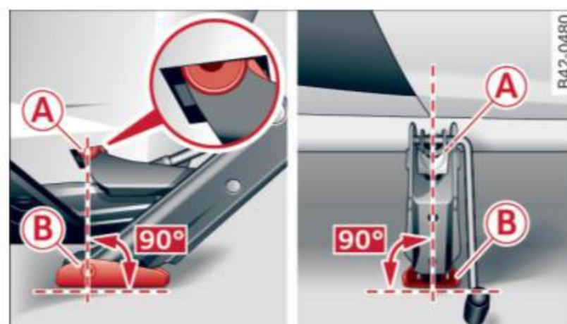
Fig. 135 Sill: positioning the vehicle jack
