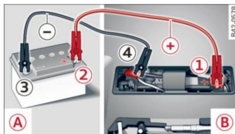
Fig. 139 Jump start using the battery in another vehicle: A - Female socket, B - Discharge
