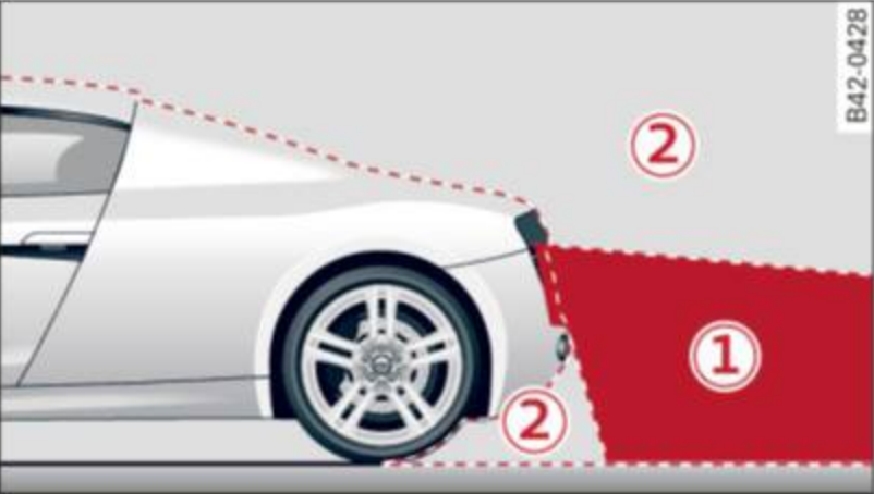
Fig. 70 Side view: Rearview camera coverage area
