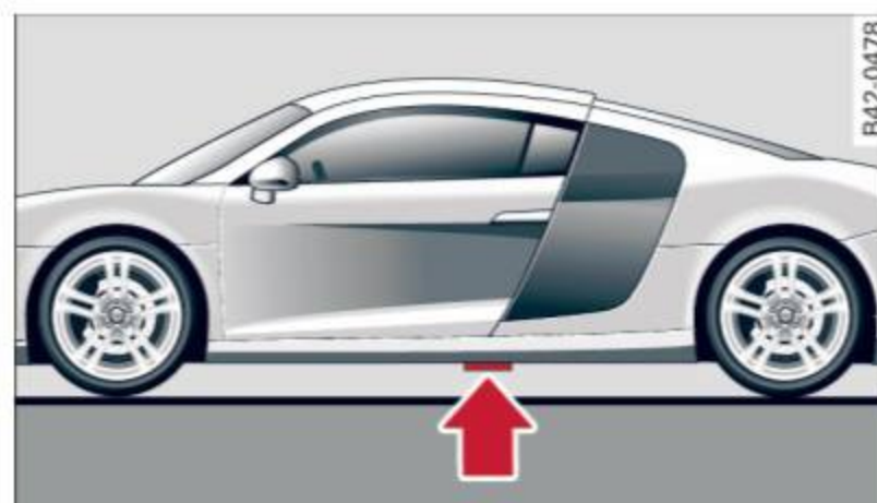
Fig. 134 Sill panels: markings
