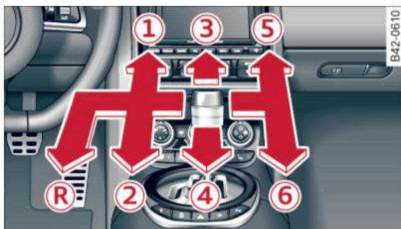
Fig. 61 Gearshift pattern: 6-speed manual transmission
