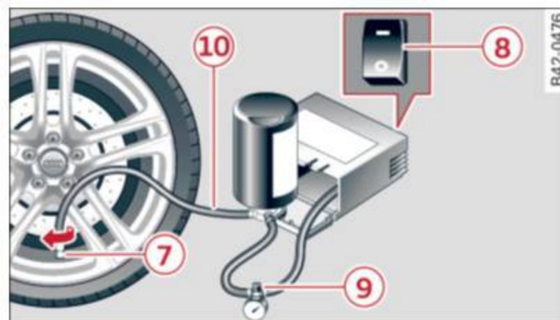
Fig. 132 Connector for the Tire Mobility System
