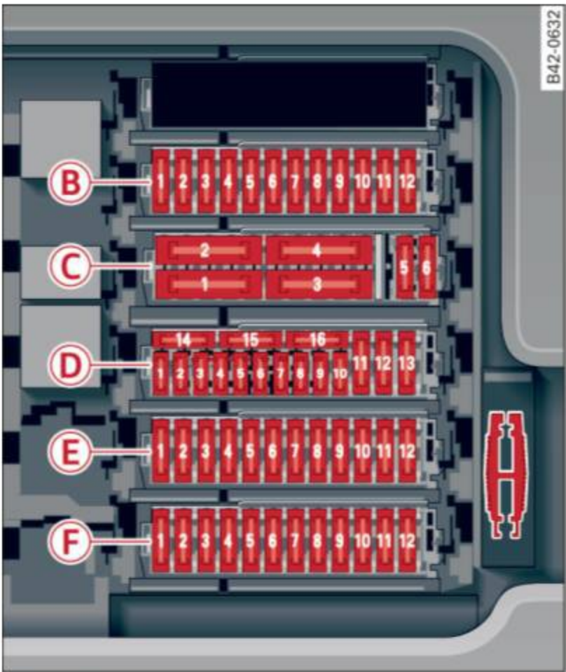
Fig. 142 Passenger footwell: Fuse panel
