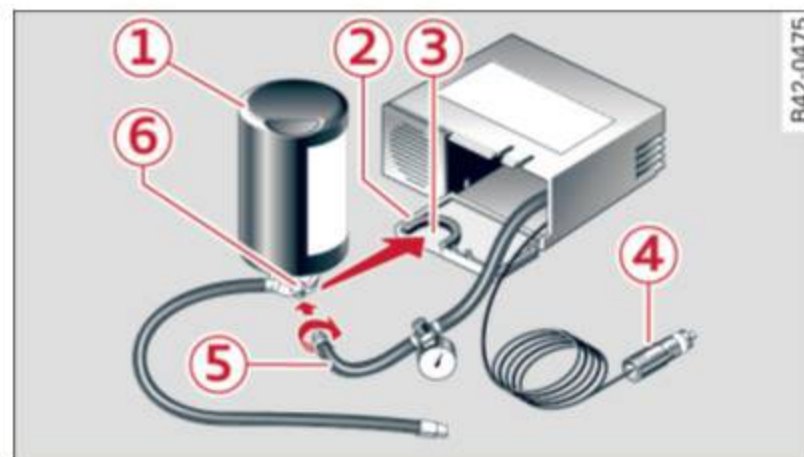
Fig. 131 Parts of the Tire Mobility System
