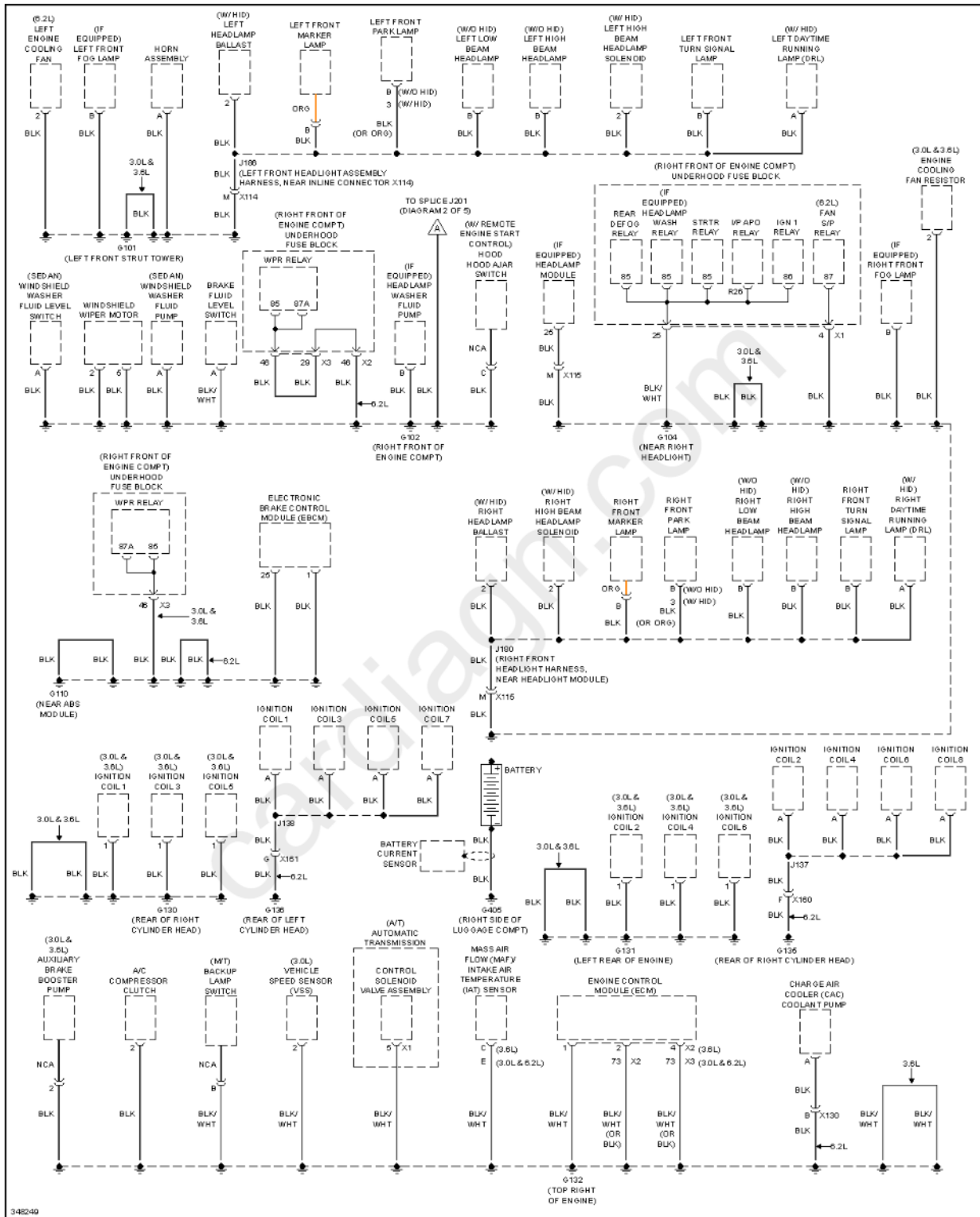
Fig. 45: Ground Distribution Circuit (1 of 5)
