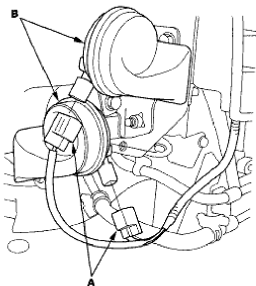
Fig. 3: Identifying Horn 1P Connector
