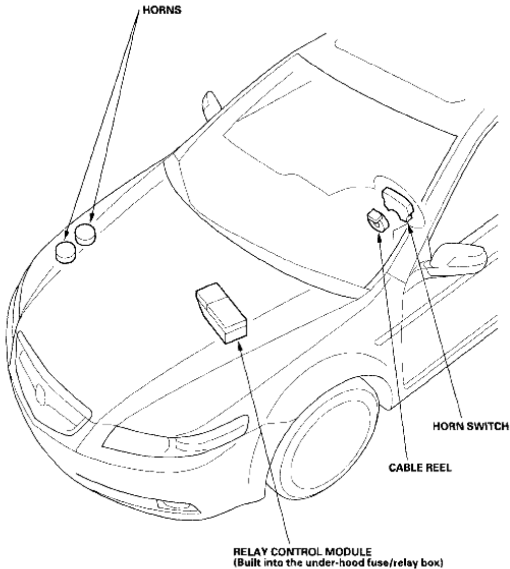
Fig. 1: Identifying Horns Components Location Courtesy of AMERICAN HONDA MOTOR CO., INC.
