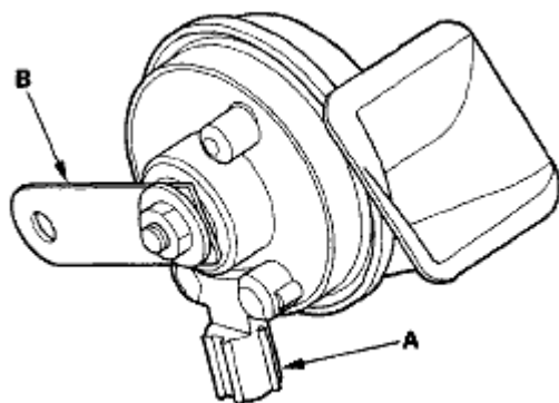
Fig. 4: Identifying Horn Battery Power Connecting Terminal And Grounding Bracket
