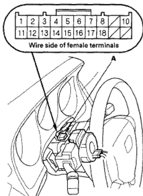
Fig. 5: Identifying Dashboard Wire Harness 20P Connector Courtesy of AMERICAN HONDA MOTOR CO., INC.
