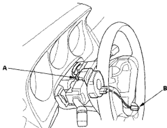
Fig. 6: Identifying Dashboard Wire Harness 20P Connector Courtesy of AMERICAN HONDA MOTOR CO., INC.
