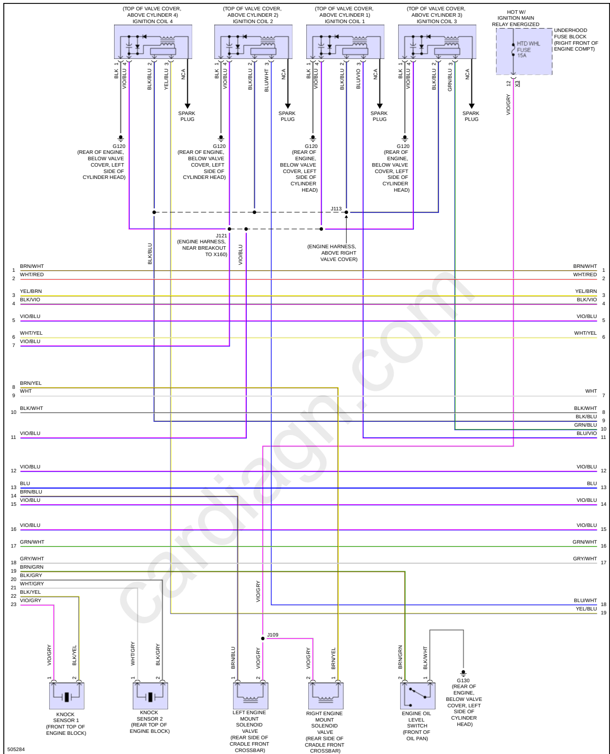
Fig 5: 2.0L VIN X, Engine Performance Circuit (5 of 7)
