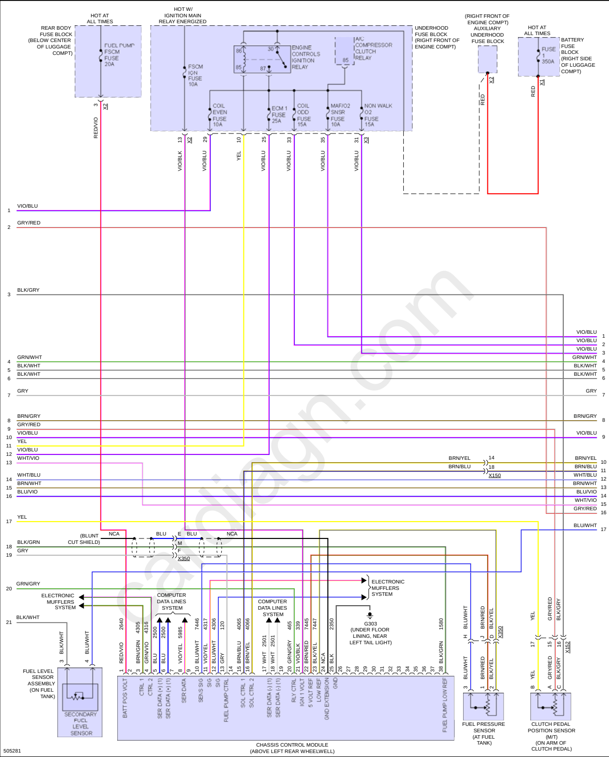
Fig 2: 2.0L VIN X, Engine Performance Circuit (2 of 7)
