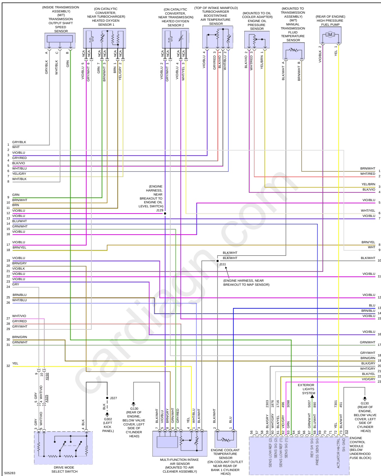
Fig 4: 2.0L VIN X, Engine Performance Circuit (4 of 7)
