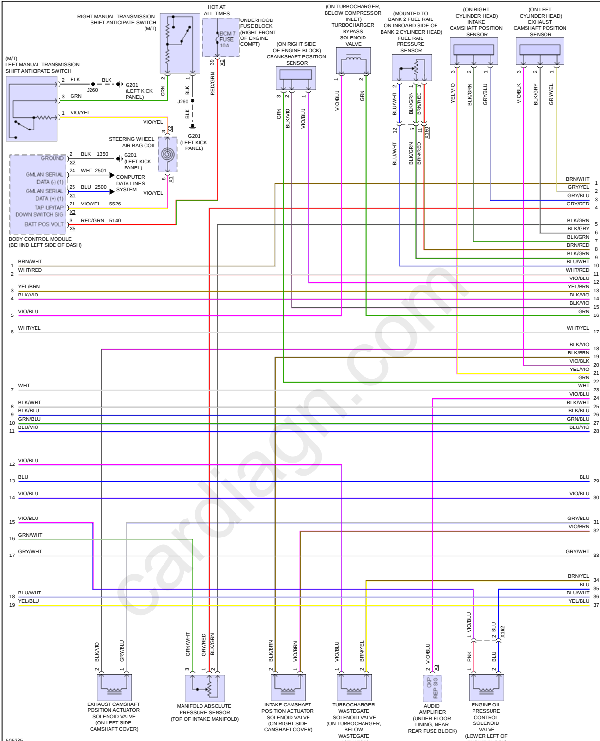
Fig 6: 2.0L VIN X, Engine Performance Circuit (6 of 7)
