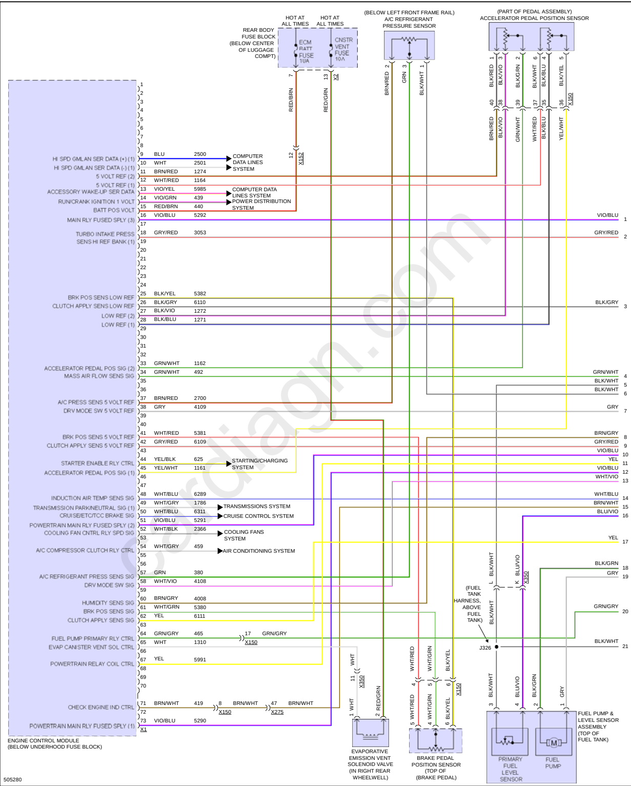
Fig 1: 2.0L VIN X, Engine Performance Circuit (1 of 7)
