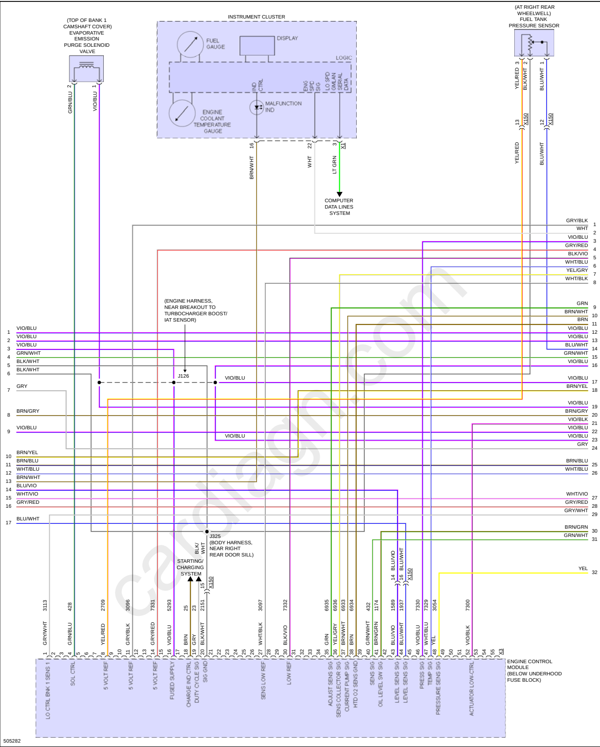
Fig 3: 2.0L VIN X, Engine Performance Circuit (3 of 7)
