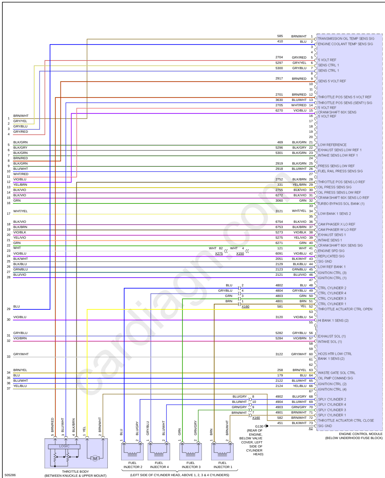
Fig 7: 2.0L VIN X, Engine Performance Circuit (7 of 7)
