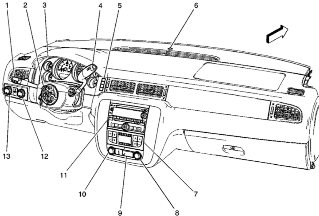
Fig. 2: Front of the I/P (Except Z75)
