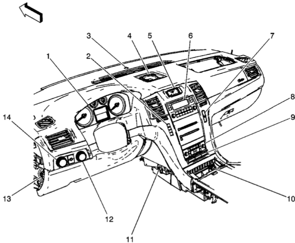
Fig. 3: Front of the I/P (Z75)
