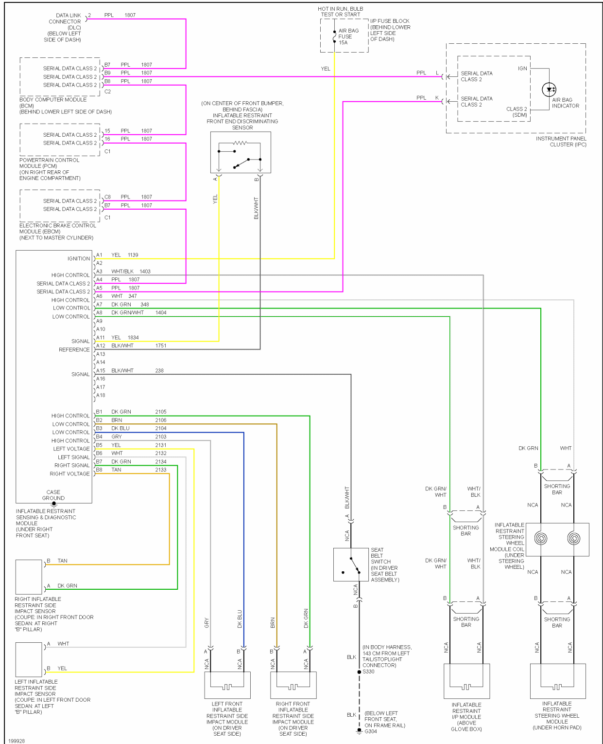
Fig. 38: Supplemental Restraints Circuit
