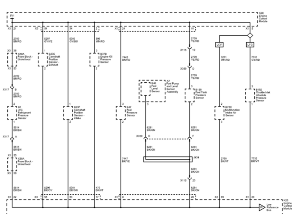
Fig. 2: 5V1 and Low Reference Bus (1 of 2) Wiring Schematics Courtesy of GENERAL MOTORS COMPANY
