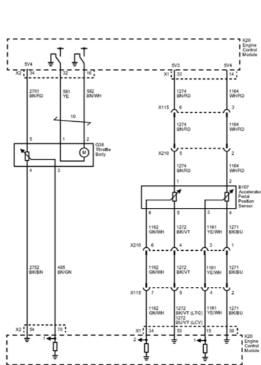
Fig. 5: Engine Data Sensors - Throttle Controls Wiring Schematics Courtesy of GENERAL MOTORS COMPANY
