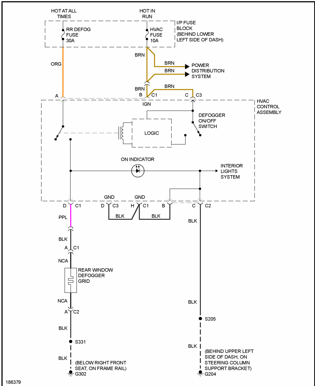
Fig. 9: Defoggers Circuit
