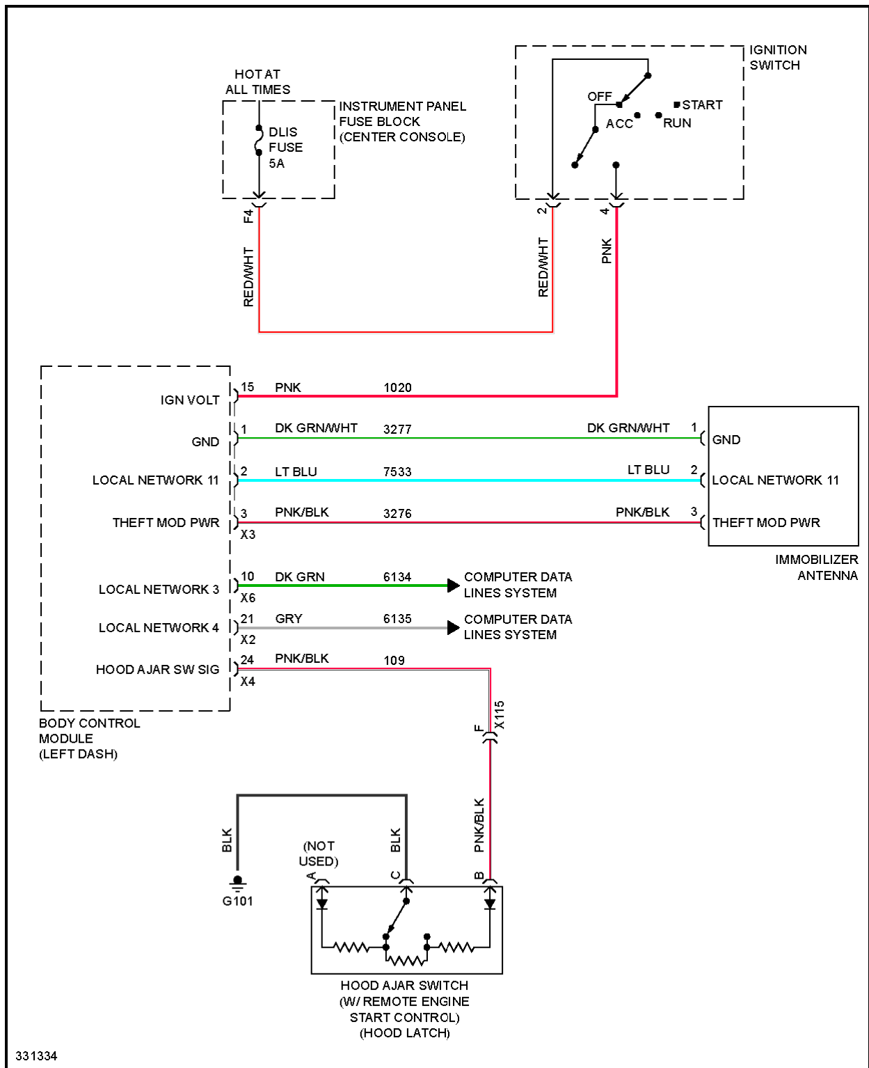
Fig. 9: Pass-Key Circuit
