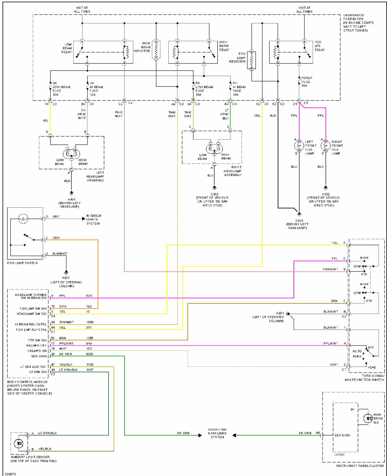
Fig. 35: Headlights Circuit
