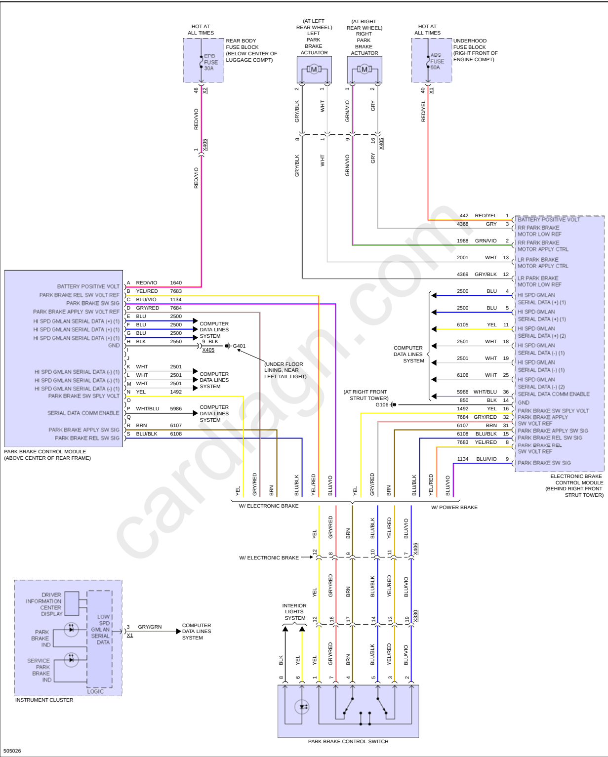
Fig 1: Park Brake System Circuit
