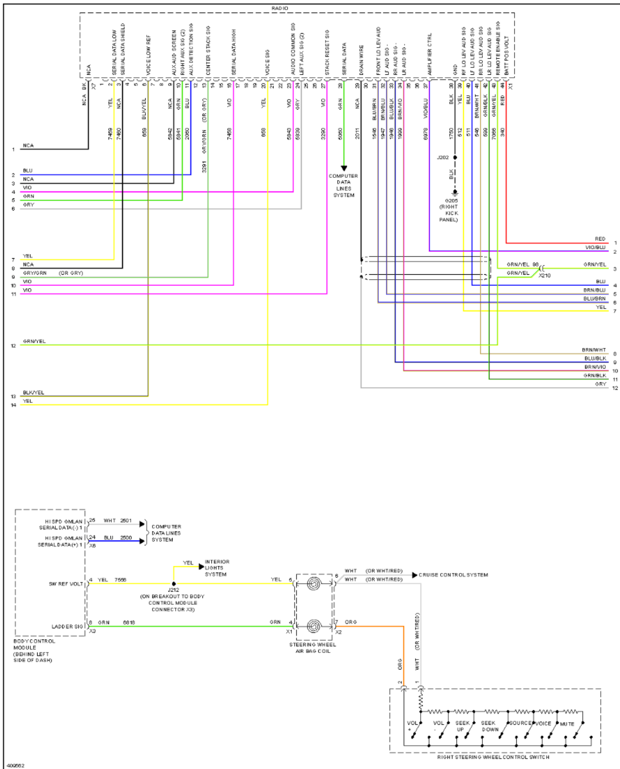
Fig. 80: Navigation Circuit, W/ Amplifier (3 of 4)
