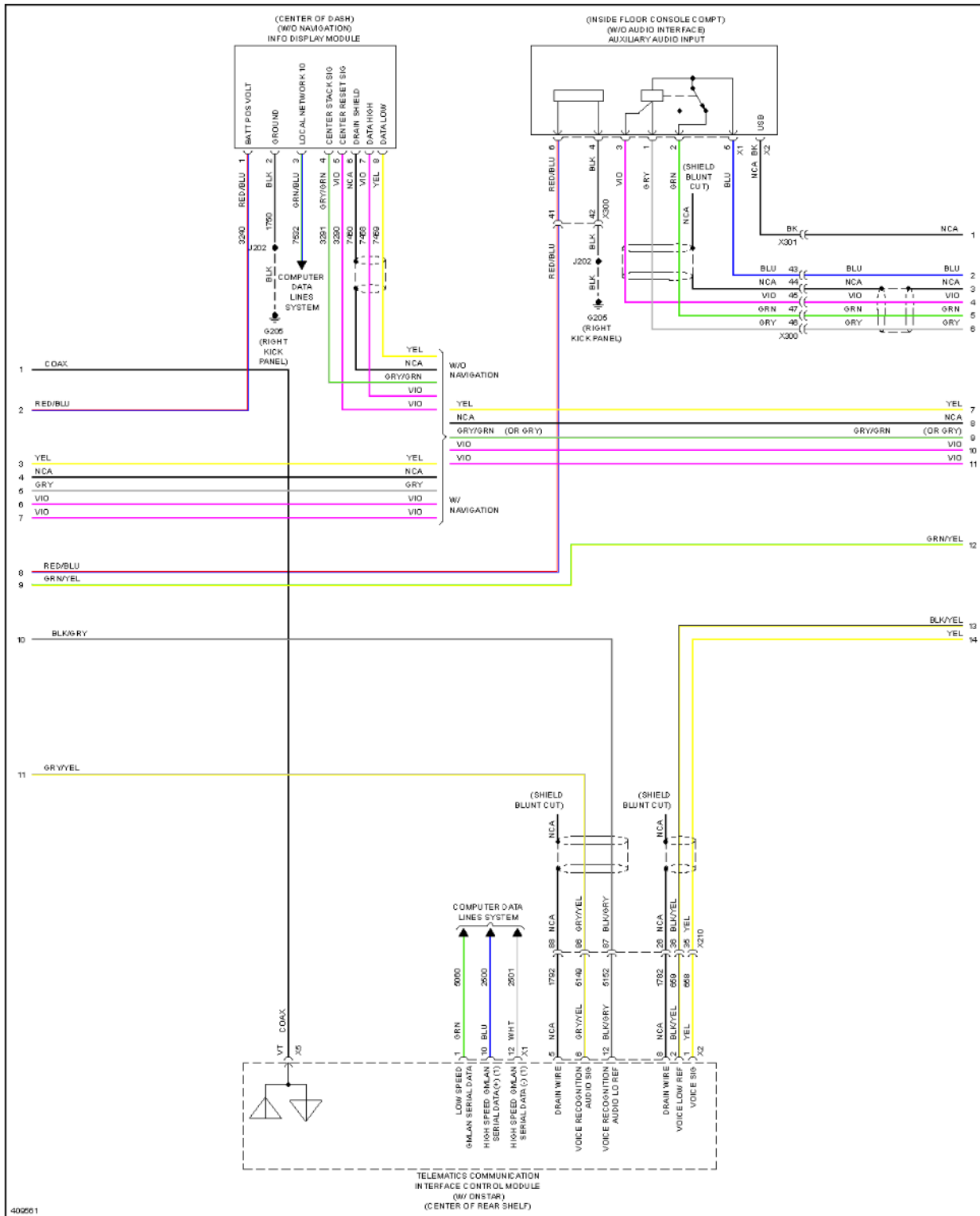
Fig. 79: Navigation Circuit, W/ Amplifier (2 of 4)
