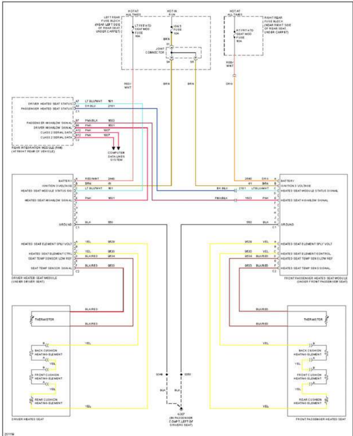
Fig. 63: Heated Seats Circuit
