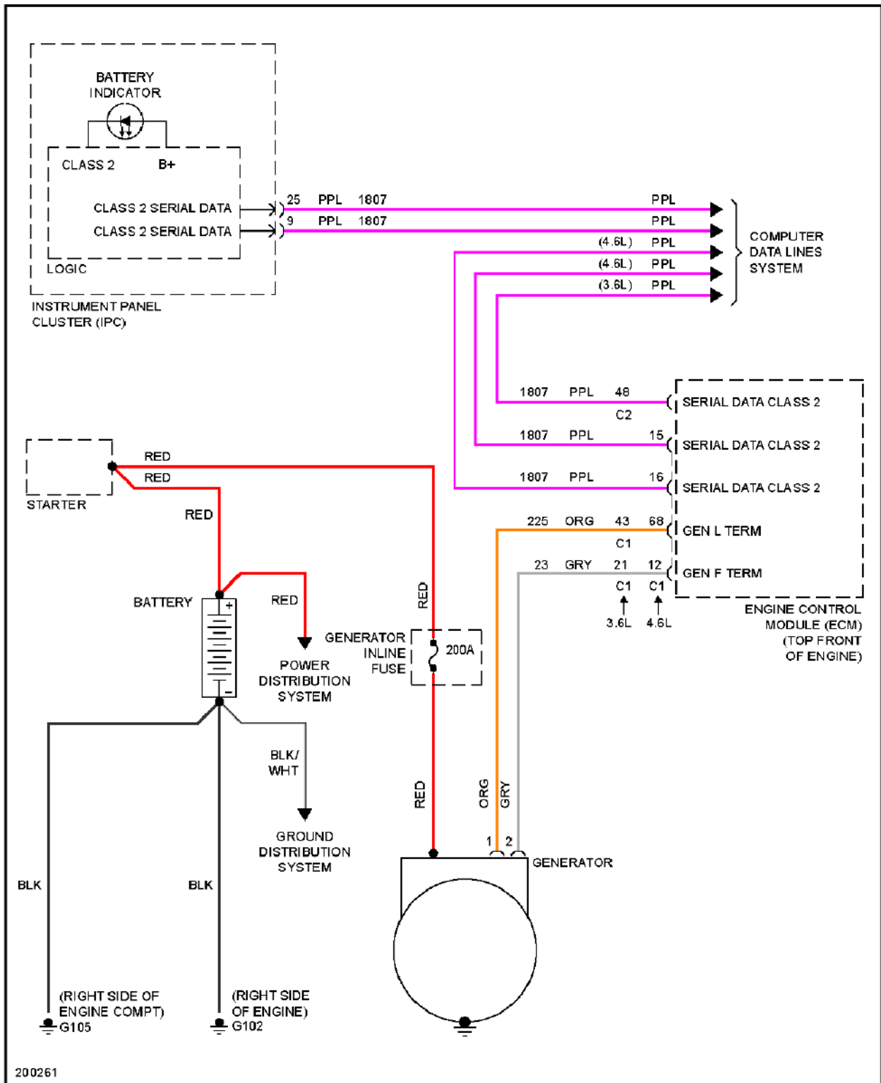
Fig. 79: Charging Circuit
