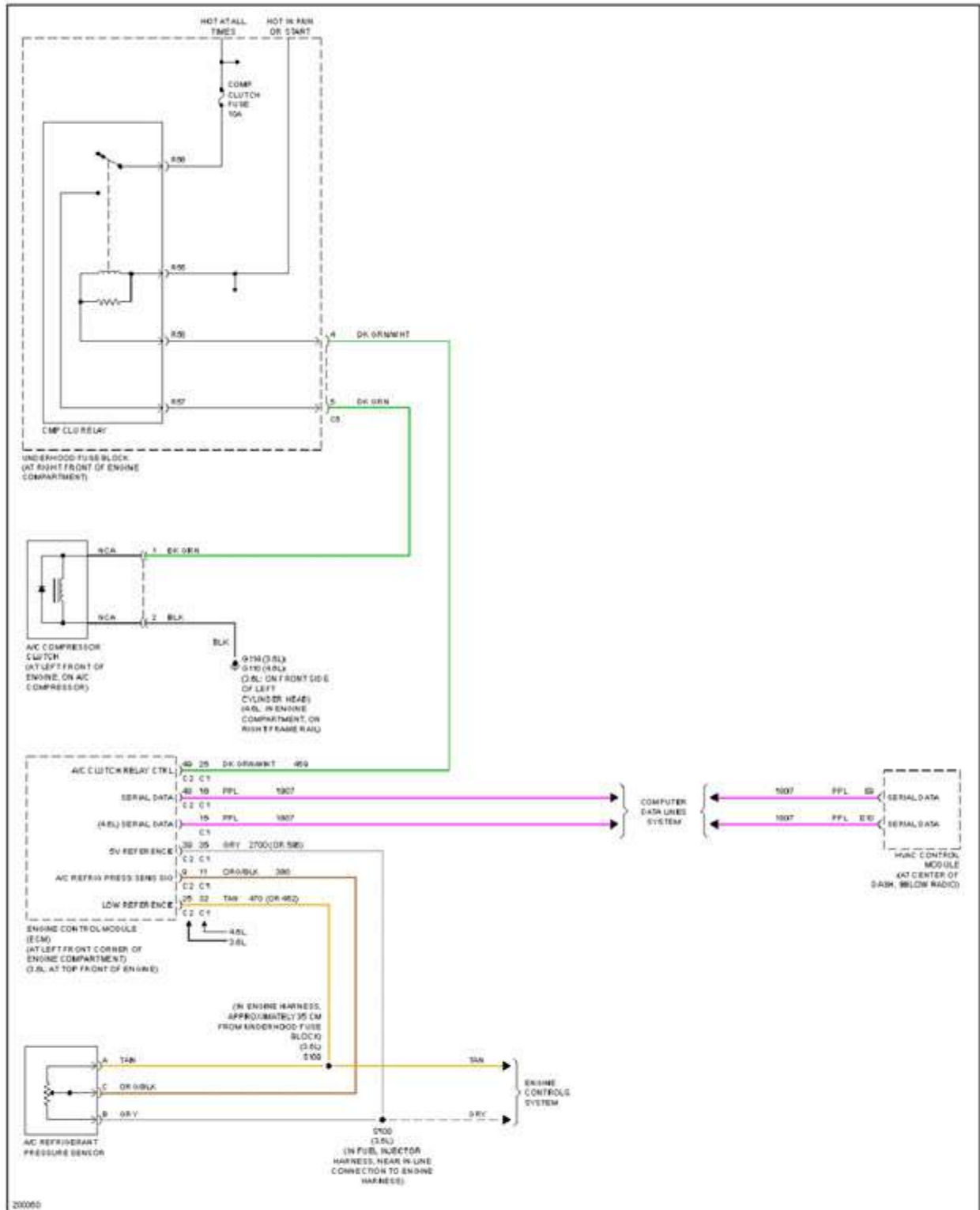
Fig. 5: Compressor Circuit
