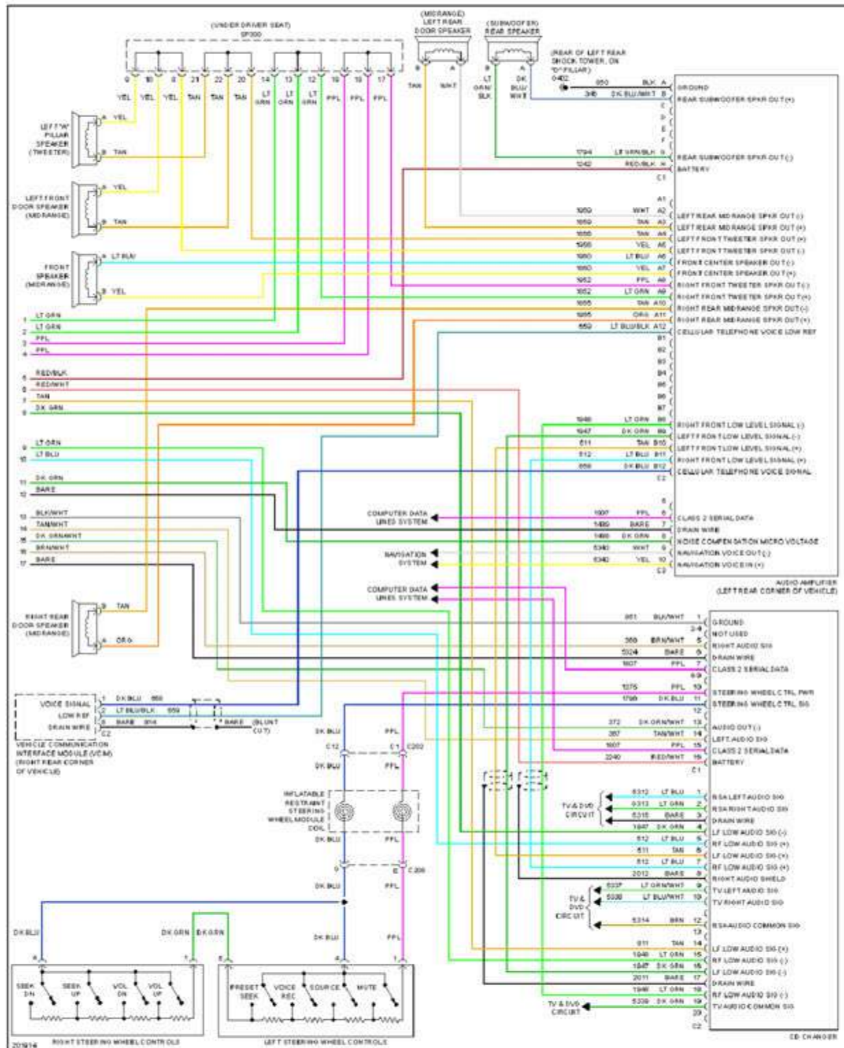
Fig. 72: Premium Sound Radio Circuit, W/ CD Changer (2 of 2)
