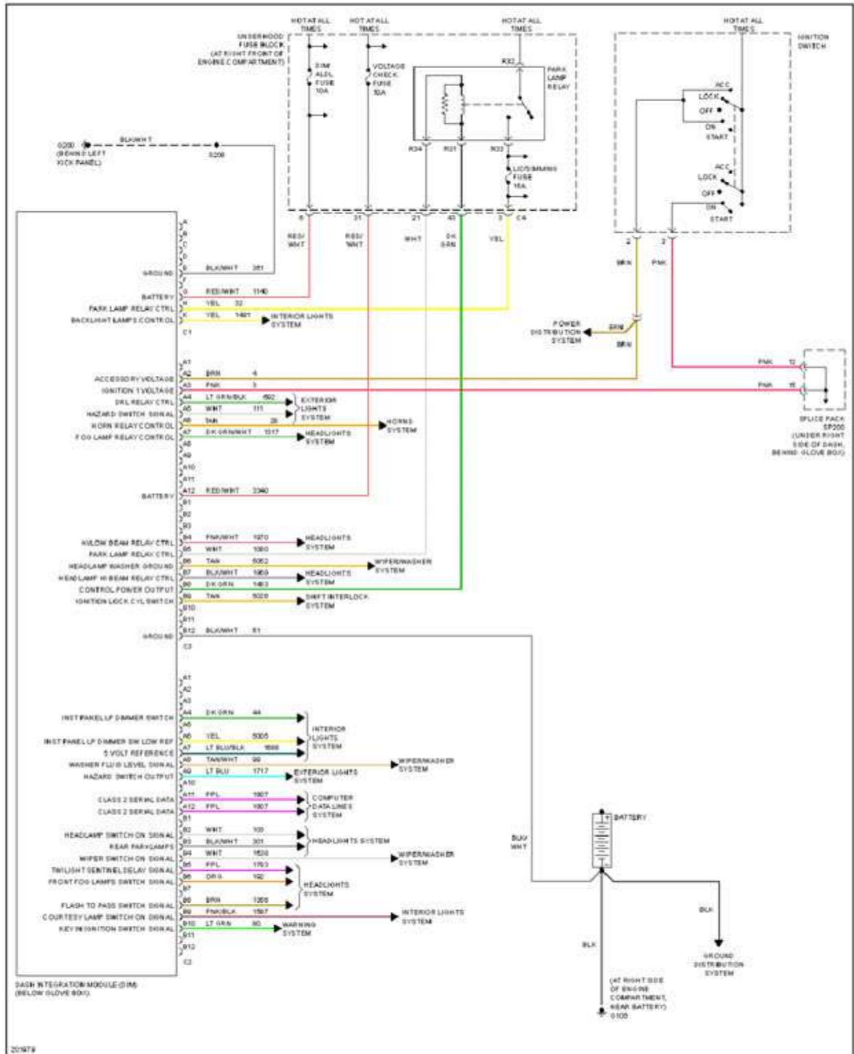
Fig. 10: Dash Integration Module Circuit
