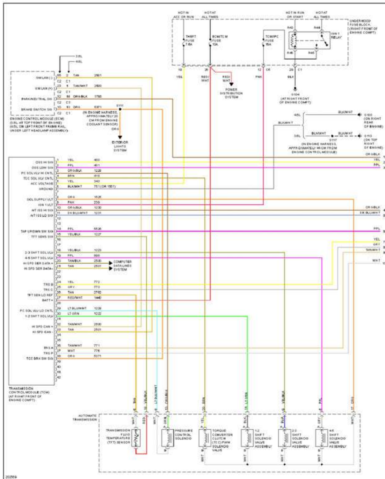
Fig. 83: Transmission Circuit (1 of 2)
