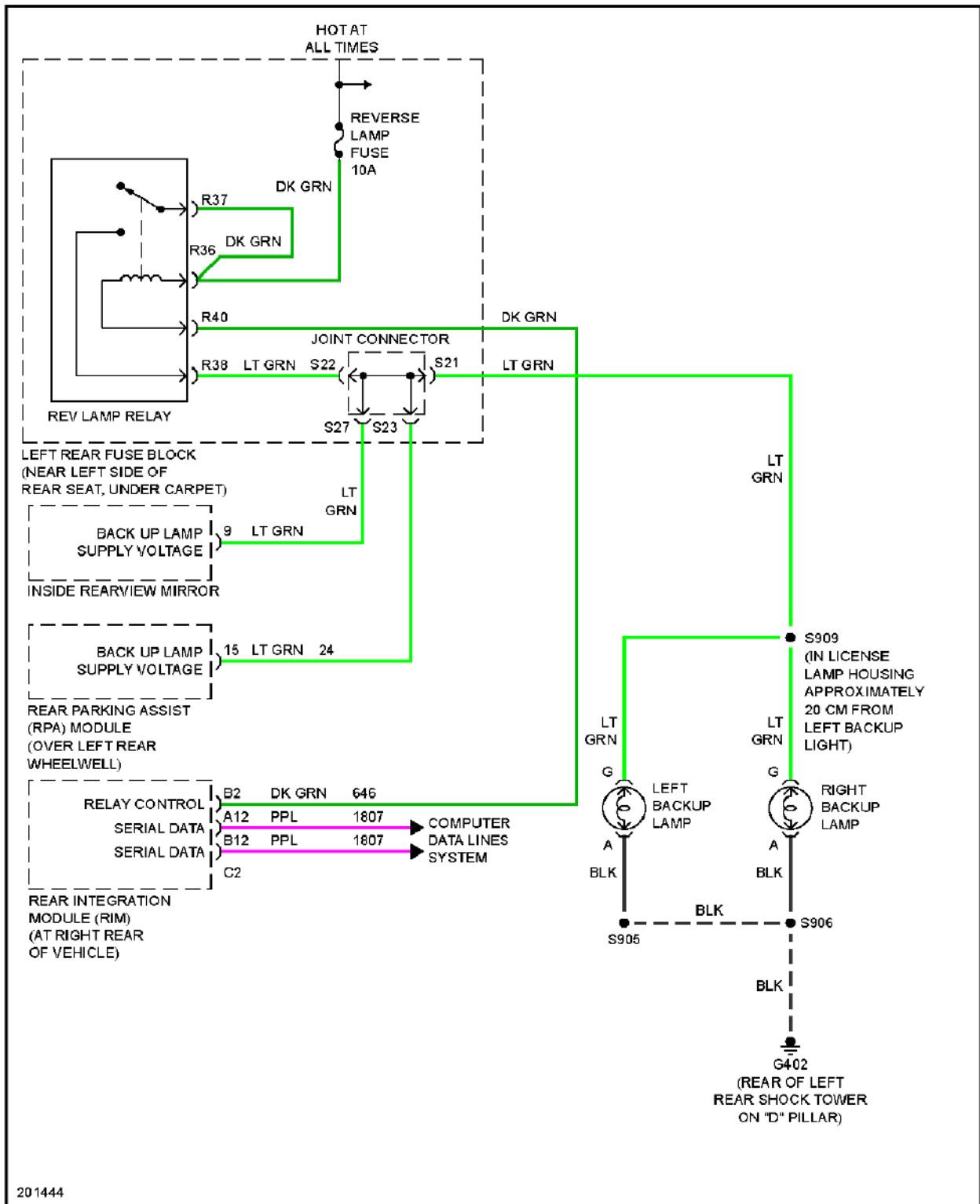
Fig. 28: Back-up Lamps Circuit
