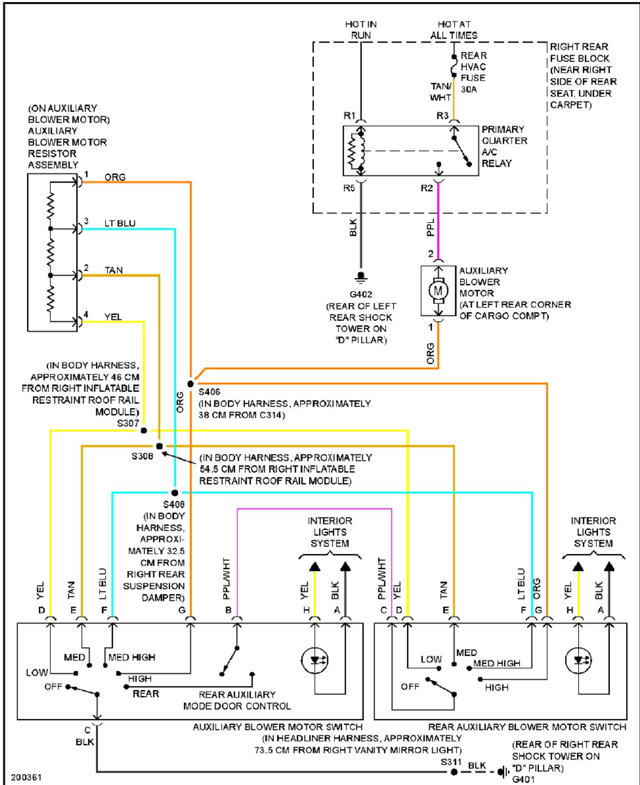
Fig. 4: Automatic A/C Circuit, Rear A/C
