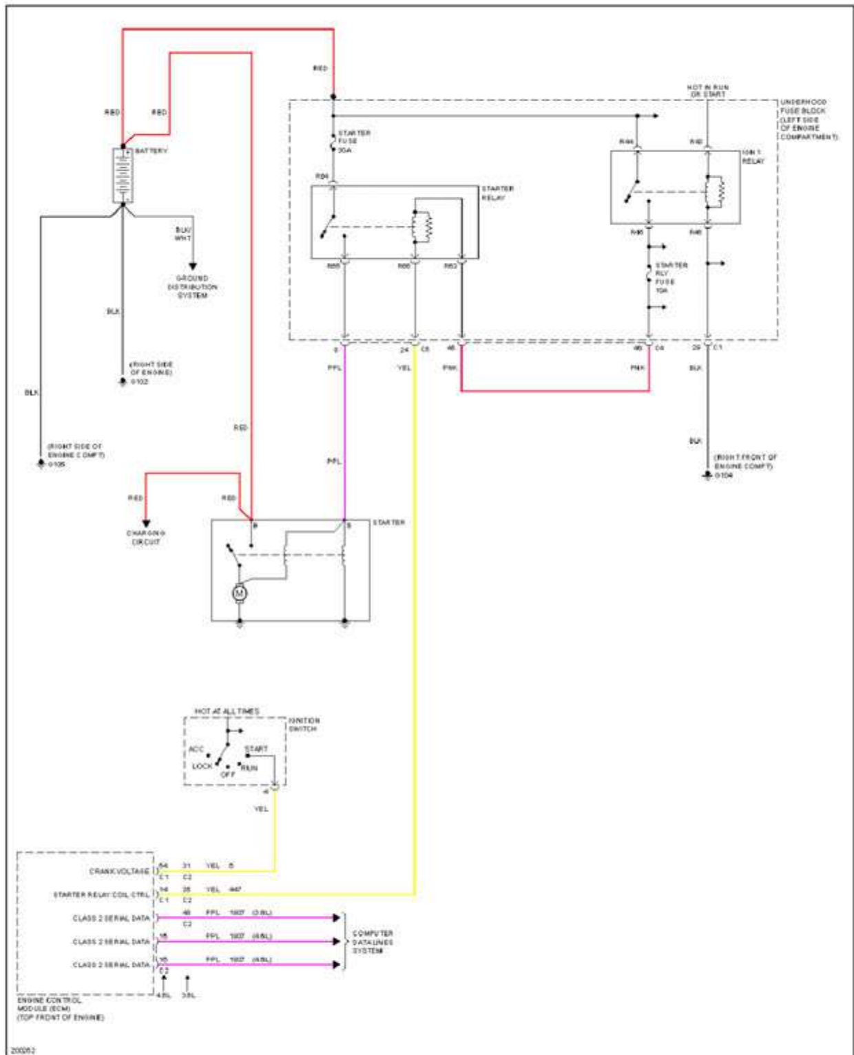
Fig. 80: Starting Circuit
