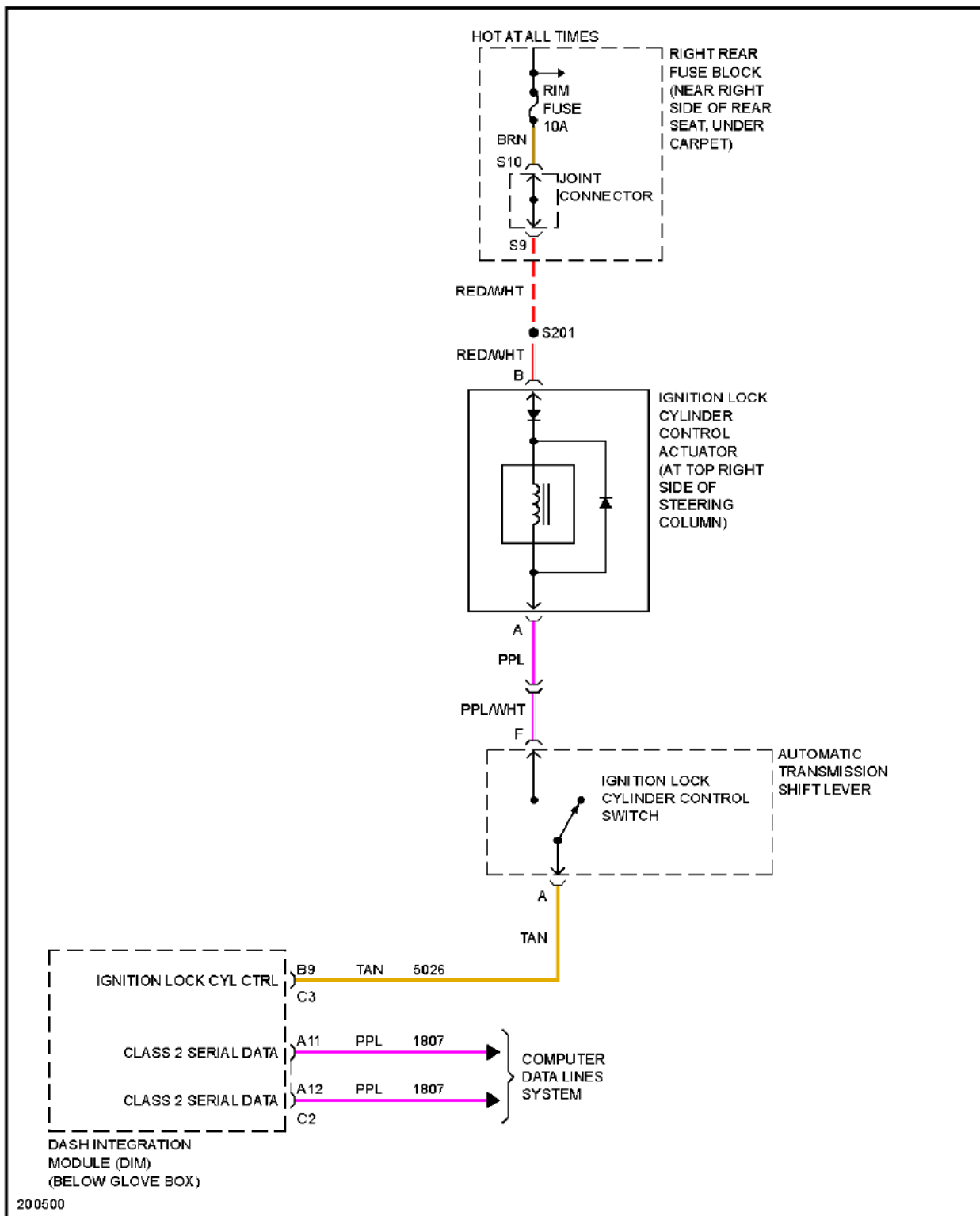
Fig. 77: Ignition Lock Solenoid Circuit
