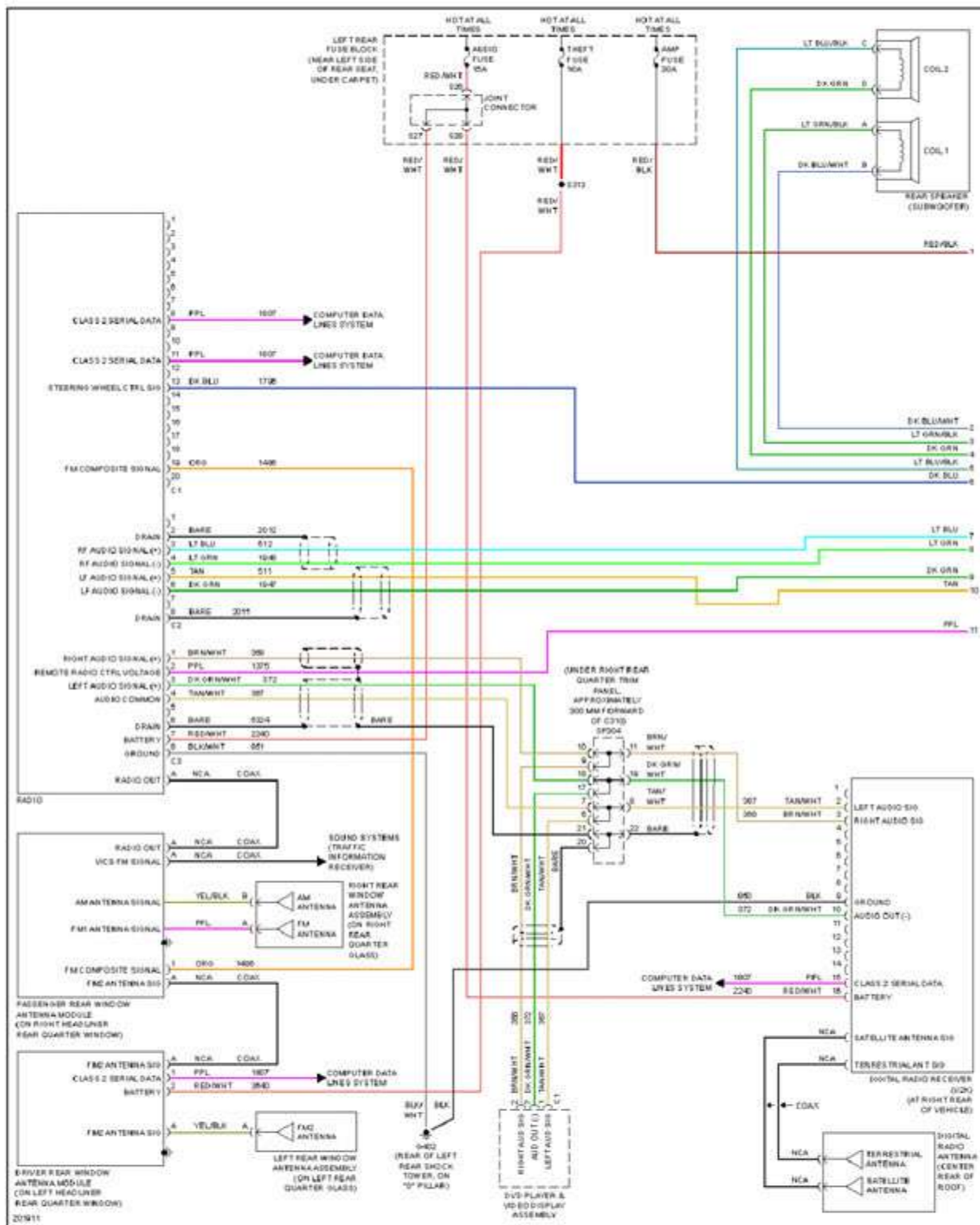
Fig. 69: Base Radio Circuit (1 of 2)
