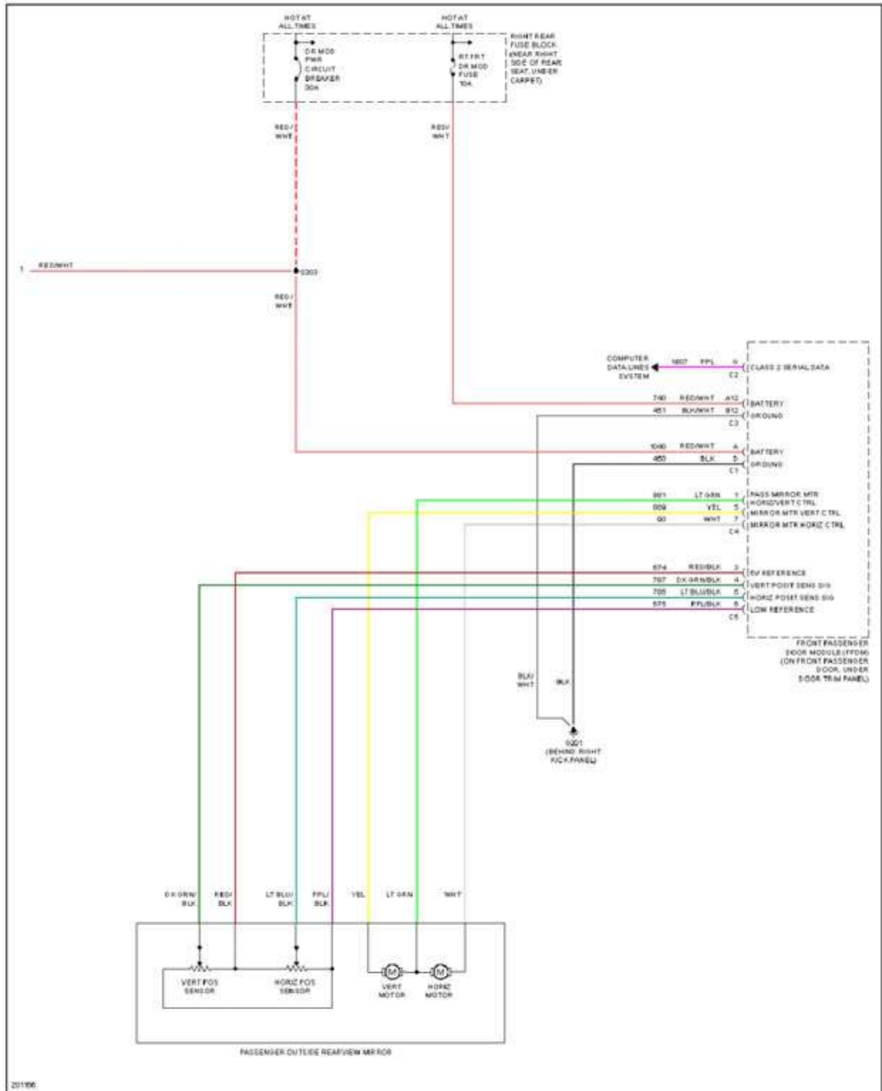
Fig. 45: Memory Mirrors Circuit (2 of 2)
