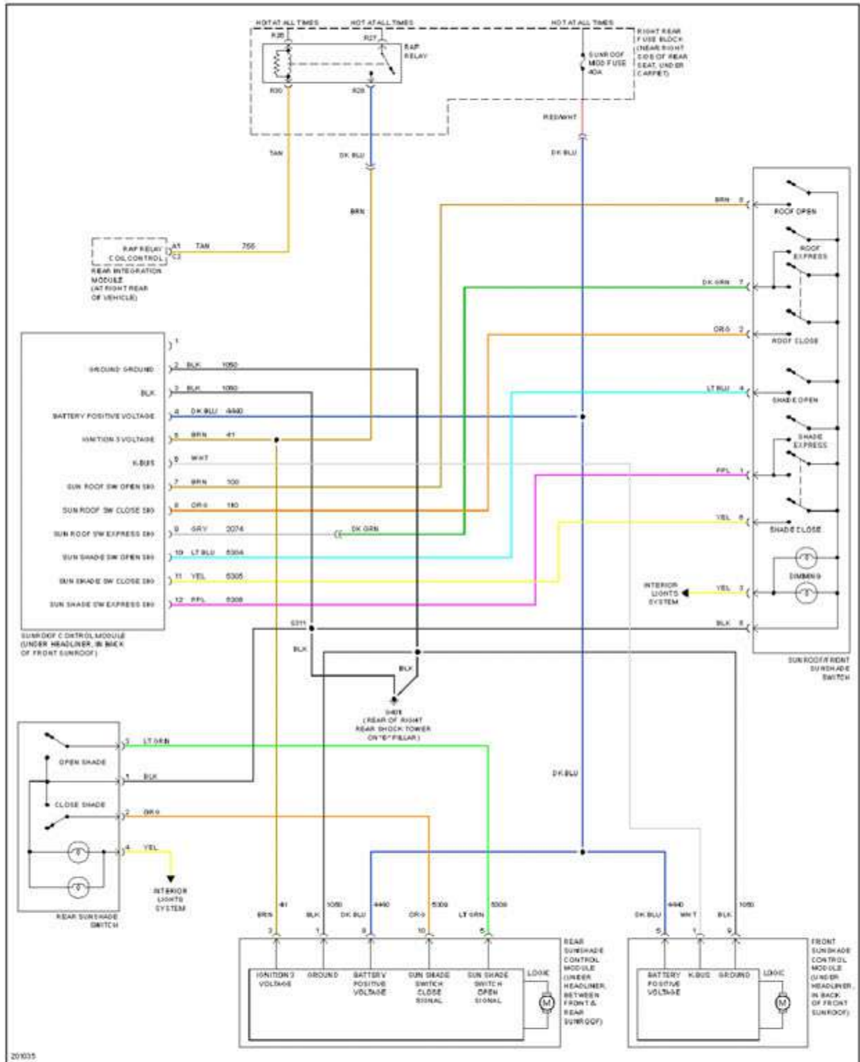
Fig. 66: Sunroof Circuit
