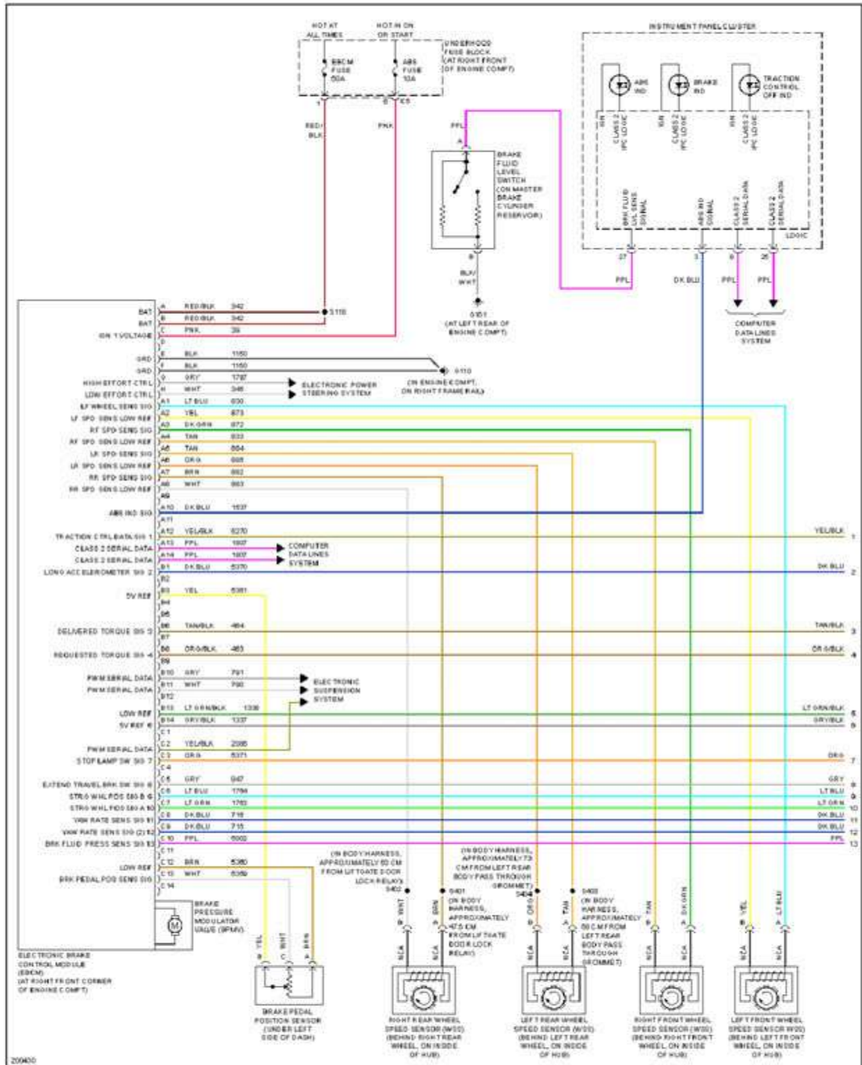
Fig. 6: Anti-lock Brakes Circuit (1 of 2)
