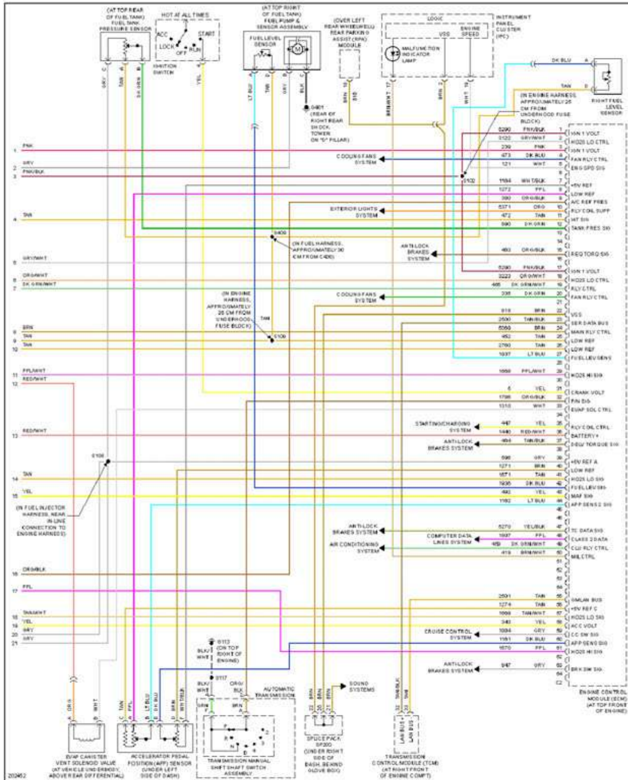
Fig. 22: 3.6L VIN 7, Engine Performance Circuit (4 of 4)
