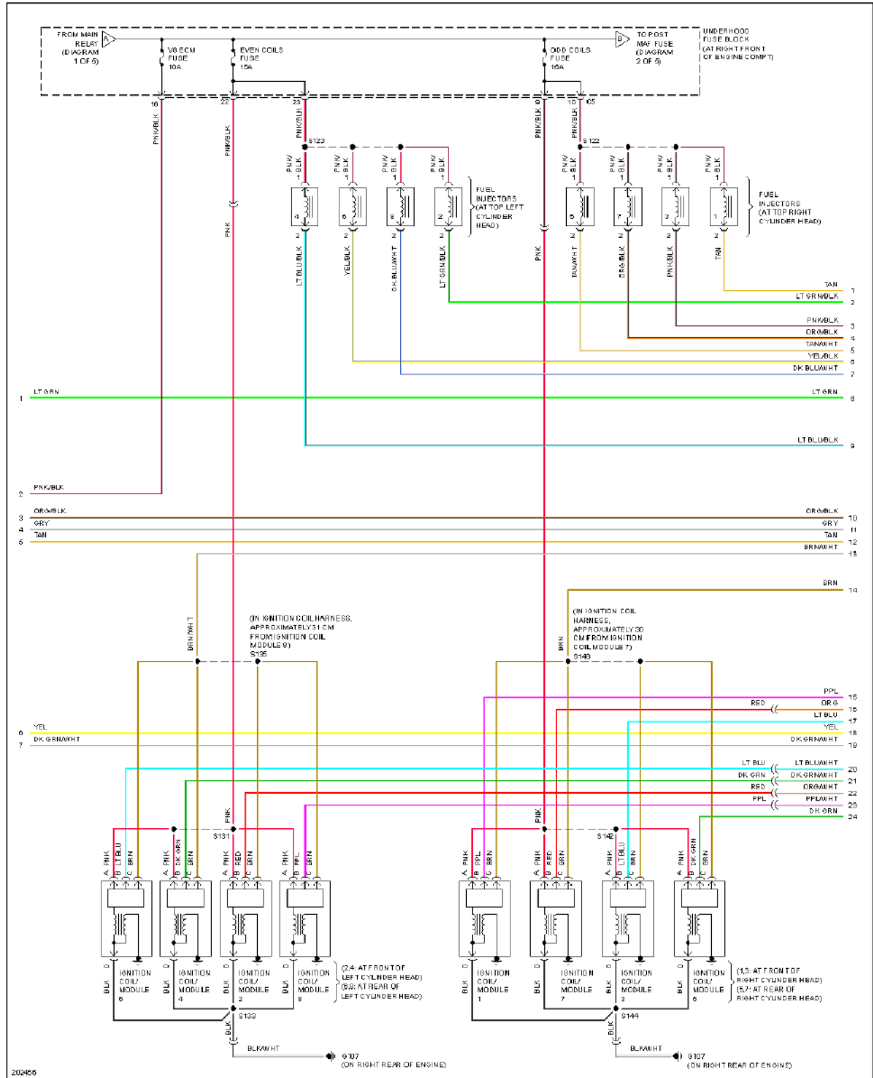
Fig. 26: 4.6L VIN A, Engine Performance Circuit (4 of 5)
