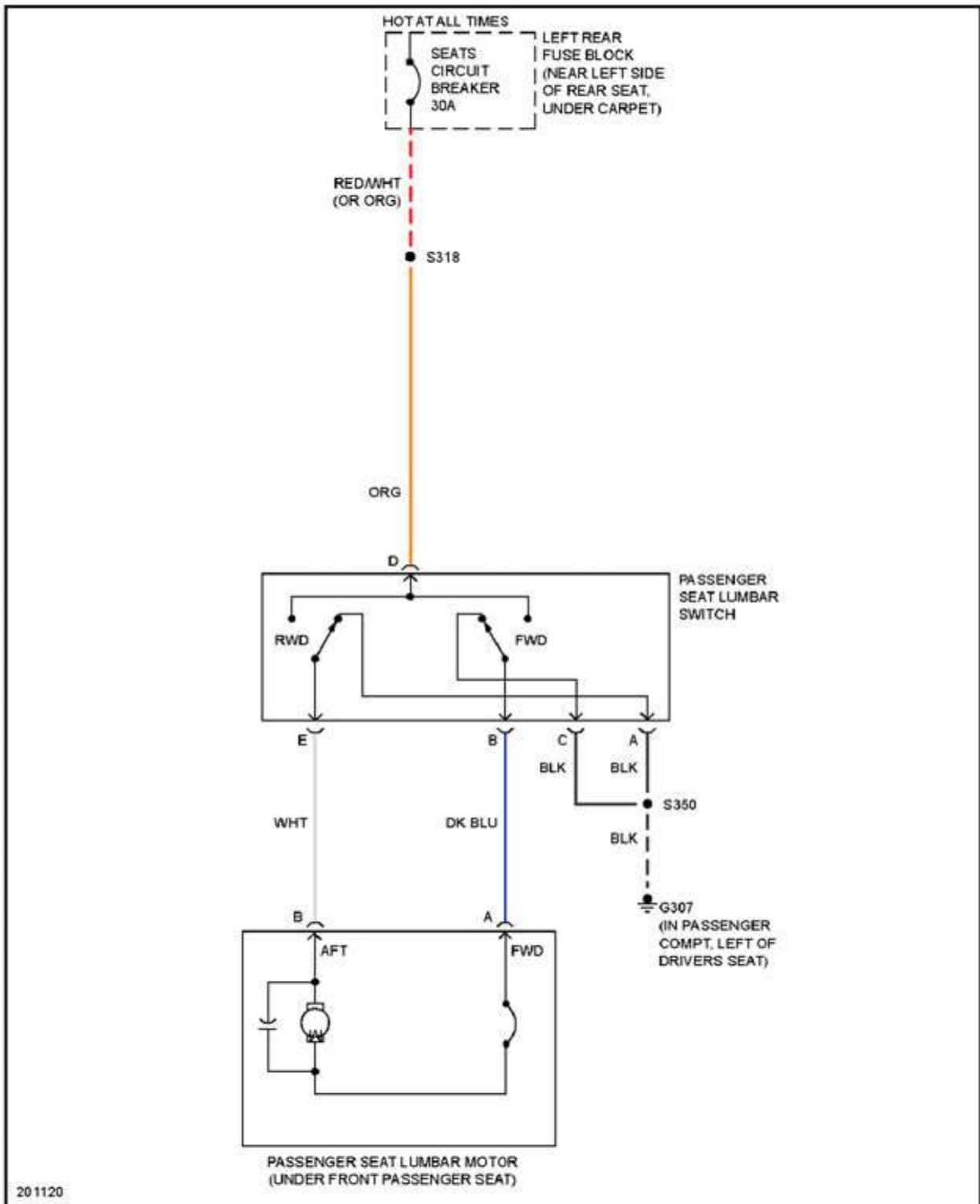
Fig. 64: Passenger's Lumbar Circuit
