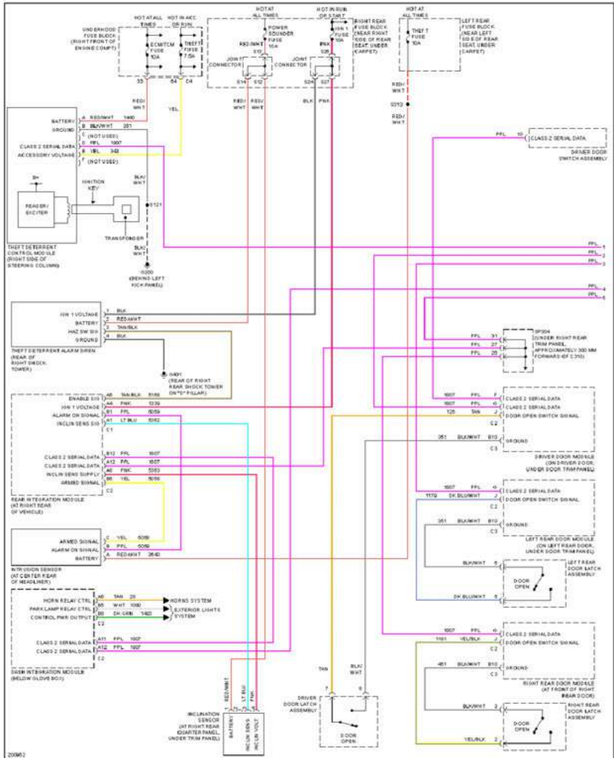
Fig. 8: Anti-theft Circuit (1 of 2)
