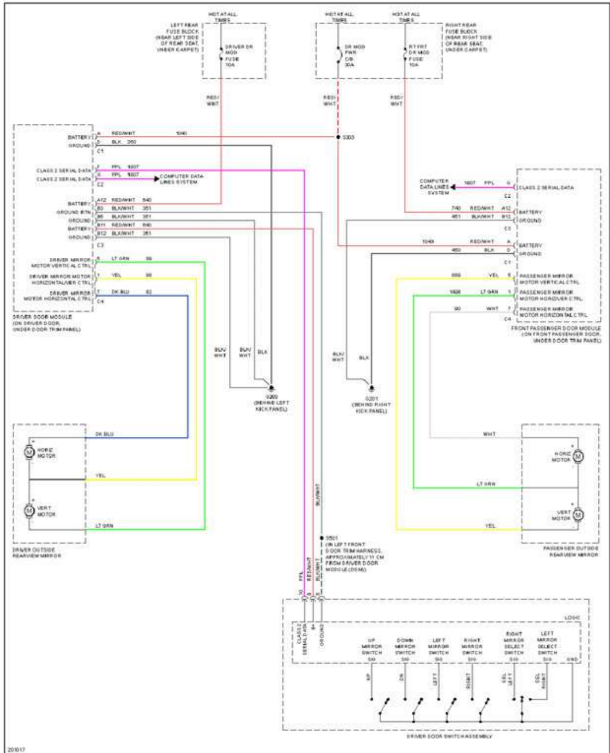
Fig. 61: Power Mirrors Circuit
