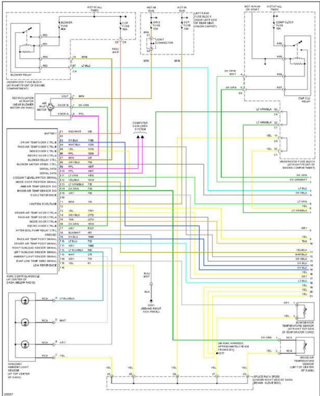
Fig. 1: Automatic A/C Circuit, Front A/C (1 of 3)
