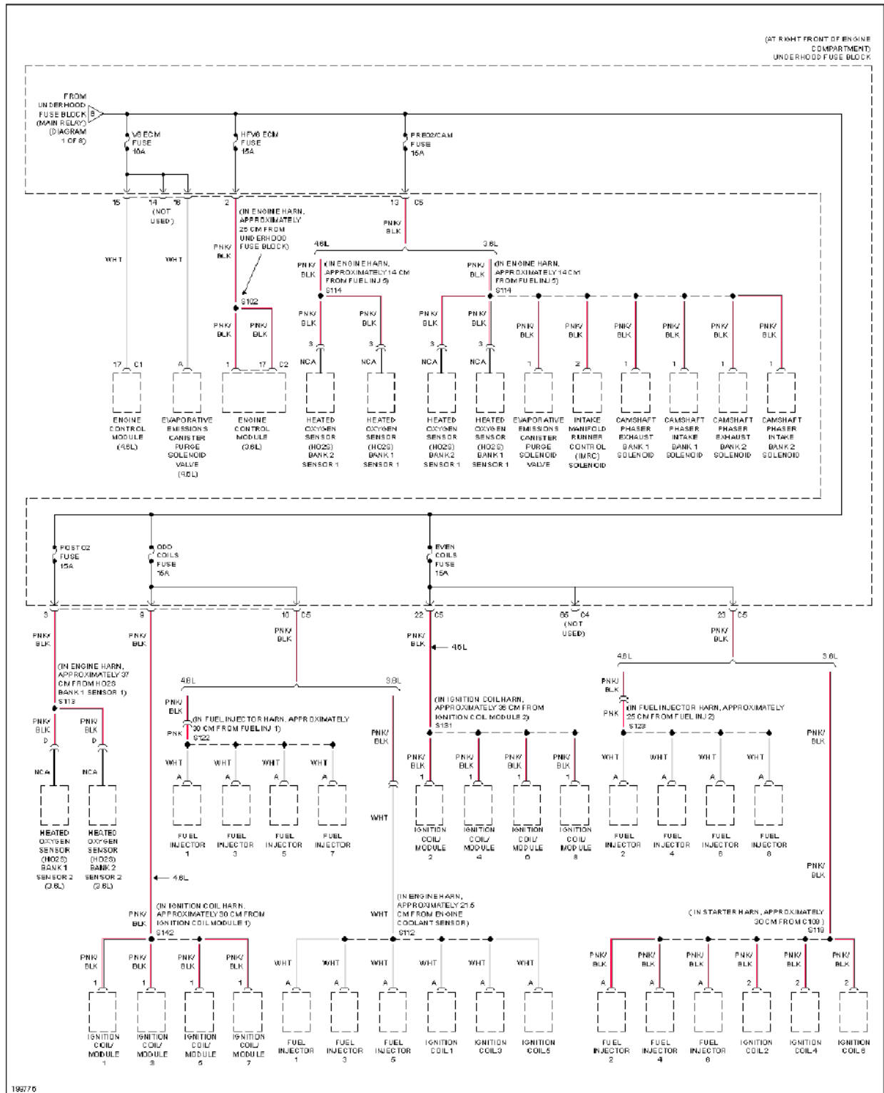
Fig. 51: Power Distribution Circuit (2 of 8)
