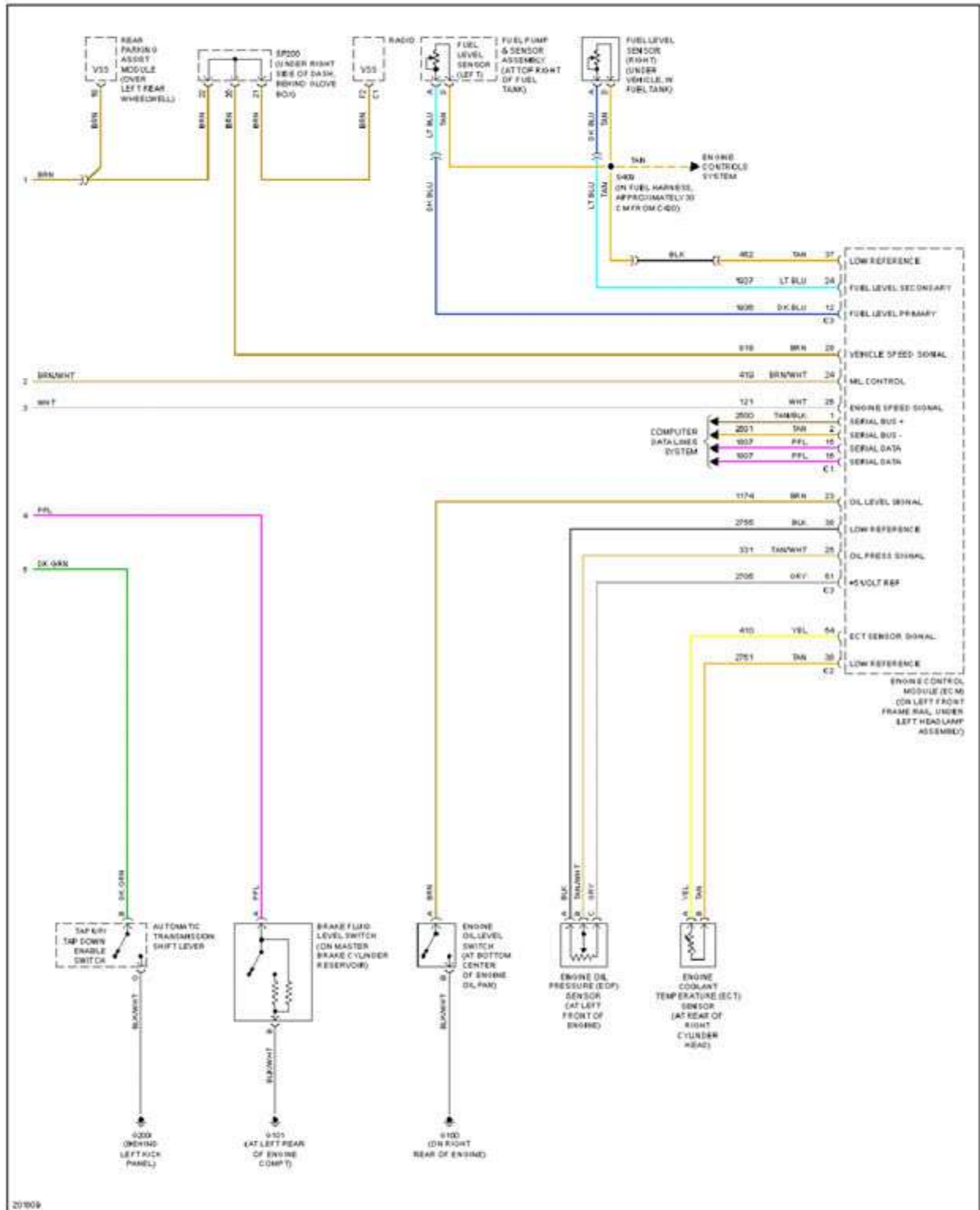
Fig. 40: 4.6L VIN A, Instrument Cluster Circuit (2 of 2)
