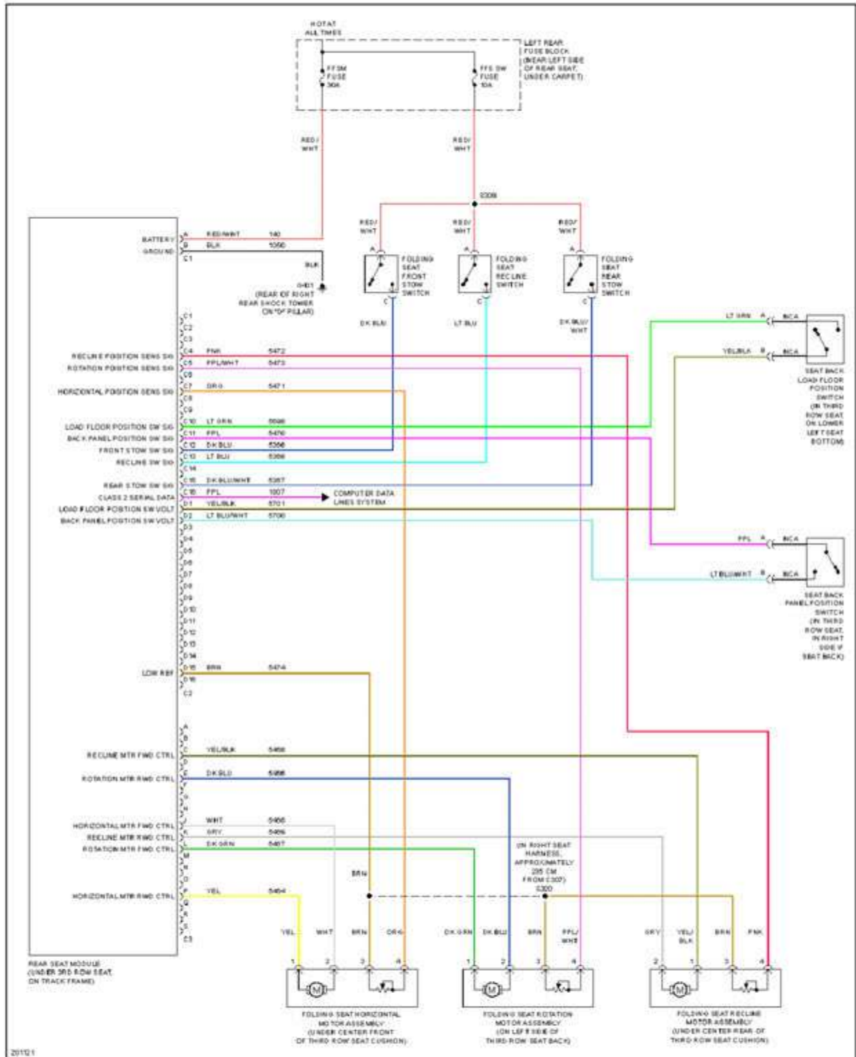
Fig. 65: Rear Power Seat Circuit
