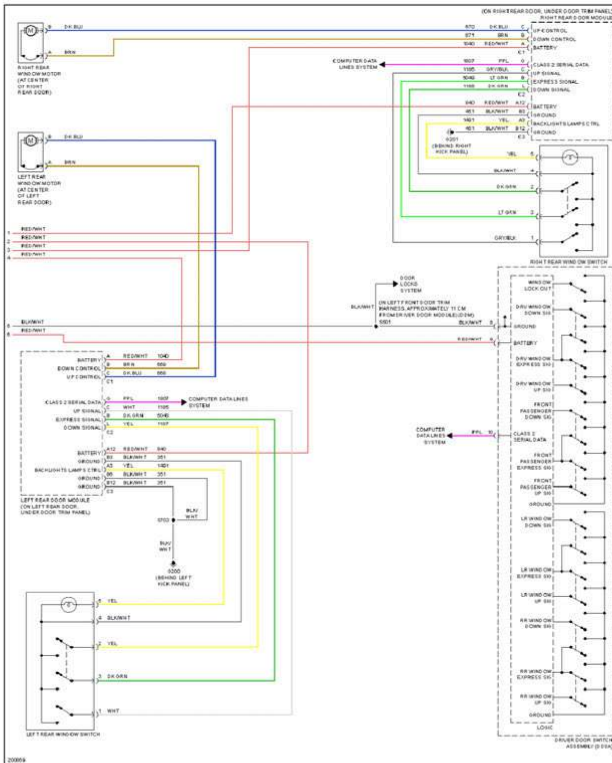
Fig. 68: Power Windows Circuit (2 of 2)
