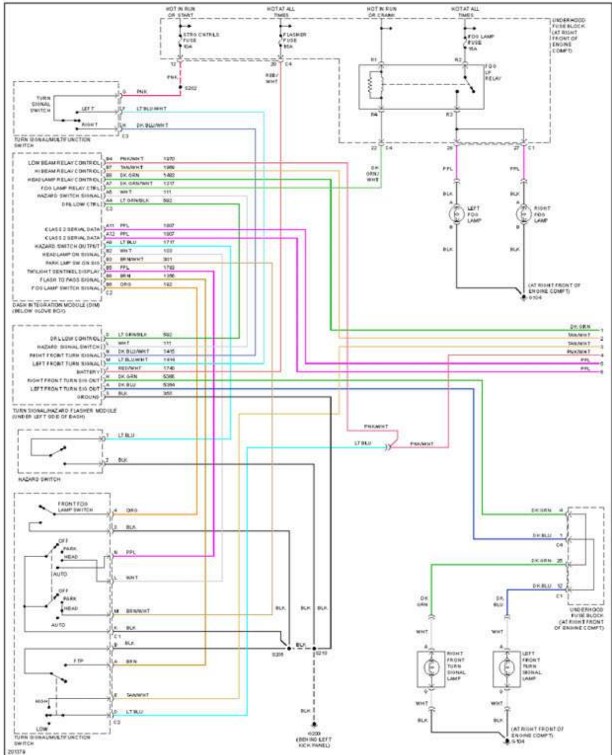
Fig. 34: Headlights Circuit (1 of 2)
