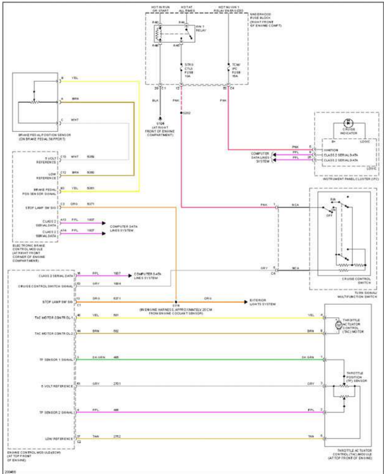
Fig. 15: 4.6L VIN A, Cruise Control Circuit
