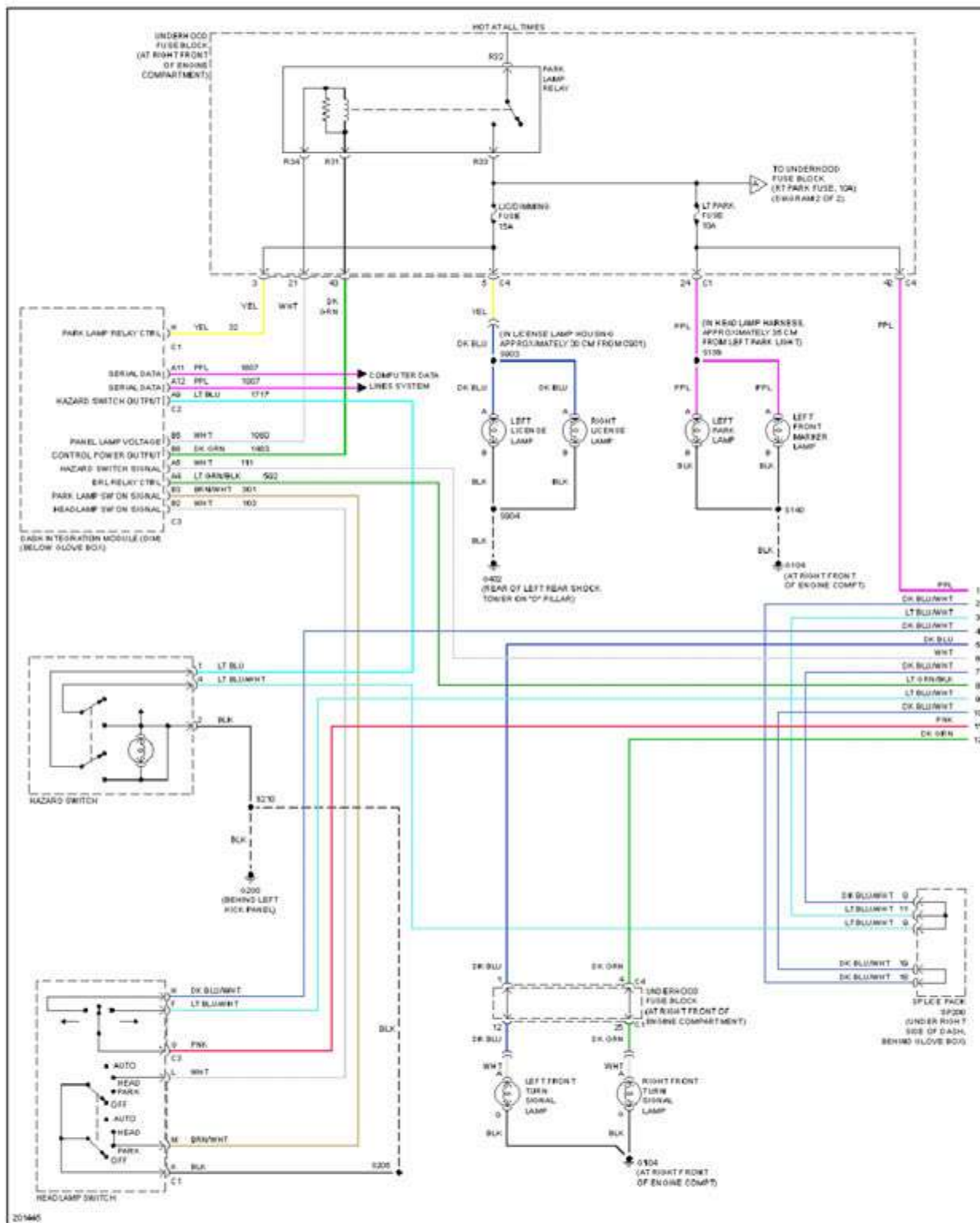
Fig. 29: Exterior Lamps Circuit (1 of 2)
