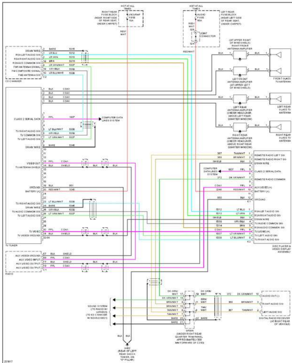
Fig. 75: TV Disc Player and Video Display Circuit
