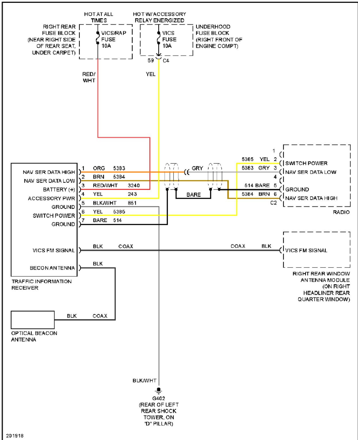
Fig. 76: Traffic Information Receiver Circuit
