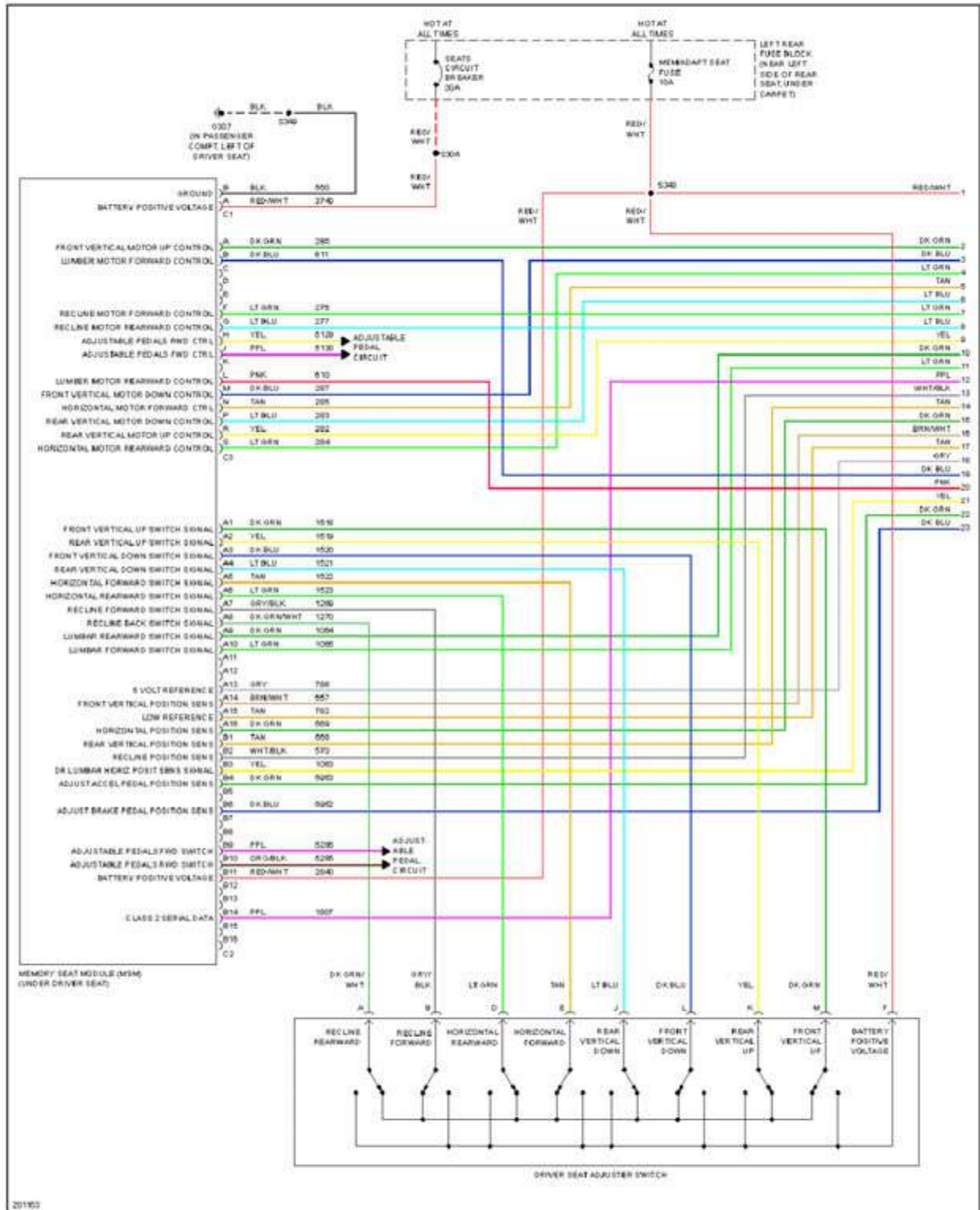
Fig. 46: Memory Seat Circuit (1 of 2)
