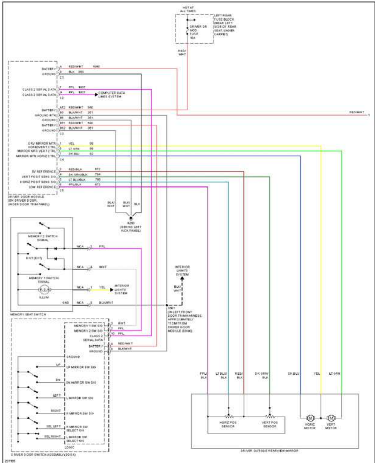
Fig. 44: Memory Mirrors Circuit (1 of 2)
