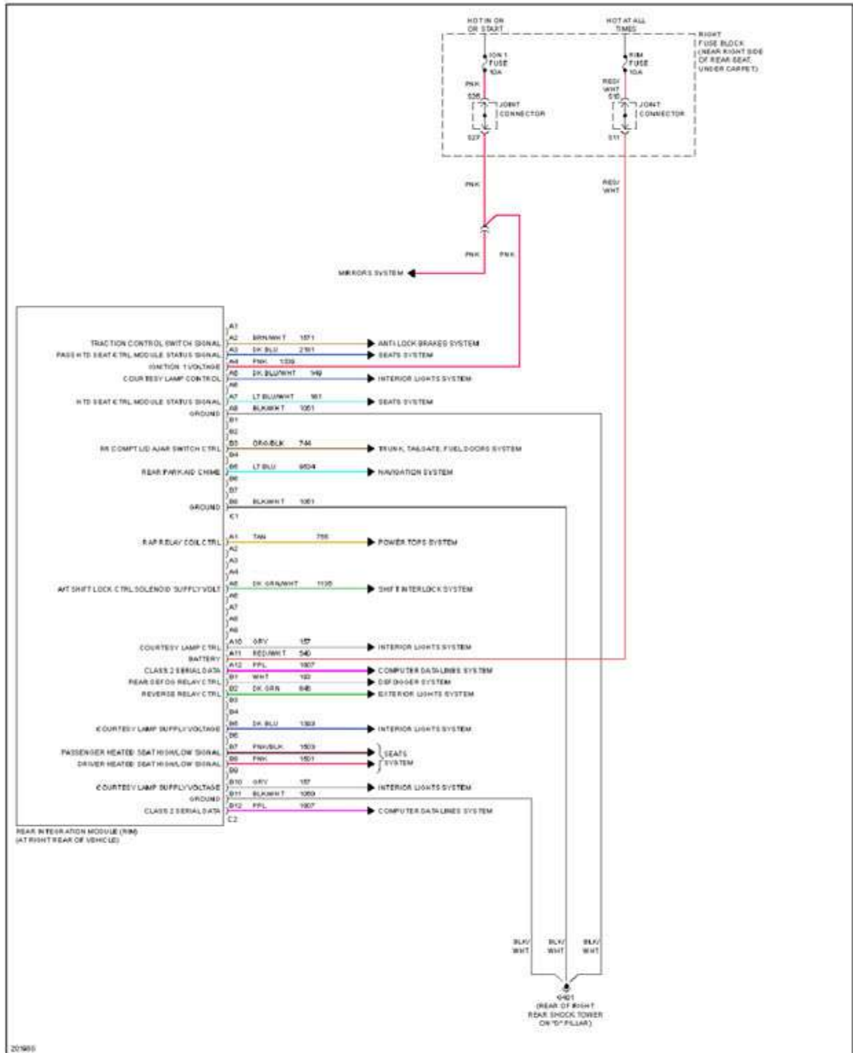
Fig. 11: Rear Integration Module Circuit
