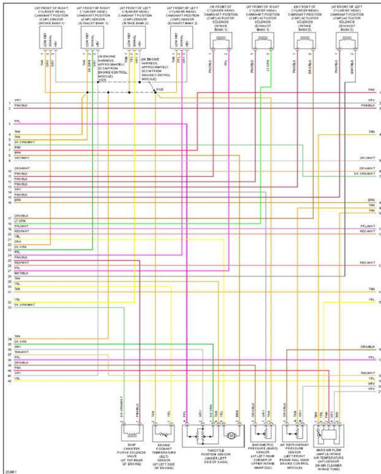
Fig. 21: 3.6L VIN 7, Engine Performance Circuit (3 of 4)
