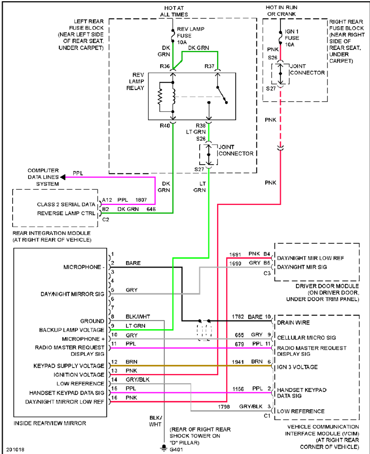
Fig. 60: Automatic Day/Night Mirror Circuit
