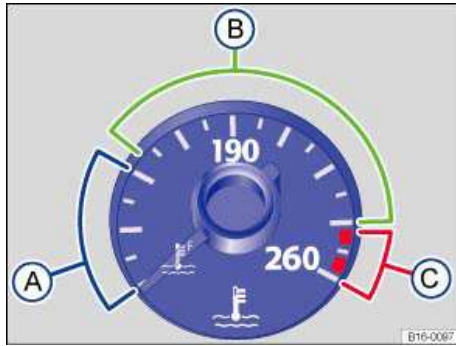
Fig. 162 Engine coolant temperature gauge in the instrument cluster: A Engine cold; B Normal temperature range; C Warning zone.
