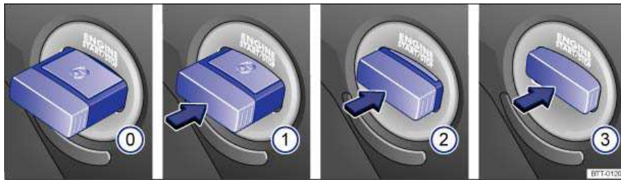
Fig. 128 In the ignition switch: Vehicle key positions.
