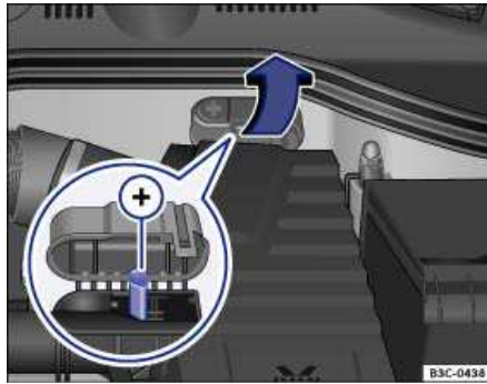
Fig. 205 In the engine compartment: Positive jump start terminal +.
