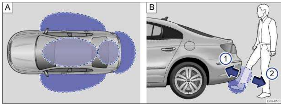
Fig. 23 Ranges of the Keyless Access locking and starting system. A: Outside the vehicle: Unlocking range. Inside the vehicle: Starting range. B: Opening the sensor-controlled luggage compartment lid (Easy Open), if equipped.
