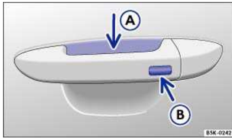
Fig. 24 Keyless Access locking and starting system: Sensor for unlocking A on the inside of the front door handles. Sensor for locking B on the outside of the front door handles.
