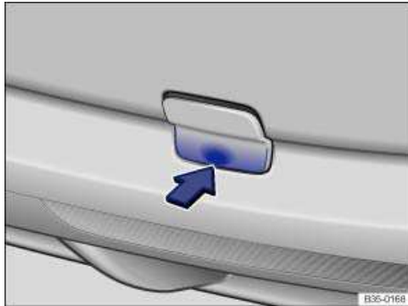
Fig. 209 In the right rear bumper: Removing the cover cap.
