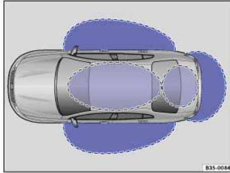
Fig. 25 Ranges of the Keyless Access locking and starting system. Outside the vehicle: Unlocking range. Inside the vehicle: Starting range.
