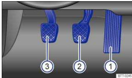
Fig. 131 Pedals in vehicles with manual transmission: 1 Accelerator pedal, 2 Brake pedal, 3 Clutch pedal.
