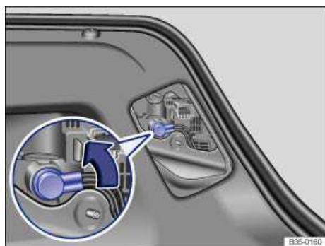
Fig. 202 In the luggage compartment lid: Removing the bulb holder.
