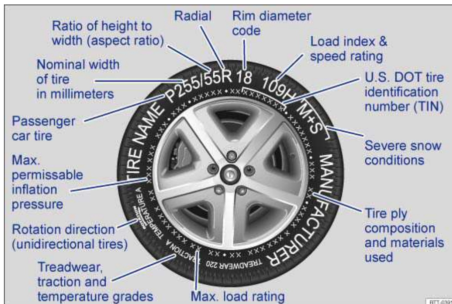
Fig. 111 International tire labeling.
