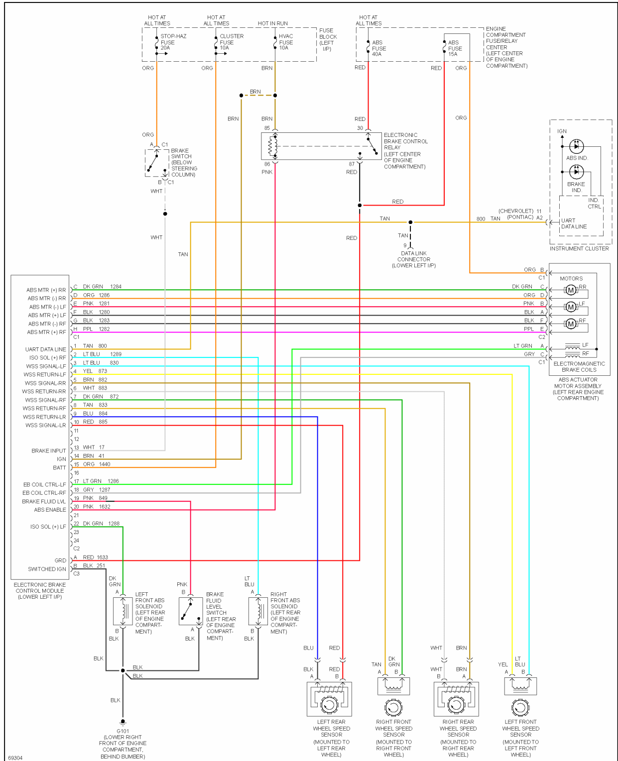
Fig. 4: Anti-lock Brake Circuits, W/O Traction Control
