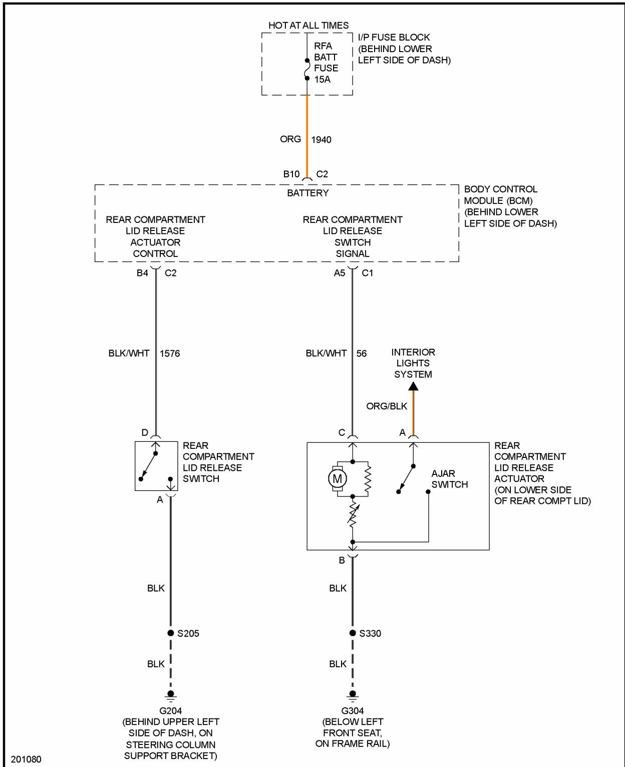
Fig. 40: Trunk Release Circuit
