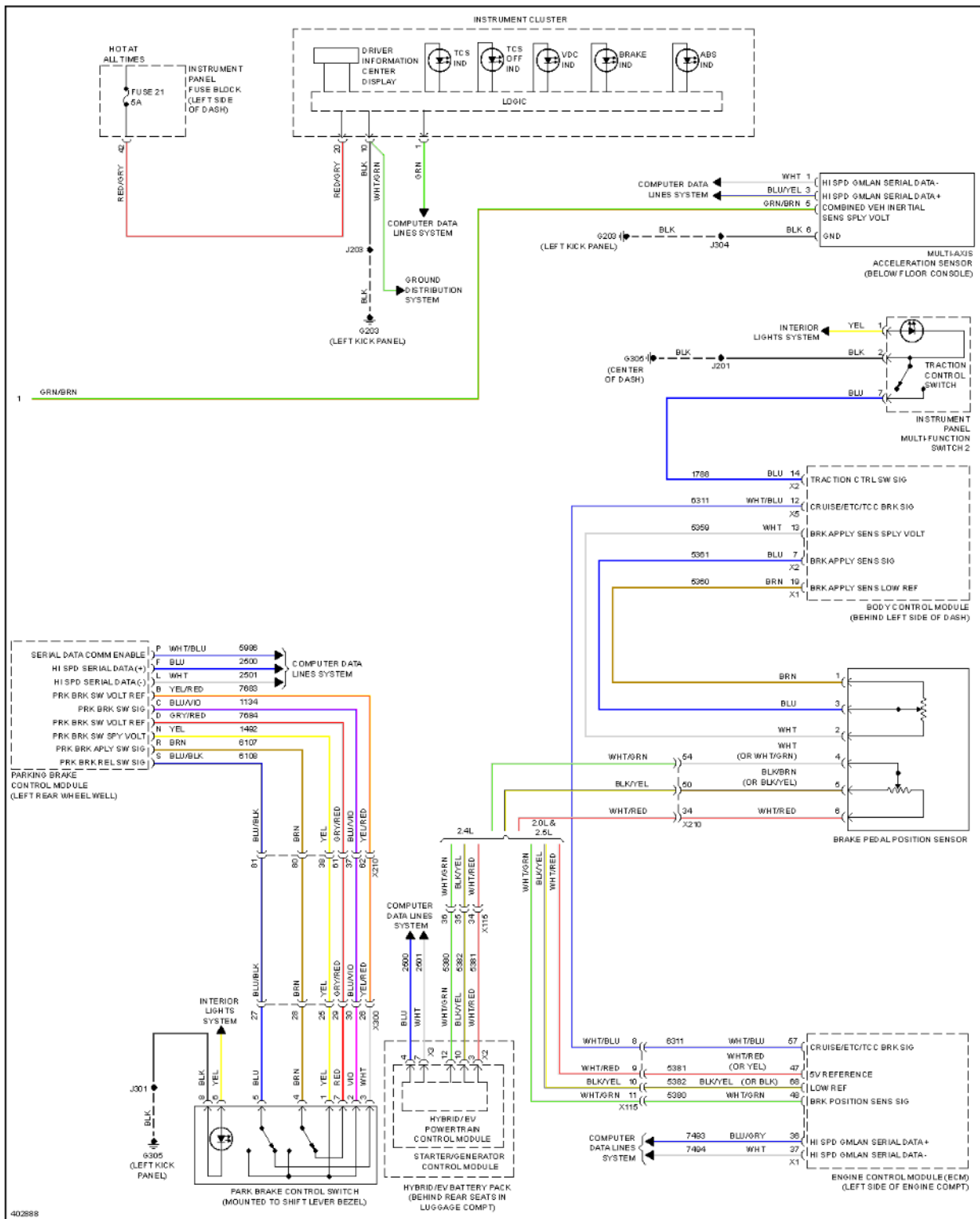
Fig. 10: Anti-lock Brakes Circuit (2 of 2)
