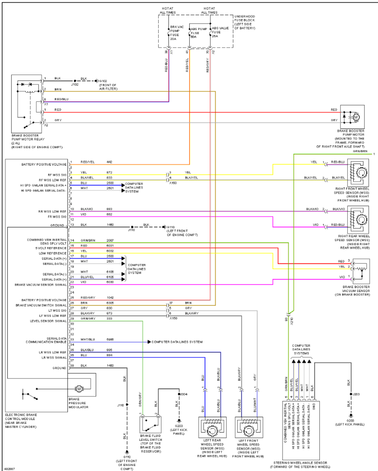
Fig. 9: Anti-lock Brakes Circuit (1 of 2)
