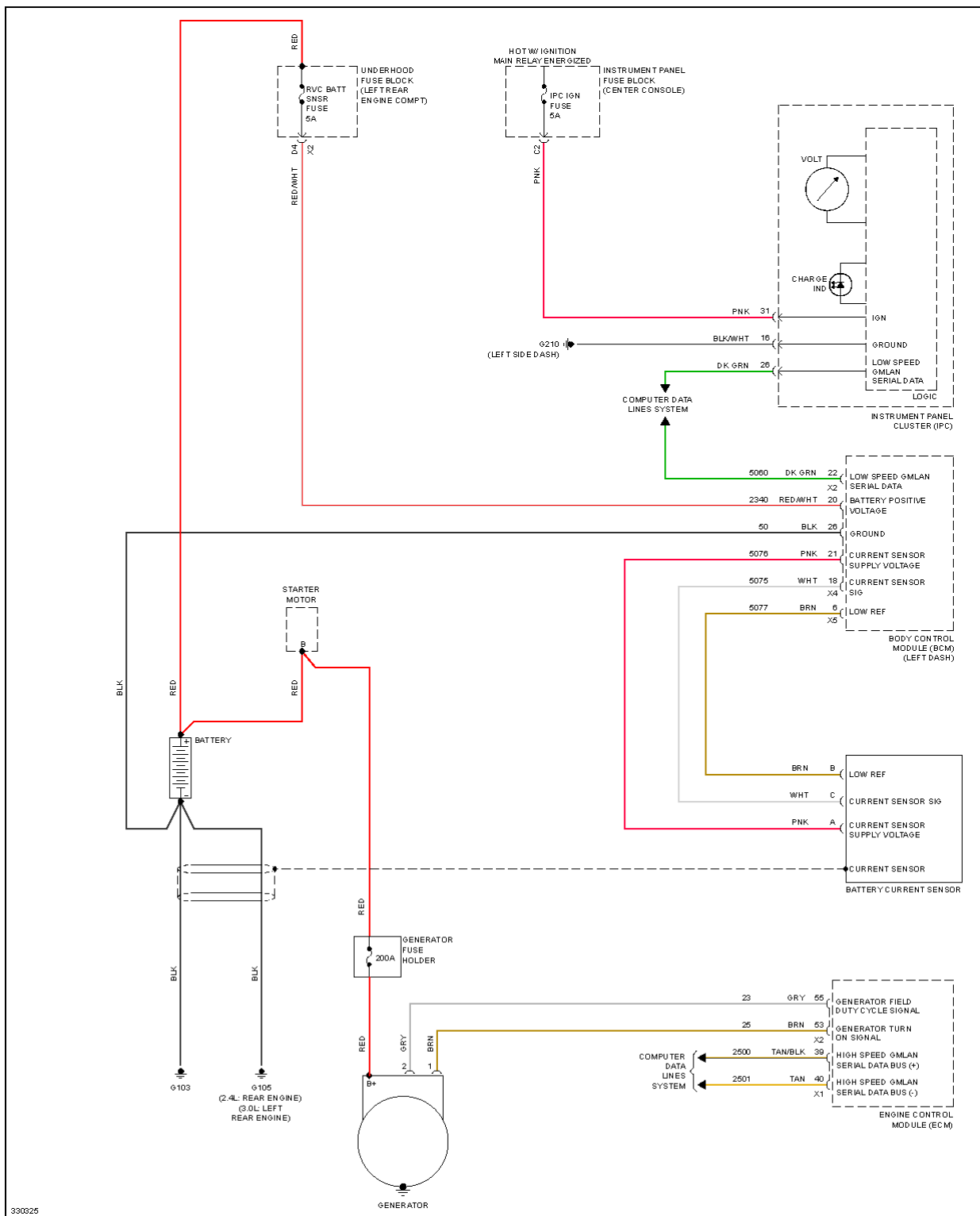
Fig. 71: Charging Circuit
