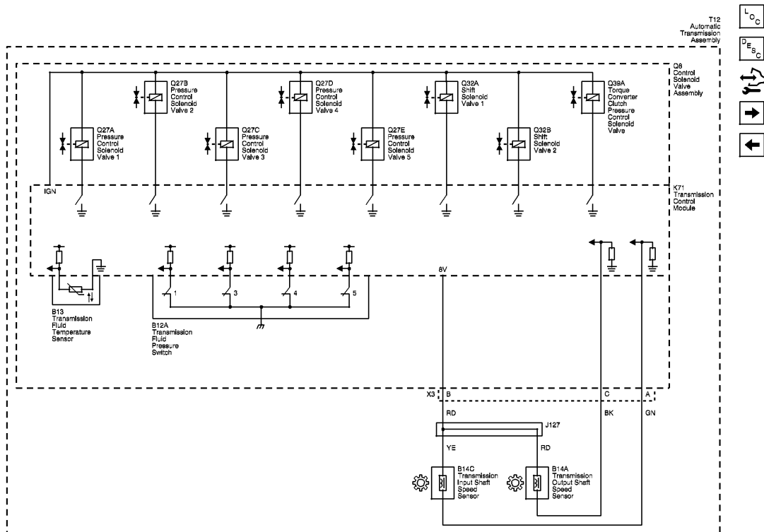
Fig. 2: Speed and Temperature Sensors, Pressure and Shift Controls Wiring Schematic Courtesy of GENERAL MOTORS COMPANY
