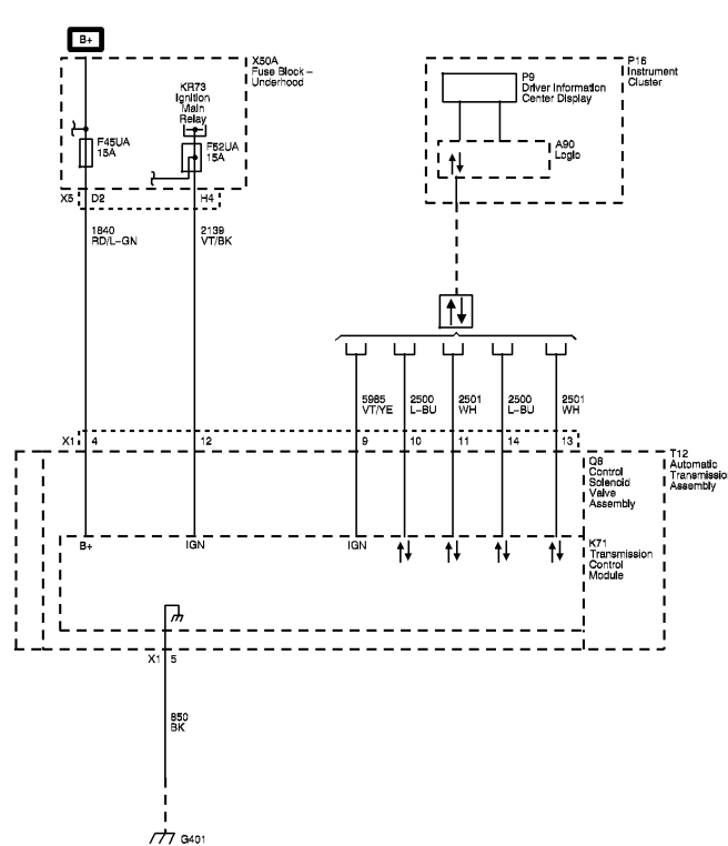
Fig. 1: Power, Ground, Data Communication, and MIL Wiring Schematic Courtesy of GENERAL MOTORS COMPANY
