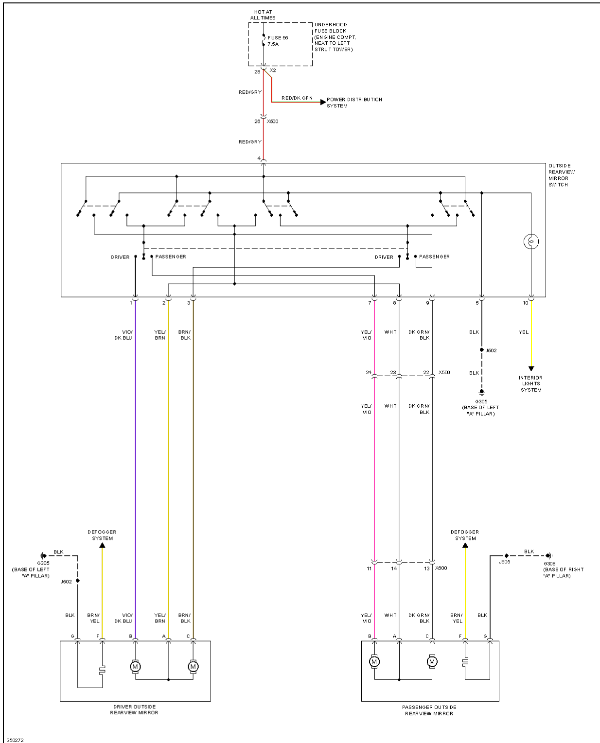
Fig. 54: Power Mirrors Circuit
