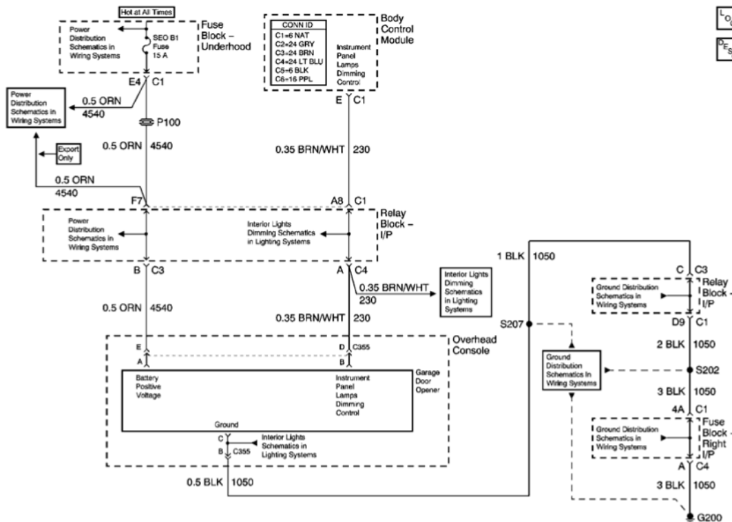
Fig. 1: Garage Door Opener Schematic Courtesy of GENERAL MOTORS CORP.
